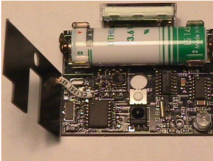
Top View of the Point Six IR Counter Transmitter Circuit Board, Model Point Sensor IR Counter
