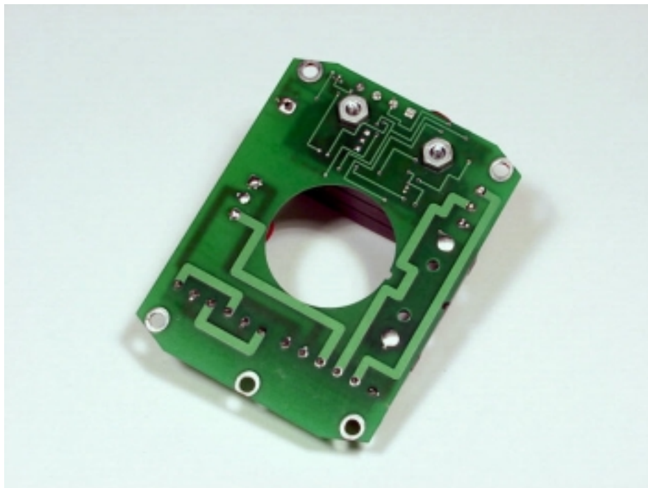
Top and Bottom View of the Point Six Limit Switch Transmitter Circuit Board, Model LSX-1
