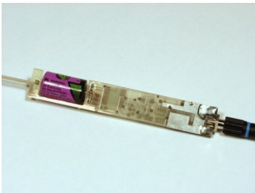
Top and Bottom View of the Point Six Wireless Temperature Probe Transmitter Circuit Board, Model WOW-PRO
