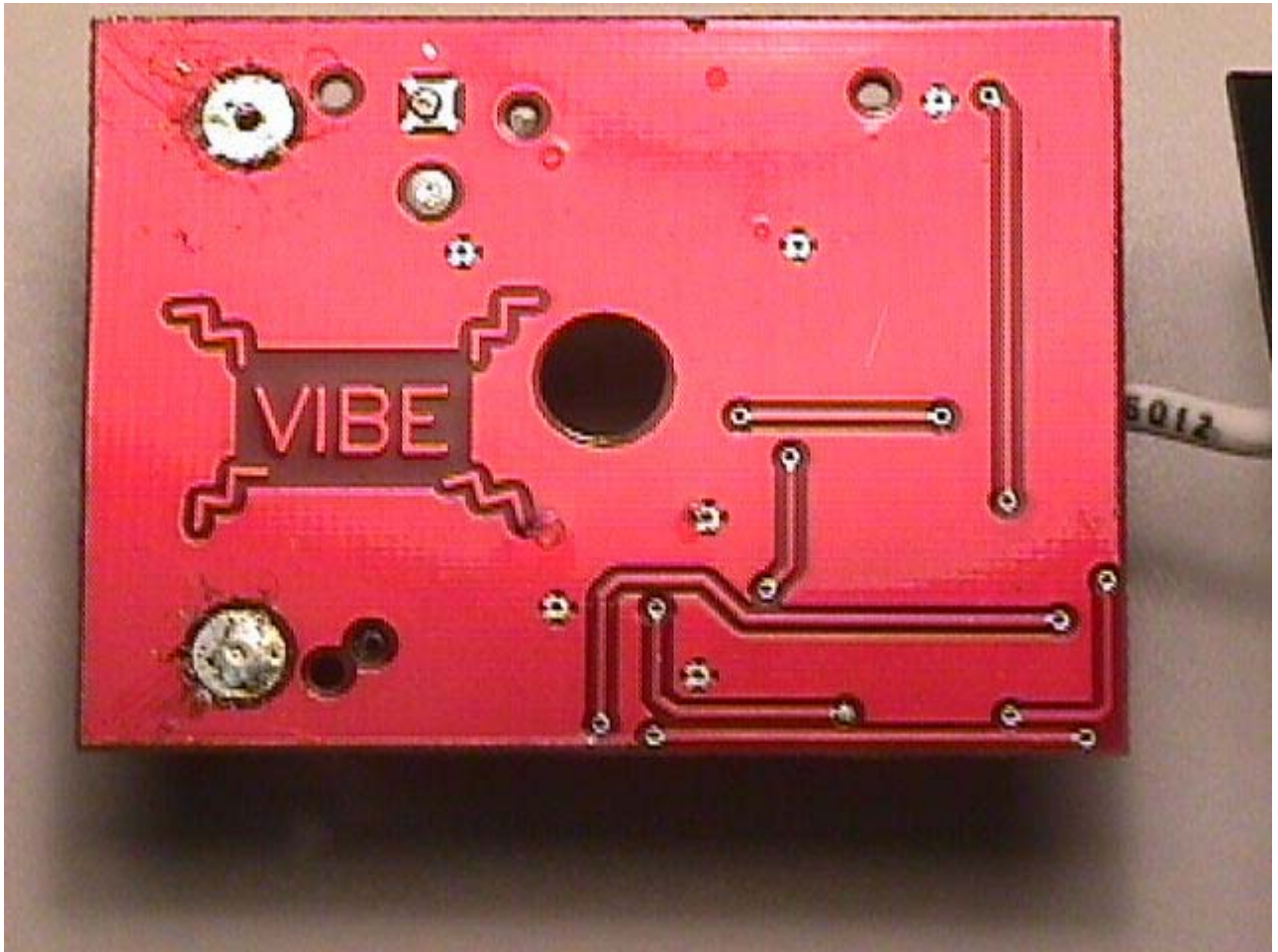
Bottom View of the Point Six Vibration Transmitter Circuit Board, Model Point Sensor Vibration
