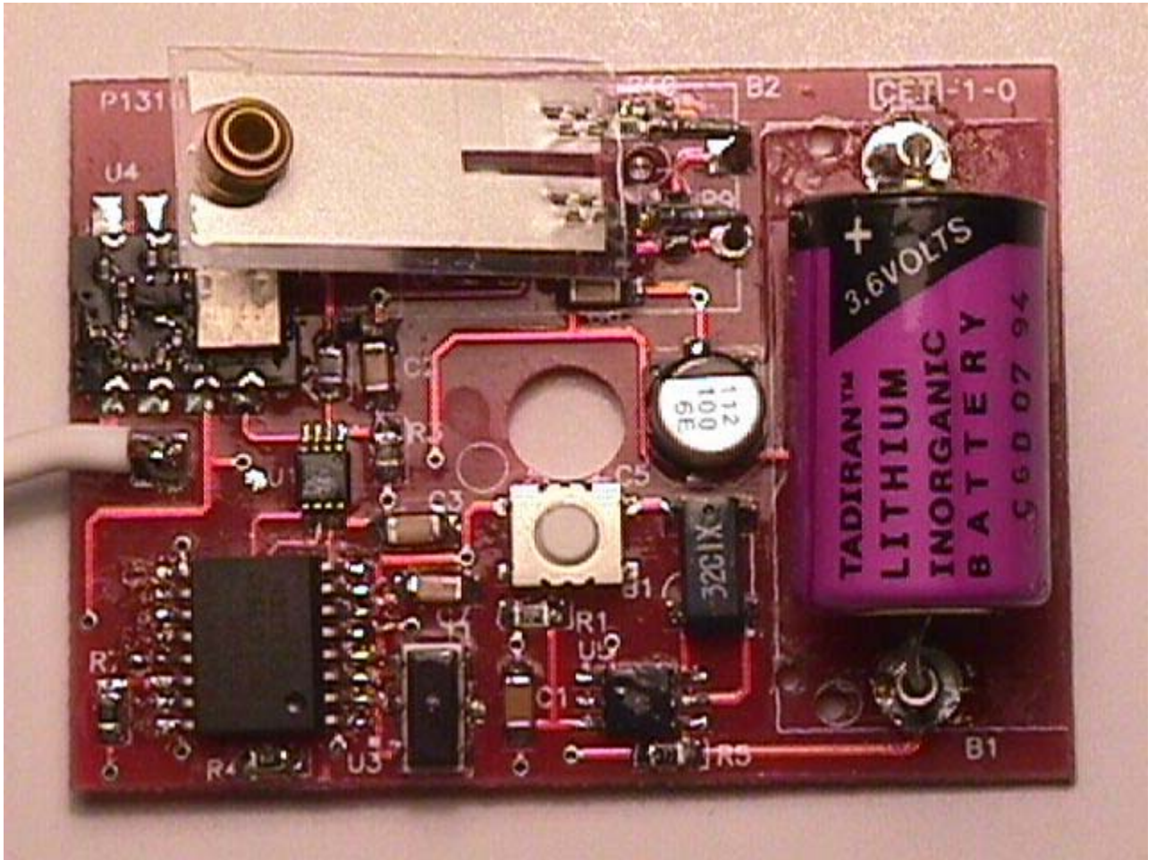
Top View of the Point Six Vibration Transmitter Circuit Board, Model Point Sensor Vibration
