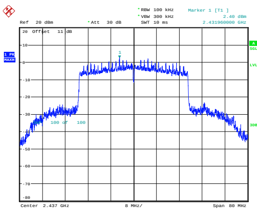
802.11ax40_2437MHz_RU_Full_Chain 1
