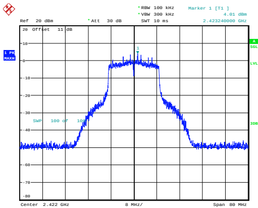
802.11n40_2422MHz_Chain 0
