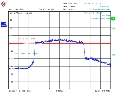
802.11ax40_2422MHz_RU_Full_Chain 0
