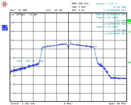
802.11n40_2452MHz_Chain 0
