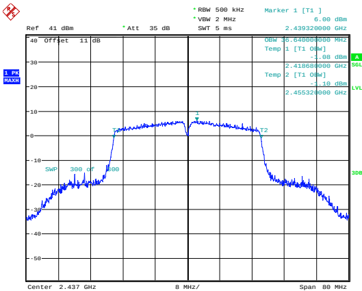
802.11n40_2437MHz_Chain 0
