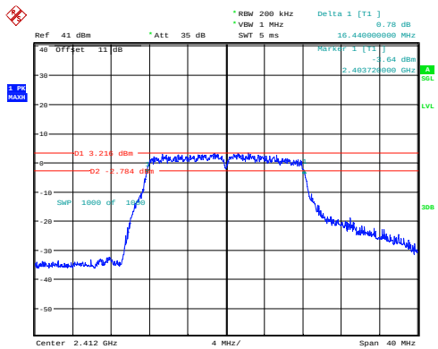
802.11g_2412MHz_Chain 0
