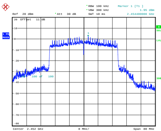
802.11ax40_2452MHz_RU_Full_Chain 1
