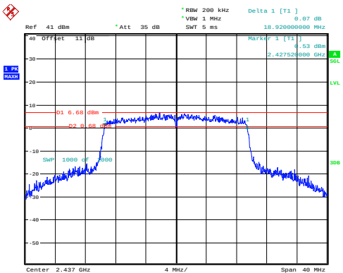
802.11ax20_2437MHz_RU_Full_Chain 0
