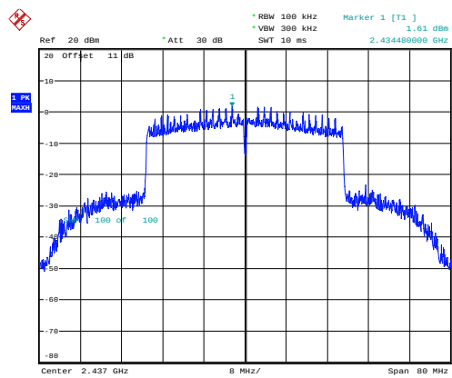
802.11ax40_2437MHz_RU_Full_Chain 0
