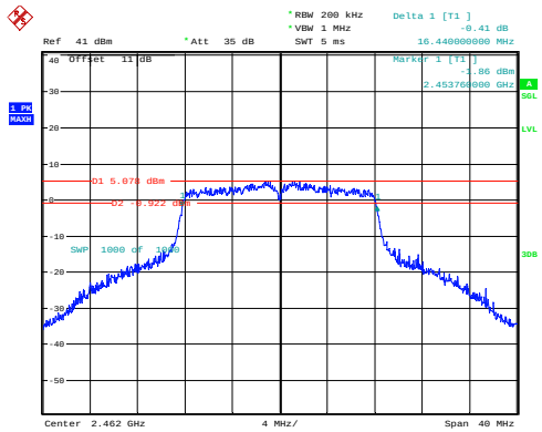
802.11g_2462MHz_Chain 0
