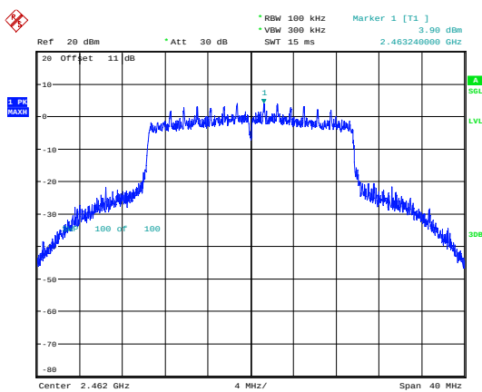
802.11ax20_2462MHz_RU_Full_Chain 0
