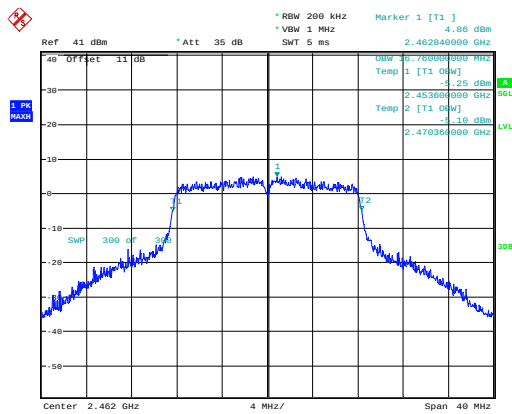
802.11g_2462MHz_Chain 0
