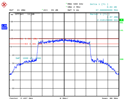
802.11ax40_2437MHz_RU_Full_Chain 0
