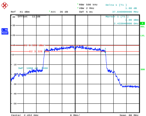
802.11ax40_2452MHz_RU_Full_Chain 0
