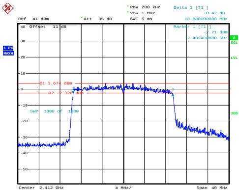
802.11ax20_2412MHz_RU_Full_Chain 0
