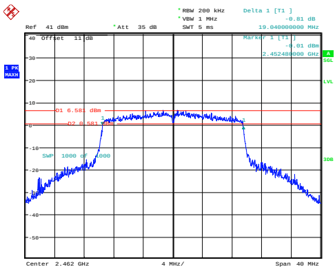
802.11ax20_2462MHz_RU_Full_Chain 0
