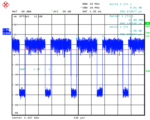
802.11ax20_2437MHz_RU_Full_Chain 0
