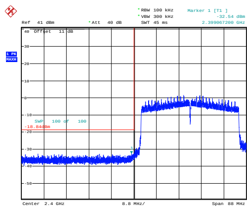
802.11ax40_2422MHz_RU_Full_Chain 0
