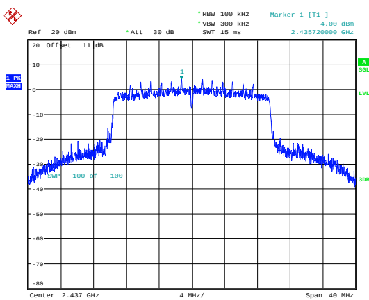
802.11ax20_2437MHz_RU_Full_Chain 0
