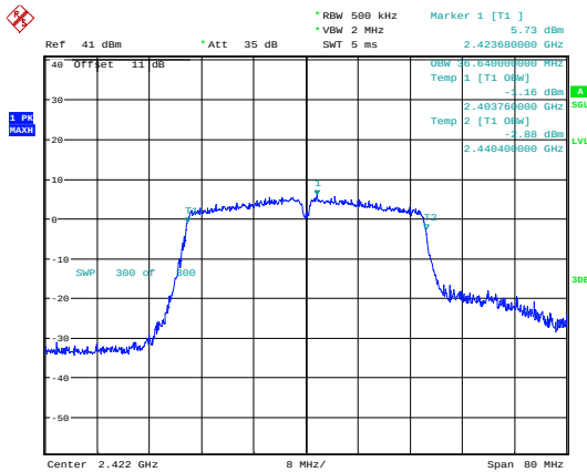
802.11n40_2422MHz_Chain 0
