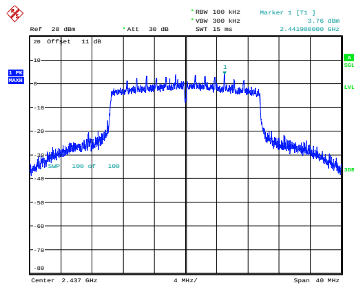
802.11ax20_2437MHz_RU_Full_Chain 1
