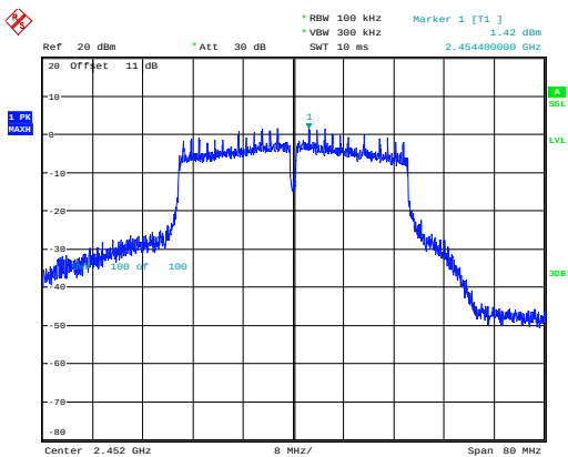
802.11n40_2452MHz_Chain 0
