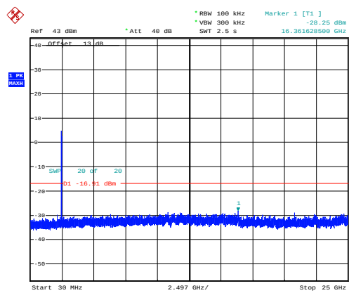
802.11ax20_2462MHz_RU_Full_Chain 1
