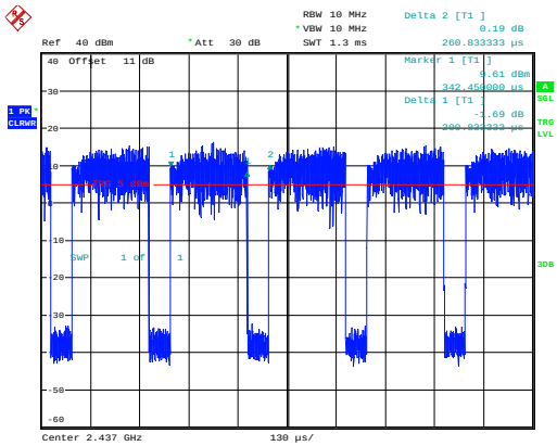
802.11ax40_2437MHz_RU_Full_Chain 0
