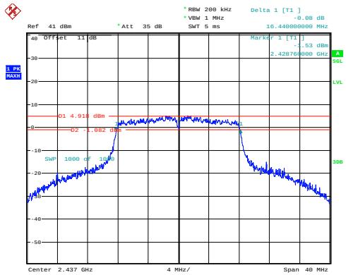
802.11g_2437MHz_Chain 0
