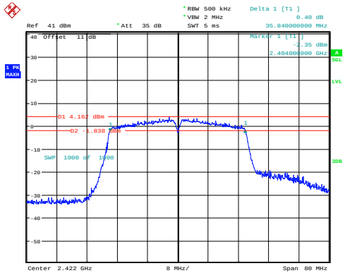
802.11n40_2422MHz_Chain 0
