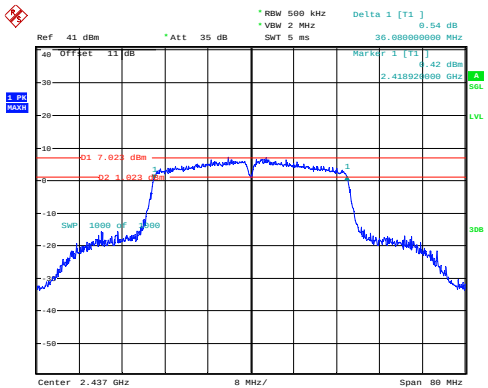
802.11n40_2437MHz_Chain 0
