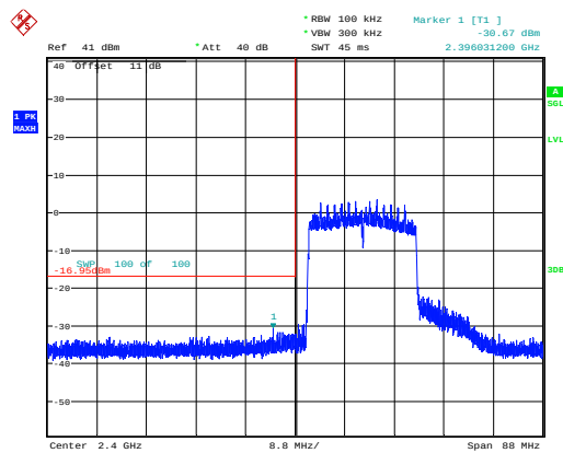
802.11ax20_2412MHz_RU_Full_Chain 1
