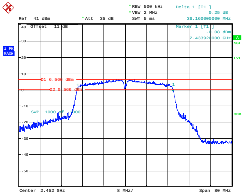
802.11n40_2452MHz_Chain 0
