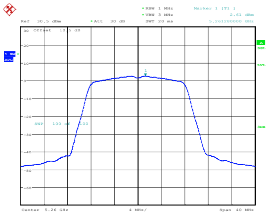
802.11a_5260MHz_Chain 1
