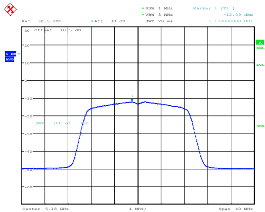
802.11n20_5180MHz_Chain 0
