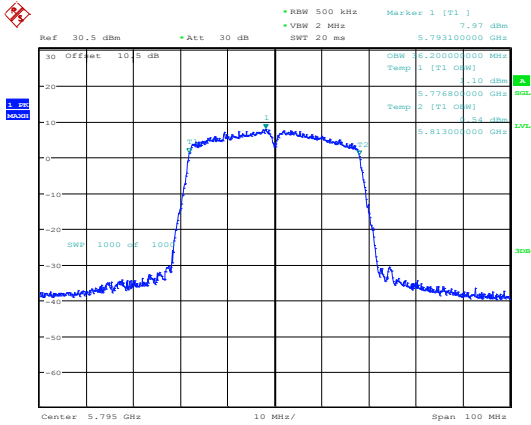
802.11ac40_5795MHz_Chain 0
