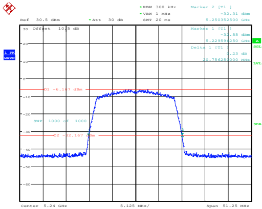
802.11n20_5240MHz_Chain 0
