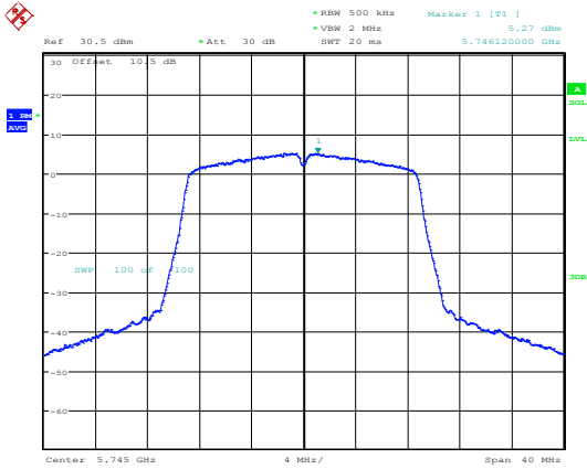
802.11n20_5745MHz_Chain 1
