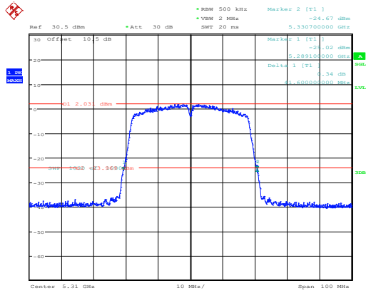
802.11ac40_5310MHz_Chain 0
