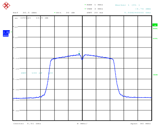
802.11ac40_5510MHz_Chain 0
