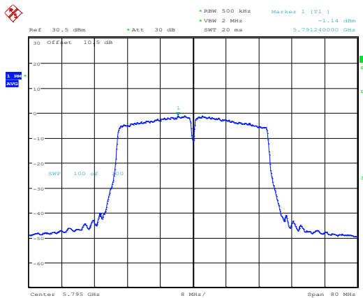
802.11ac40_5795MHz_Chain 0
