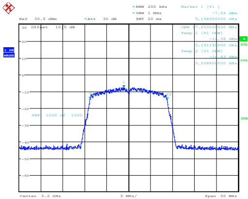
802.11n20_5200MHz_Chain 0
