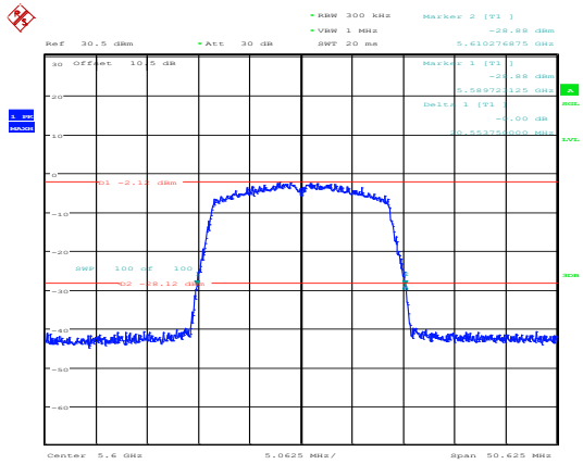
802.11n20_5600MHz_Chain 0
