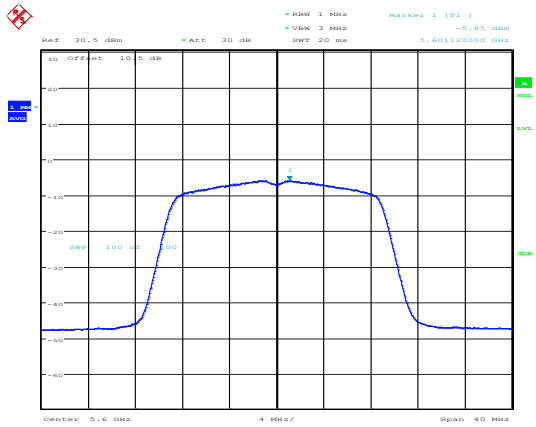
802.11n20_5600MHz_Chain 1
