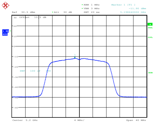
802.11n20_5200MHz_Chain 0
