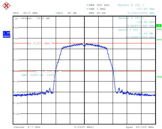
802.11a_5700MHz_Chain 0
