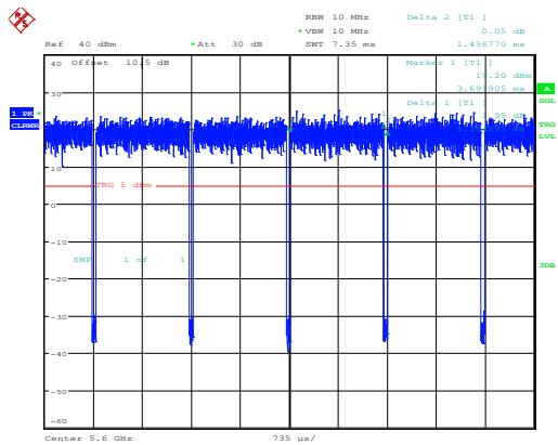
5470-5725MHz 802.11a_5600MHz_Chain 0
