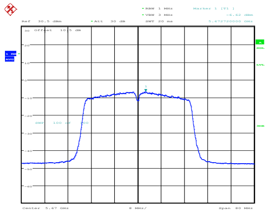
802.11ac40_5670MHz_Chain 0
