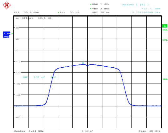
802.11n20_5240MHz_Chain 0
