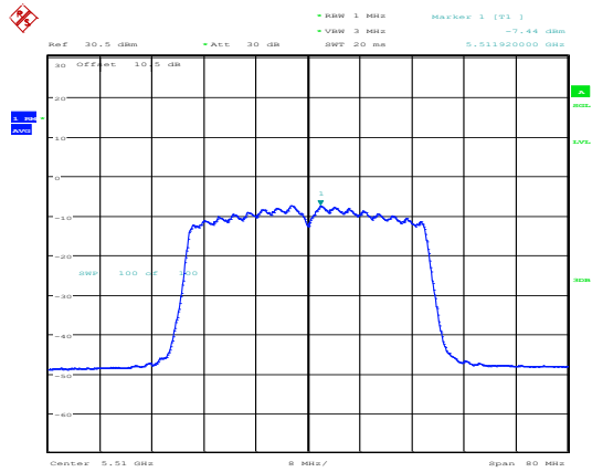
802.11ac40_5510MHz_Chain 1
