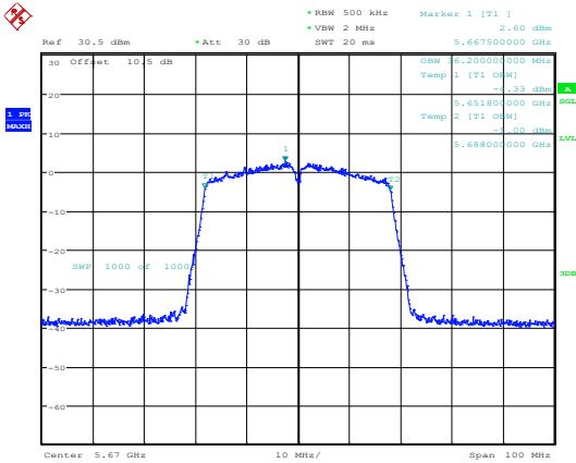
802.11ac40_5670MHz_Chain 0
