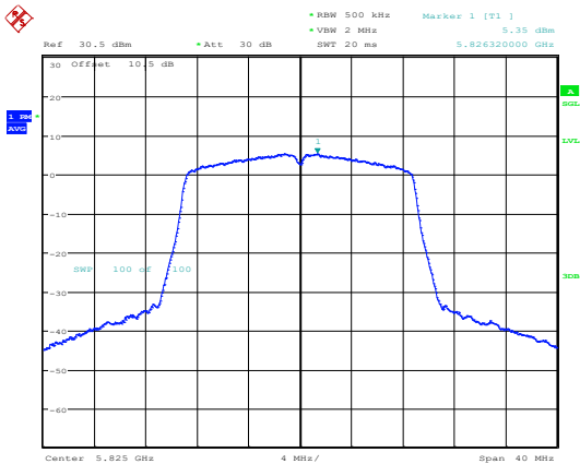
802.11n20_5825MHz_Chain 1
