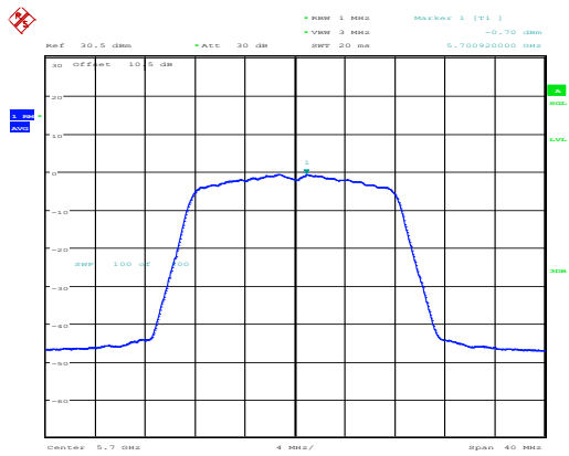
802.11a_5700MHz_Chain 0
