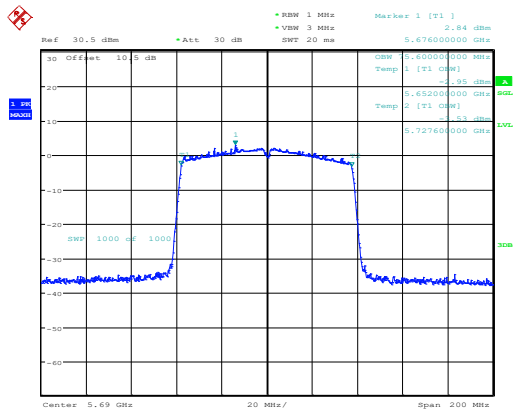
802.11ac80_5690MHz_Chain 0
