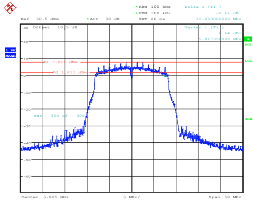
802.11a_5825MHz_Chain 0
