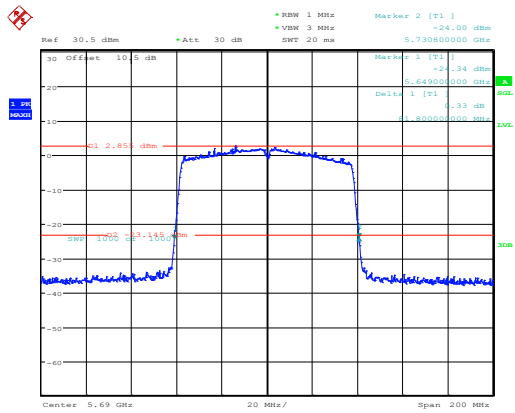
802.11ac80_5690MHz_Chain 0
