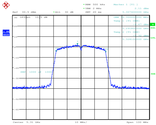
802.11ac40_5310MHz_Chain 0
