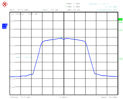
802.11a_5500MHz_Chain 0
