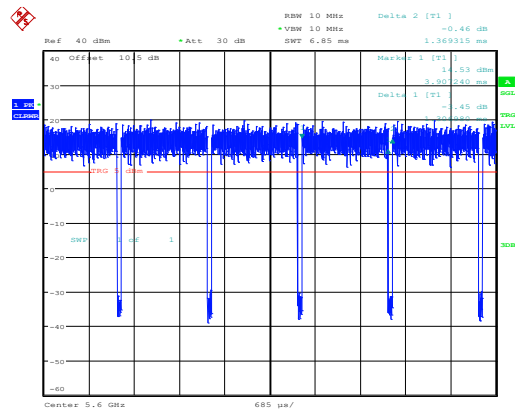
802.11n20_5600MHz_Chain 0
