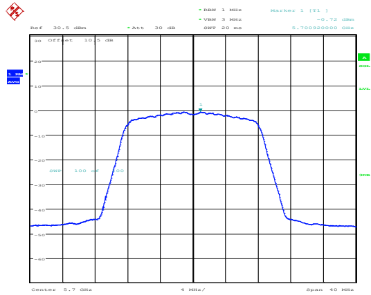
802.11a_5700MHz_Chain 1
