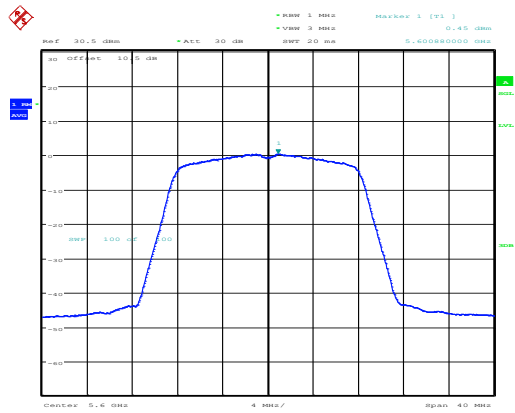
802.11a_5600MHz_Chain 0
