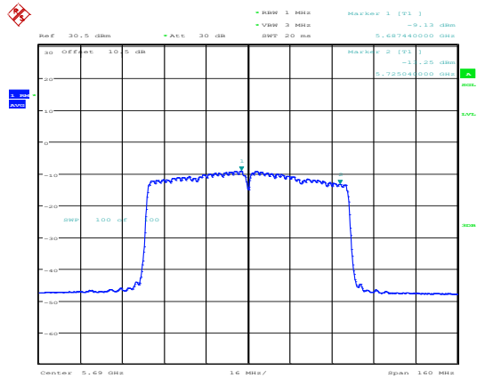
802.11ac80_5690MHz_Chain 0
