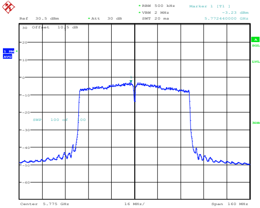
802.11ac80_5775MHz_Chain 1
