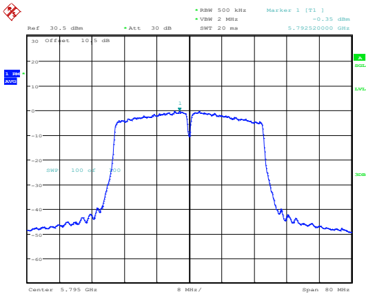
802.11ac40_5795MHz_Chain 1
