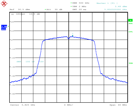
802.11n20_5825MHz_Chain 0
