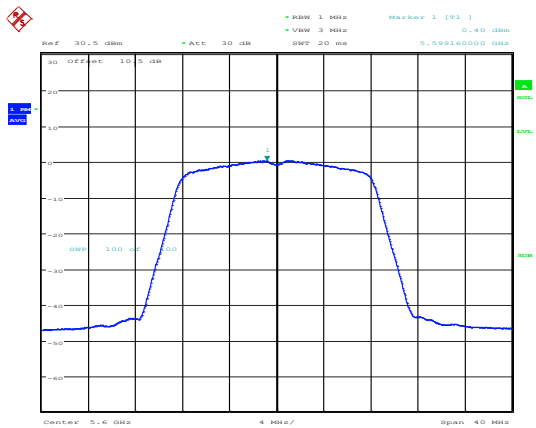
802.11a_5600MHz_Chain 1
