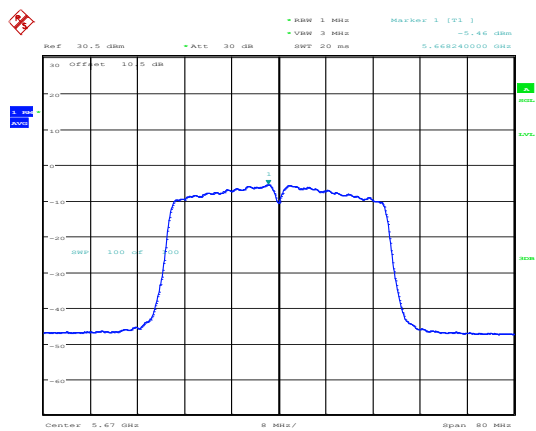
802.11n40_5670MHz_Chain 1
