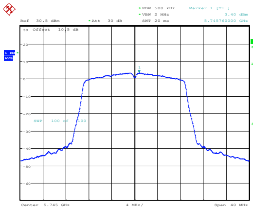
802.11ac20_5745MHz_Chain 1
