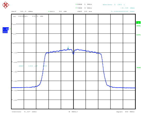
802.11ac40_5670MHz_Chain 1
