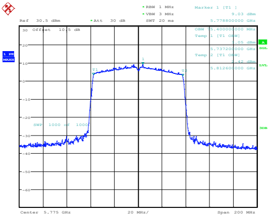
802.11ac80_5775MHz_Chain 0
