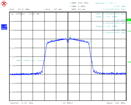
802.11ac40_5510MHz_Chain 0
