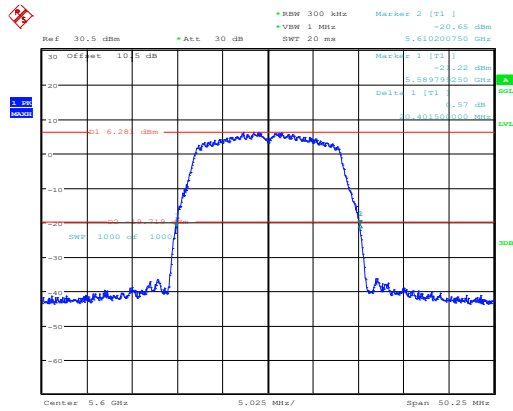
802.11a_5600MHz_Chain 0
