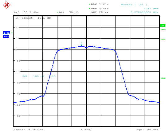
802.11a_5280MHz_Chain 1
