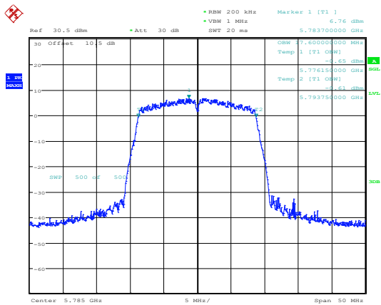
802.11n20_5785MHz_Chain 0
