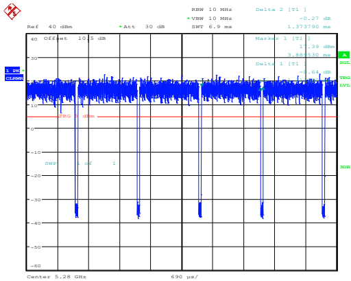
802.11n20_5280MHz_Chain 0
