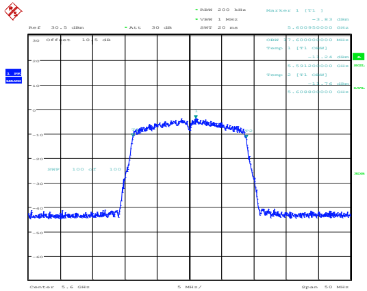
802.11n20_5600MHz_Chain 0
