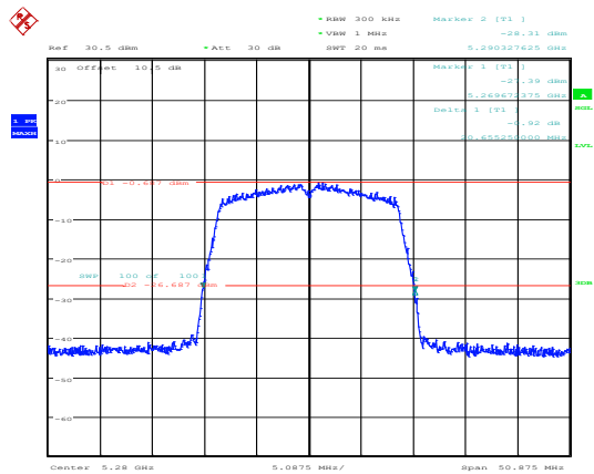
802.11n20_5280MHz_Chain 0
