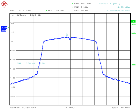
802.11n20_5785MHz_Chain 1
