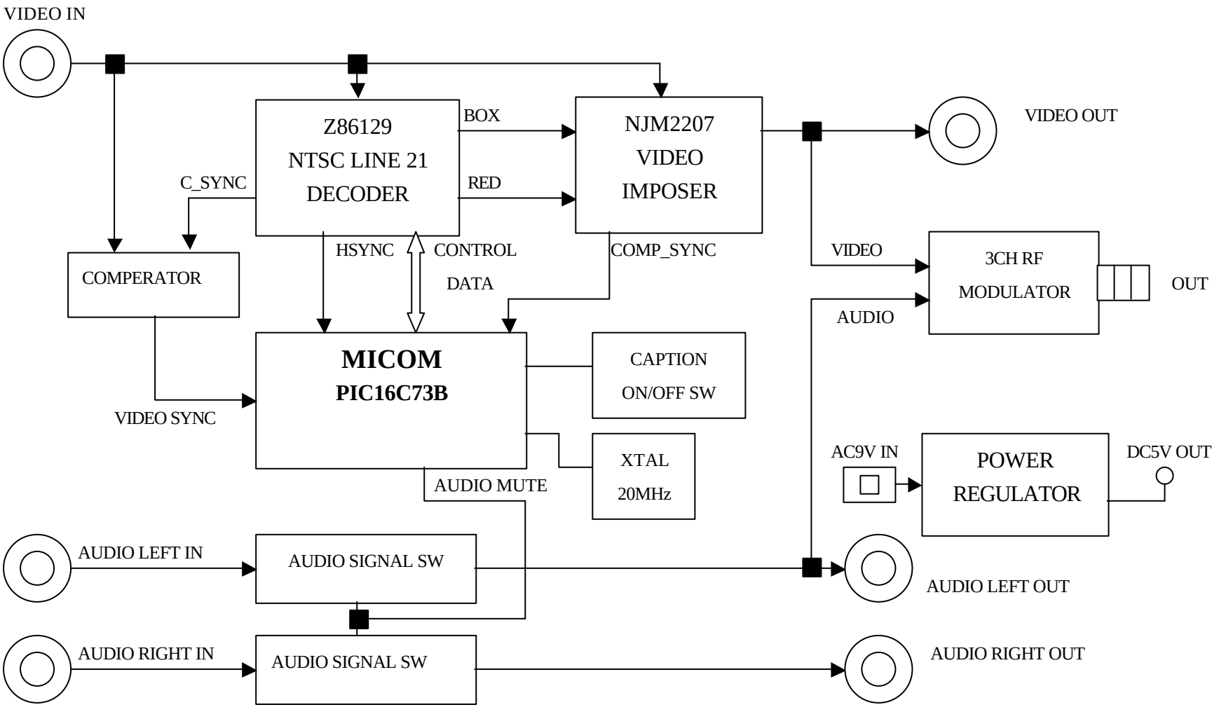
Block Diagram [Protect TV Decoder]
