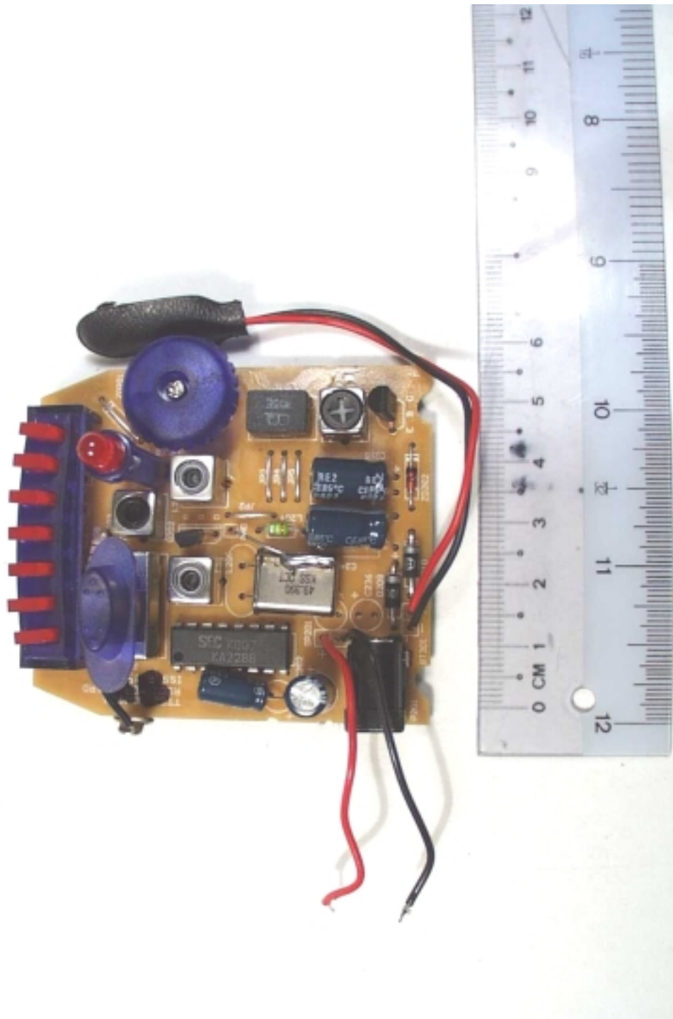
PCB – Component Side
