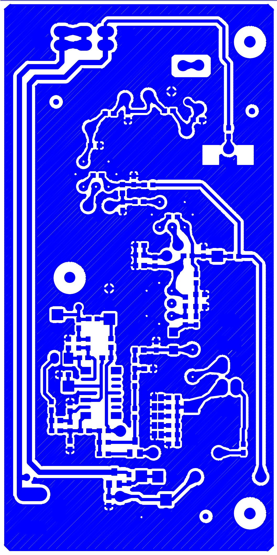
BOTTOM COPPER SIDE
