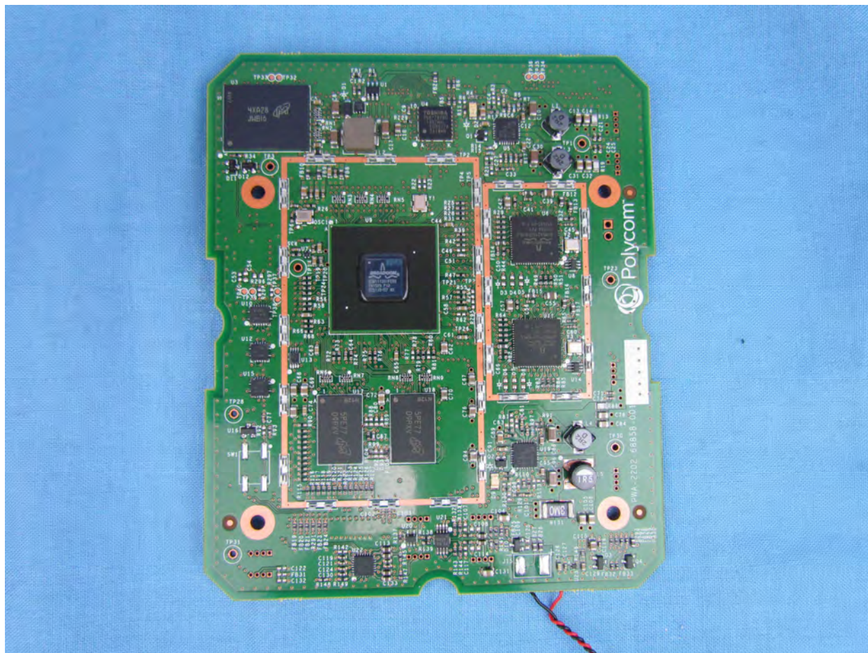
Right Arm PCB Bottom without Shields
