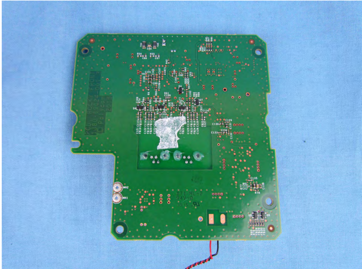
Front Arm PCB Bottom
