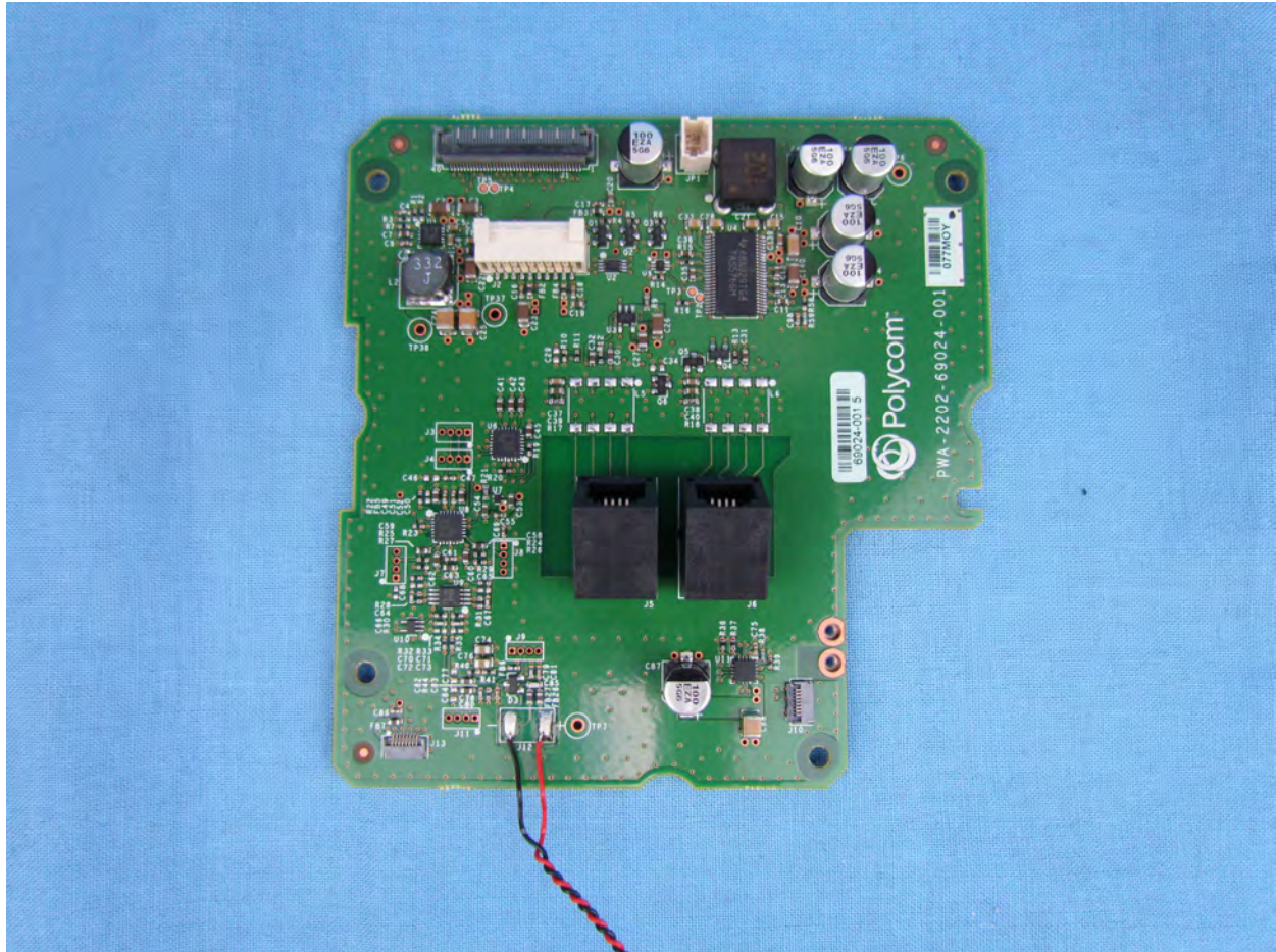
Front Arm PCB Top
