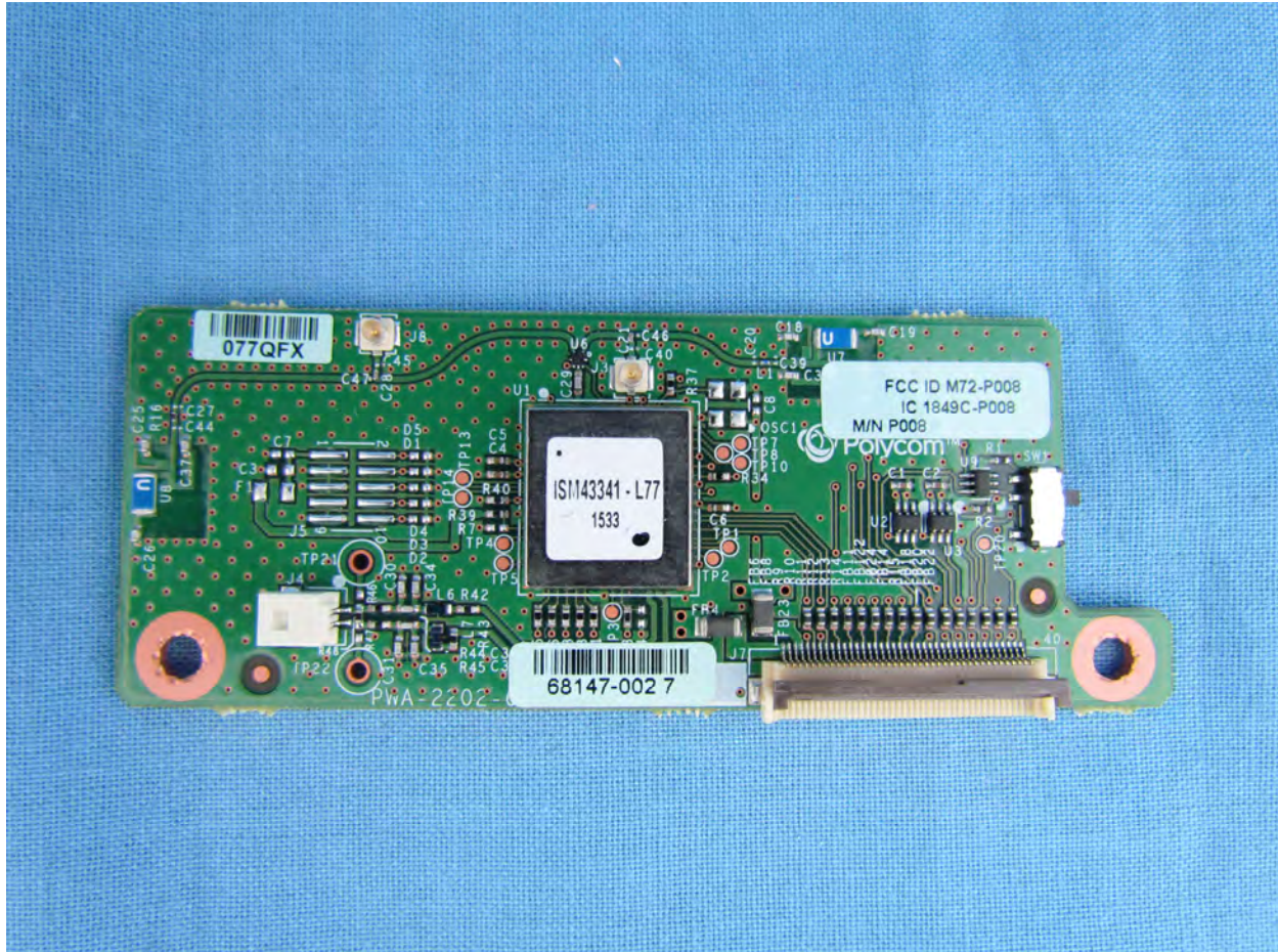
RF Board Top
