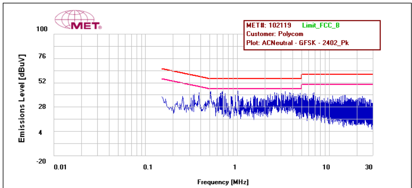
Plot 2. Conducted Emissions, 15.207(a), Neutral Line, GFSK
