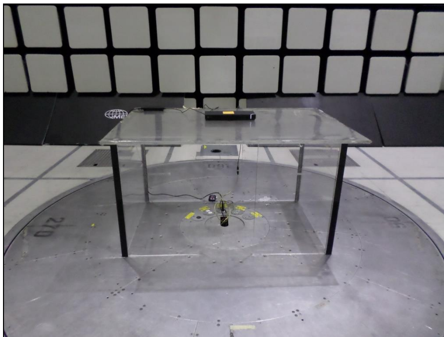
Photograph 3. Radiated Spurious Emissions, Test Setup, Below 1 GHz, Front View
