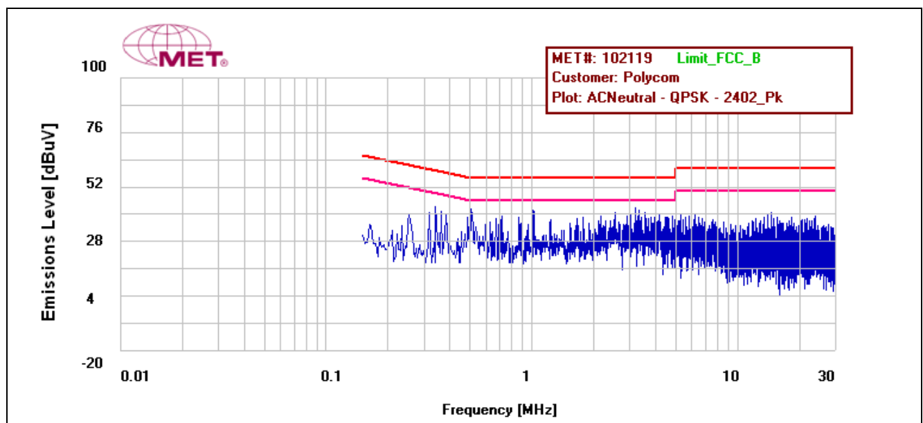
Plot 4. Conducted Emissions, 15.207(a), Neutral Line, QPSK
