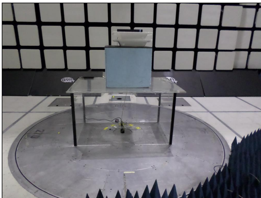
Photograph 6. Radiated Spurious Emissions, Test Setup, Above 1 GHz, Front View
