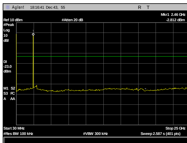
Plot 20. Conducted Spurious Emissions, Mid Channel, 30 MHz – 25 GHz
