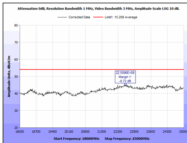
Plot 15. Radiated Spurious Emissions, 18 GHz – 25 GHz
