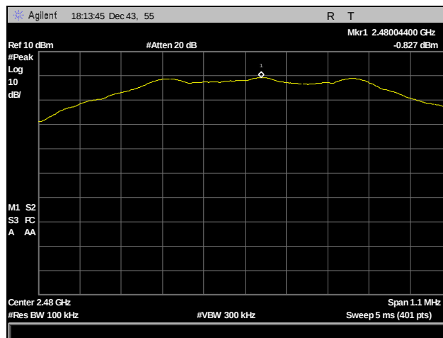
Plot 26. Peak Power Spectral Density, High Channel
