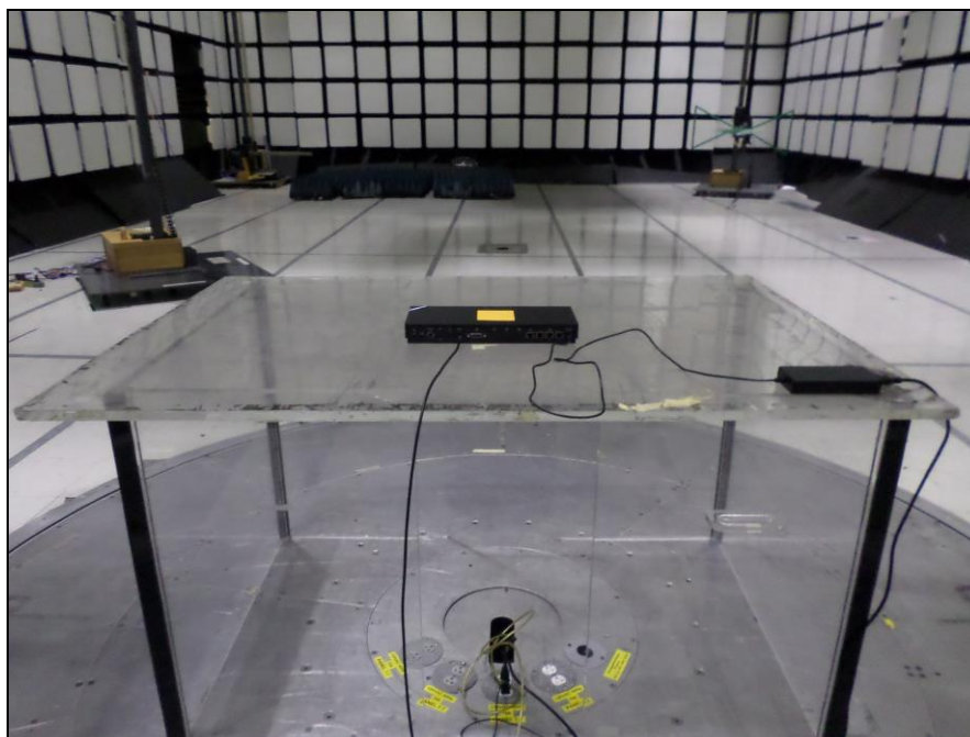
Photograph 4. Radiated Spurious Emissions, Test Setup, Below 1 GHz, Rear View
