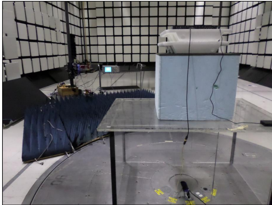
Photograph 9. Radiated Spurious Emissions, Test Setup, Above 18 GHz, Rear View
