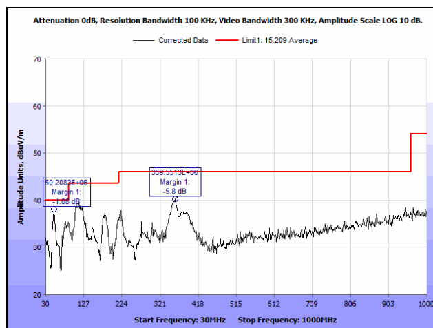
Plot 11. Radiated Spurious Emissions, Mid Channel, 30 MHz – 1 GHz
