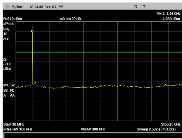
Plot 21. Conducted Spurious Emissions, High Channel, 30 MHz – 25 GHz
