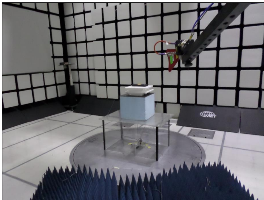
Photograph 8. Radiated Spurious Emissions, Test Setup, 1 GHz – 18 GHz, Antenna View
