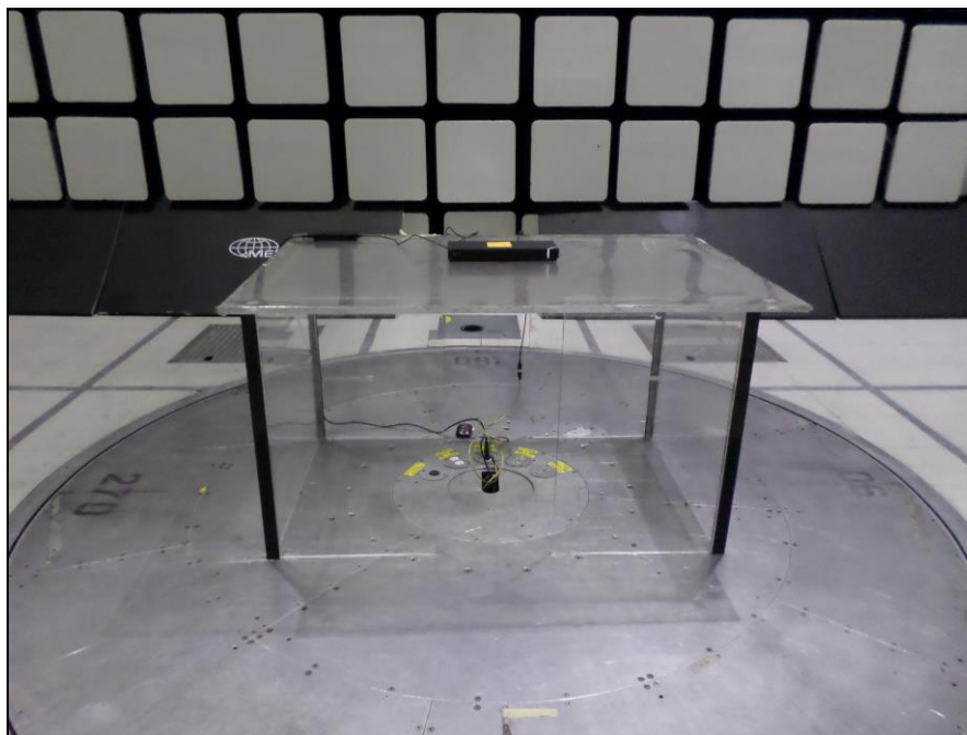
Photograph 3. Radiated Spurious Emissions, Test Setup, Below 1 GHz, Front View
