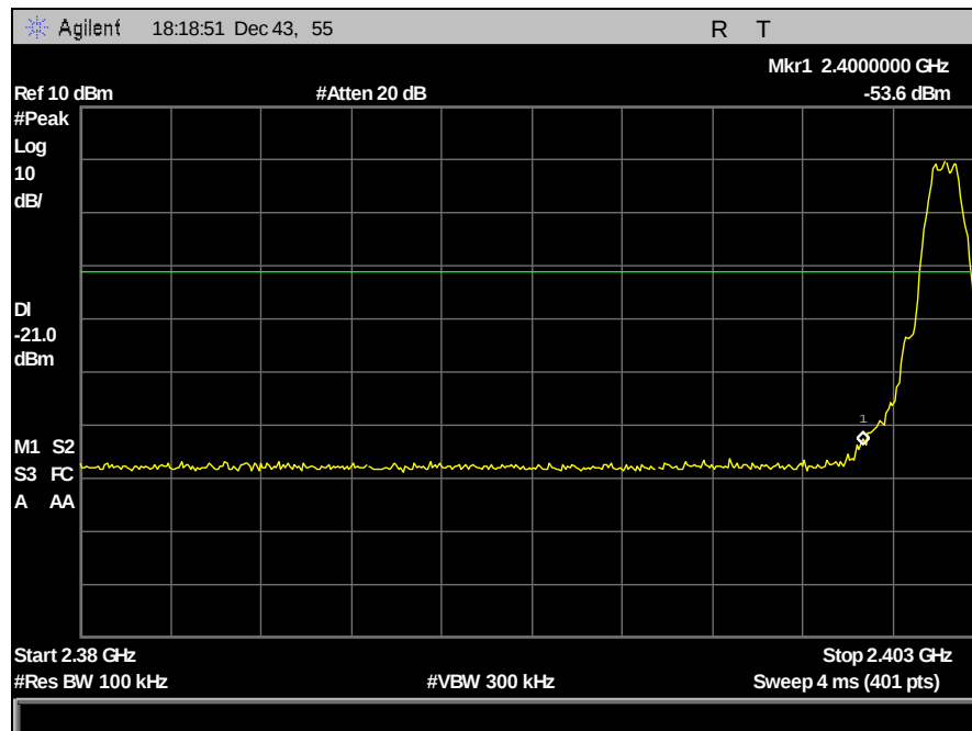
Plot 22. Conducted Band Edge, Low Channel
