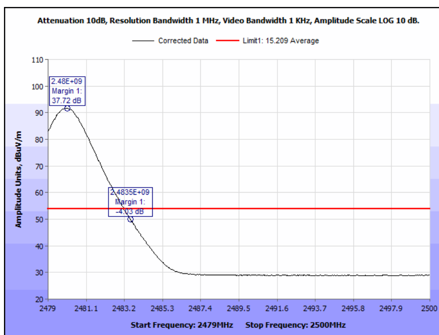
Plot 17. Radiated Restricted Band Edge, High Channel, Average
