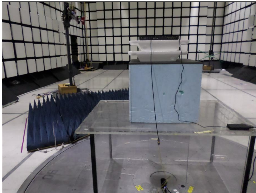
Photograph 7. Radiated Spurious Emissions, Test Setup, 1 GHz – 18 GHz, Rear View
