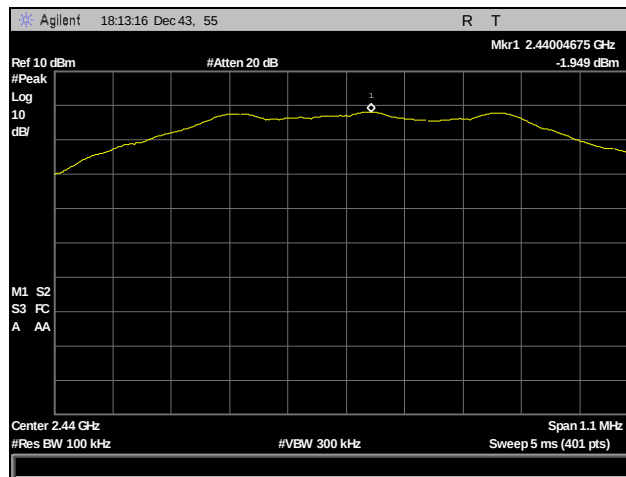
Plot 25. Peak Power Spectral Density, Mid Channel
