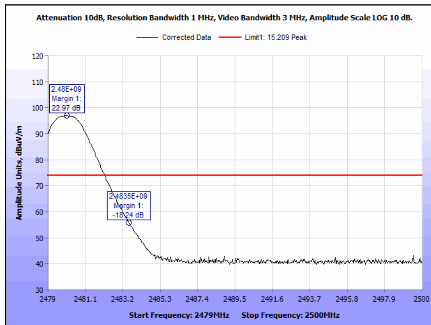
Plot 18. Radiated Restricted Band Edge, High Channel, Peak
