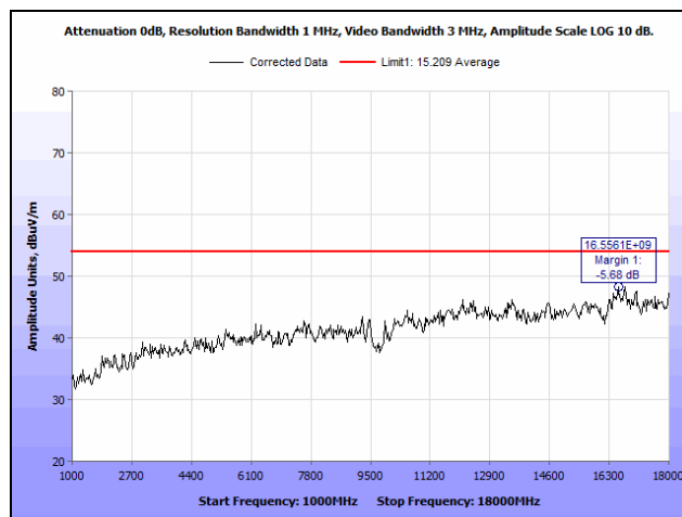
Plot 12. Radiated Spurious Emissions, Mid Channel, 1 GHz – 18 GHz
