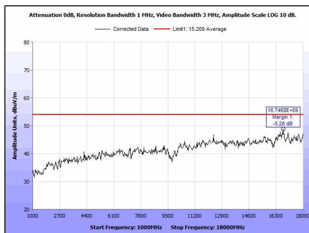
Plot 10. Radiated Spurious Emissions, Low Channel, 1 GHz – 18 GHz
