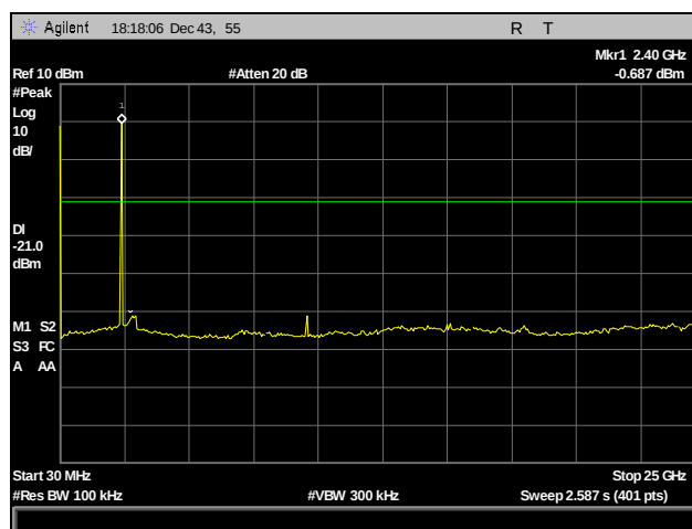
Plot 19. Conducted Spurious Emissions, Low Channel, 30 MHz – 25 GHz
