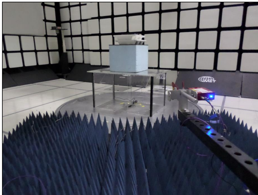
Photograph 10. Radiated Spurious Emissions, Test Setup, Above 18 GHz, Antenna View
