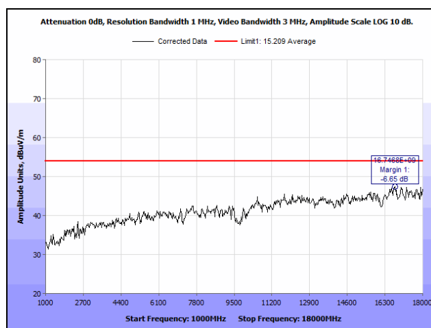
Plot 14. Radiated Spurious Emissions, High Channel, 1 GHz – 18 GHz
