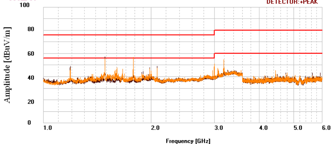
Plot 5. Radiated Emissions, 1 GHz – 6 GHz, Peak Plot
