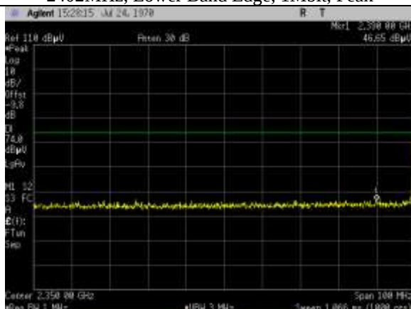
2402MHz, Lower Band Edge, 2Mbit, Peak
