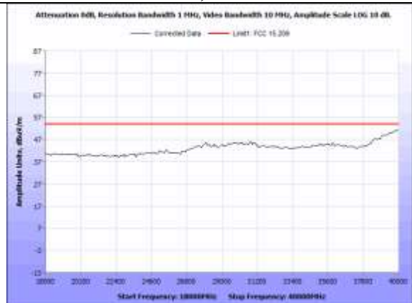
18-40GHz, Horizontal
