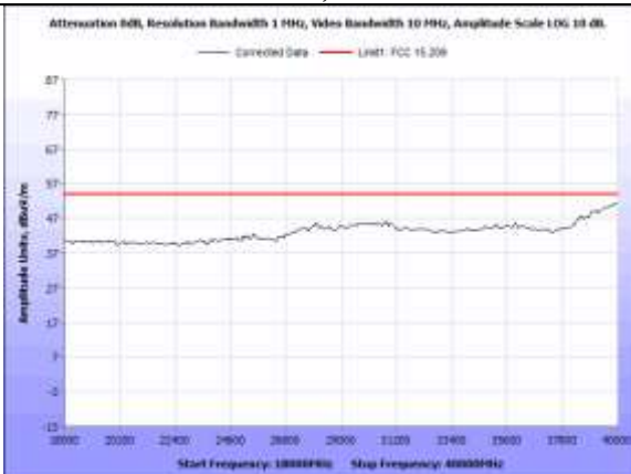
18-40GHz, Vertical
