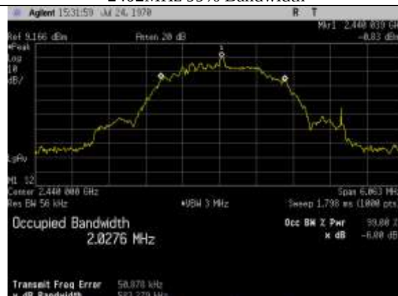
2440MHz 99% Bandwidth
