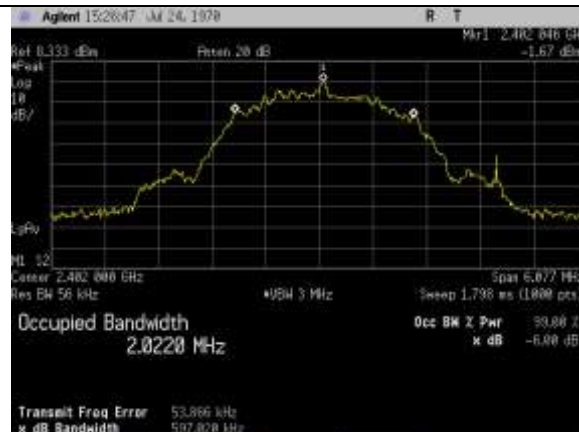
2402MHz 99% Bandwidth
