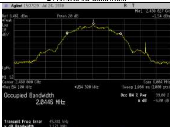
2480MHz 6B Bandwidth
