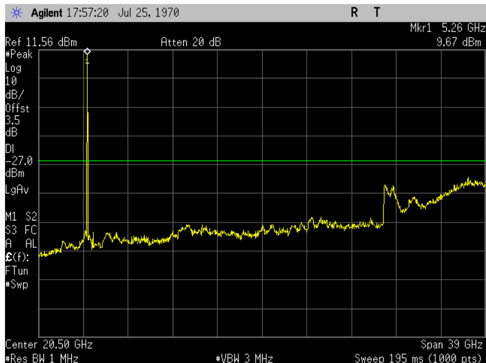
U-NII-2A_5260MHz_low_mid Ch_52_20MHz BW_a-mode_-27dBm_1-40GHz_Port 2
