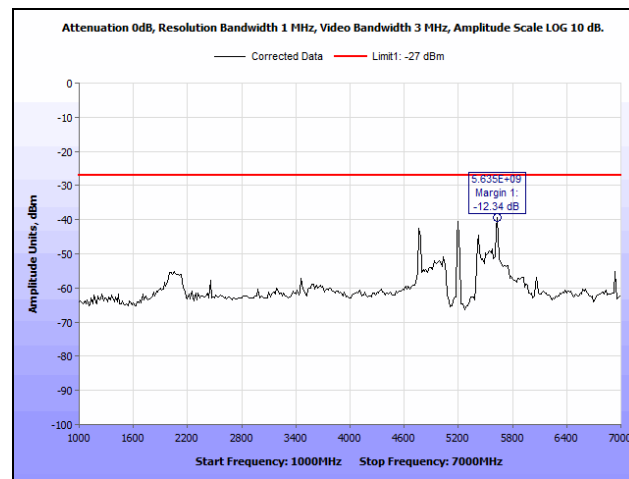
Plot 23. Radiated Spurious Emissions, 802.11a 20 MHz, 5200 MHz, Both Chains, 1 GHz – 7 GHz
