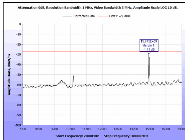
Plot 27. Radiated Spurious Emissions, 802.11a 20 MHz, 5240 MHz, Both Chains, 7 GHz – 18 GHz
