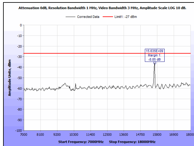
Plot 33. Radiated Spurious Emissions, 802.11n 20 MHz, 5200 MHz, Both Chains, 7 GHz – 18 GHz
