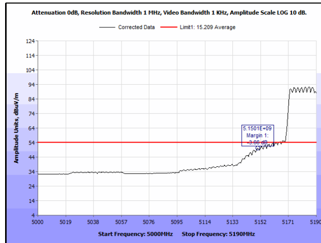
Plot 51. Radiated Band Edge, 802.11n 40 MHz, 5190 MHz, Both Chains, Average
