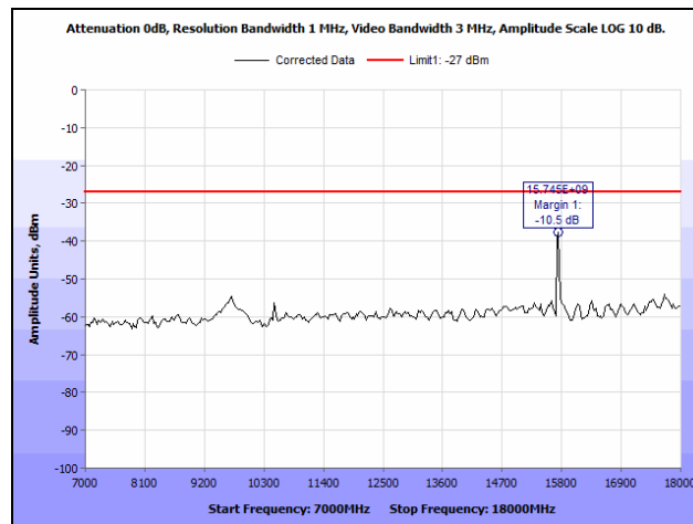
Plot 36. Radiated Spurious Emissions, 802.11n 20 MHz, 5240 MHz, Both Chains, 7 GHz – 18 GHz
