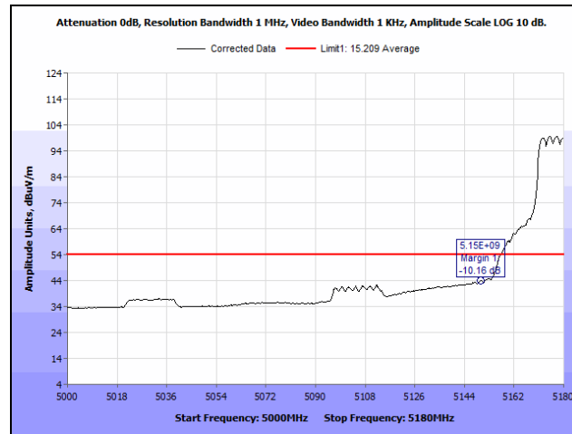
Plot 47. Radiated Band Edge, 802.11n 20 MHz, 5180 MHz, Both Chains, Average
