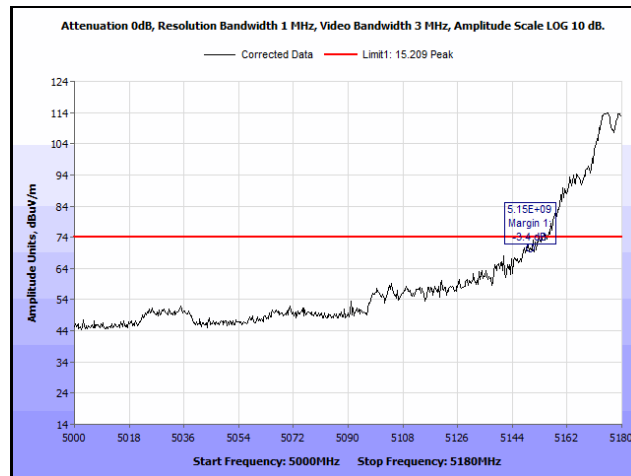
Plot 44. Radiated Band Edge, 802.11a 20 MHz, 5180 MHz, Both Chains, Peak
