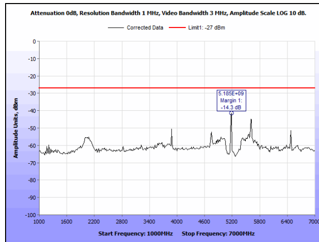
Plot 29. Radiated Spurious Emissions, 802.11n 20 MHz, 5180 MHz, Both Chains, 1 GHz – 7 GHz
