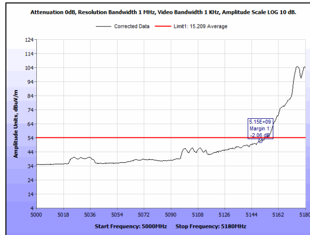
Plot 43. Radiated Band Edge, 802.11a 20 MHz, 5180 MHz, Both Chains, Average
