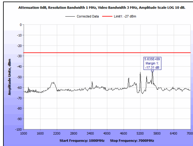
Plot 32. Radiated Spurious Emissions, 802.11n 20 MHz, 5200 MHz, Both Chains, 1 GHz – 7 GHz
