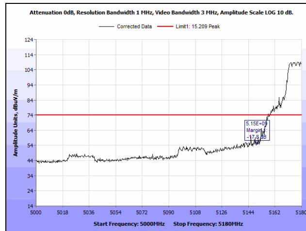
Plot 48. Radiated Band Edge, 802.11n 20 MHz, 5180 MHz, Both Chains, Peak
