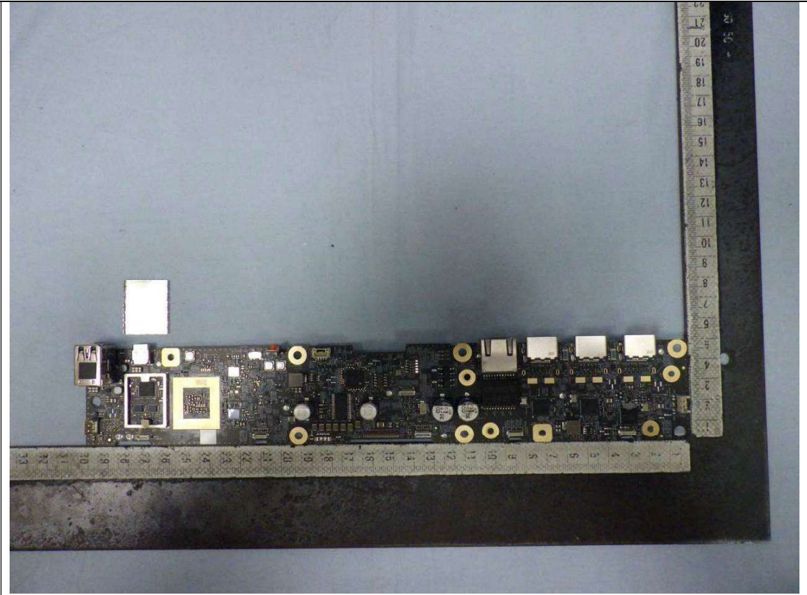
Top view - 2 of main board of the EUT (Removed heatsink)
