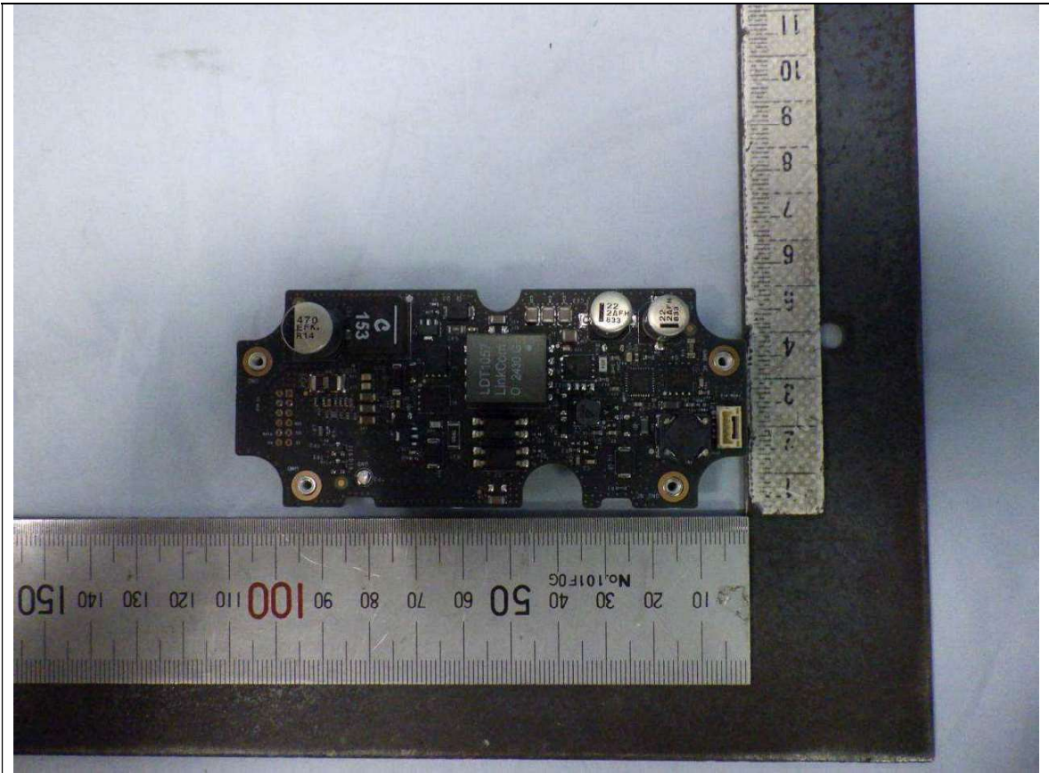
Bottom view of PoE board of the EUT
