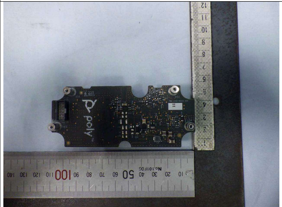
Top view of PoE board of the EUT
