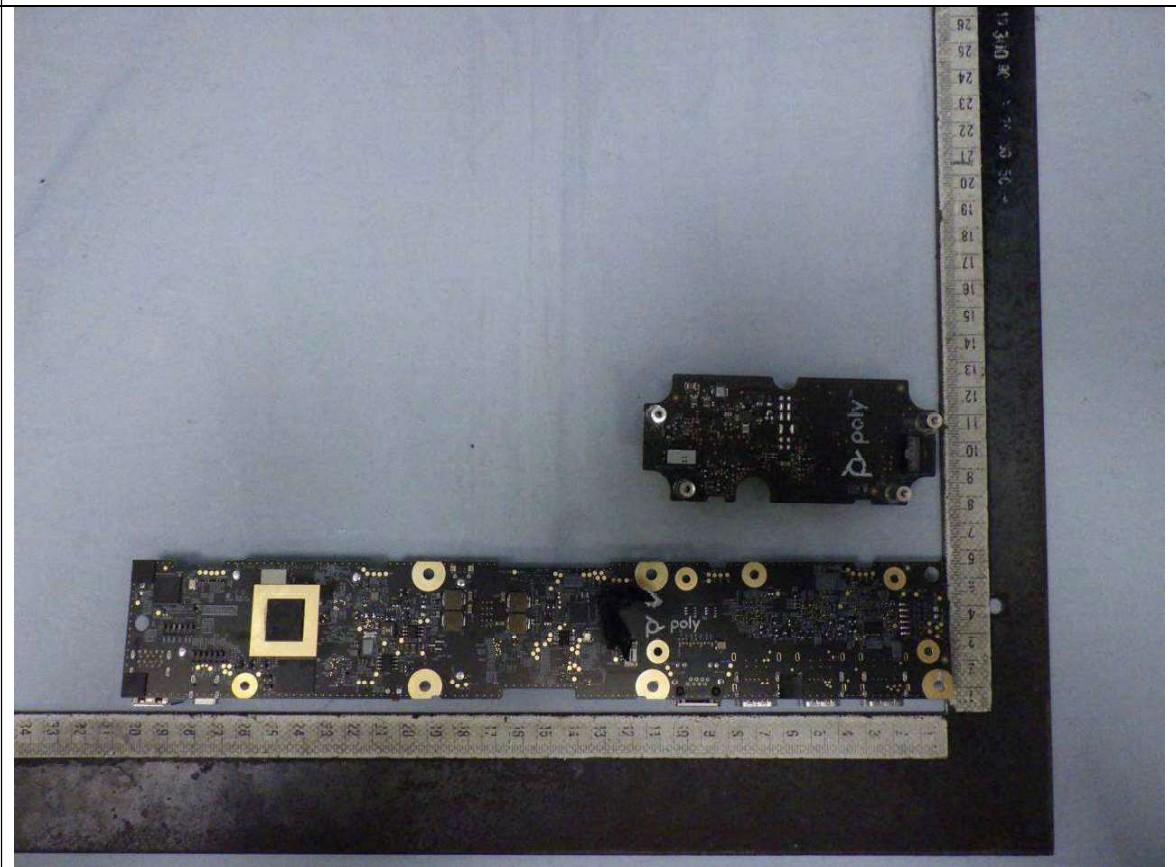
Bottom view - 2 of main board of the EUT (Removed PoE board)
