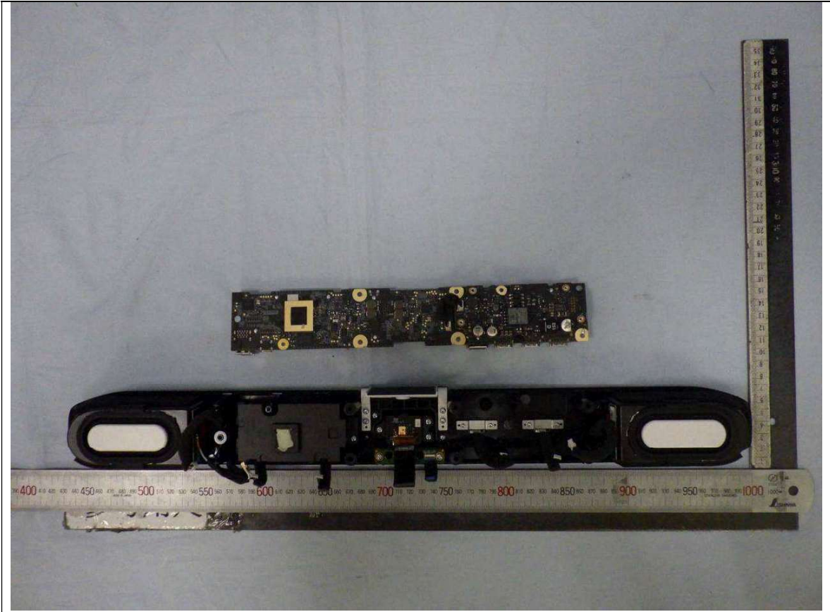
Internal view - 5 of the EUT
