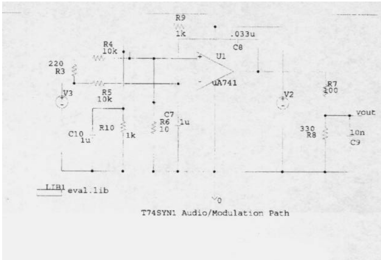
Schematics, Audio Filter, LPF
