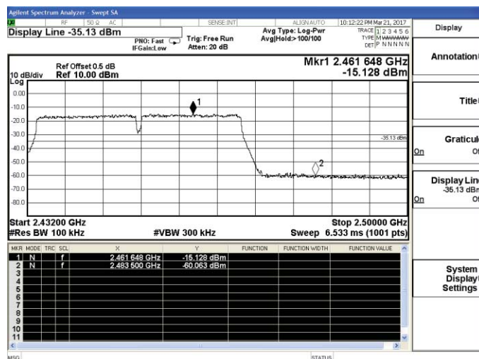
802.11n-HT40-High channel
