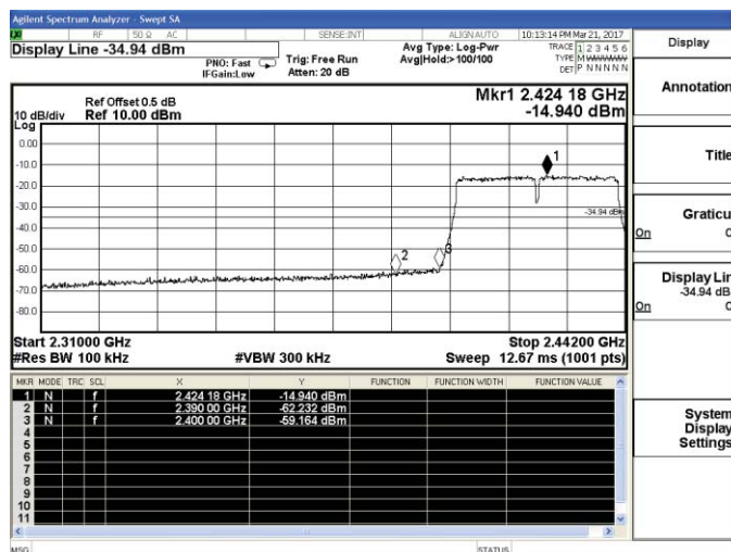
802.11n-HT40-Low channel
