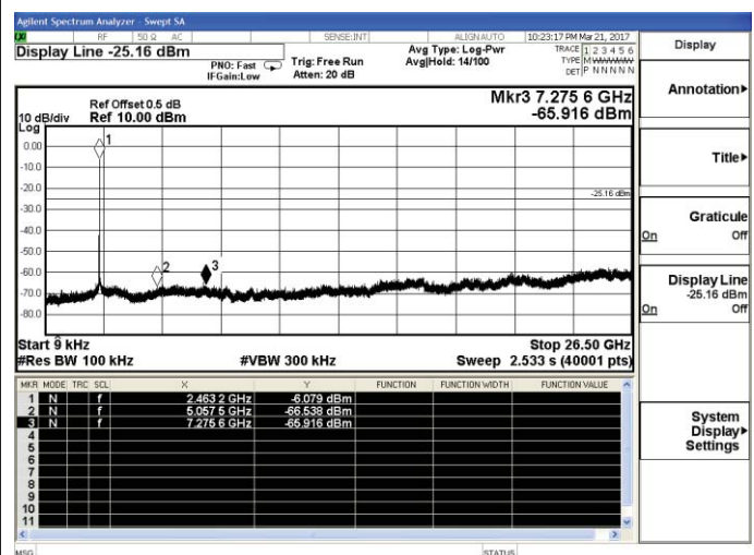
802.11b-High channel
