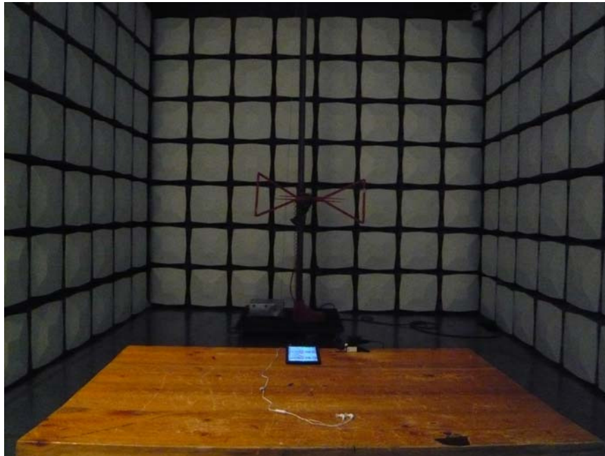
Radiated Emissions –Front View (Charging&Playing Below 1GHz)
