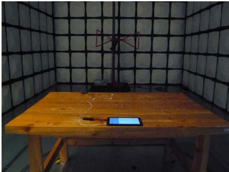
Radiated Emissions –Rear View (Connect to U-disk Below 1GHz)
