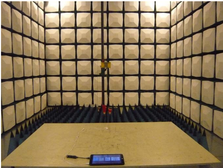
Radiated Emission –Rear View (Connect to U-disk Above 1 GHz)
