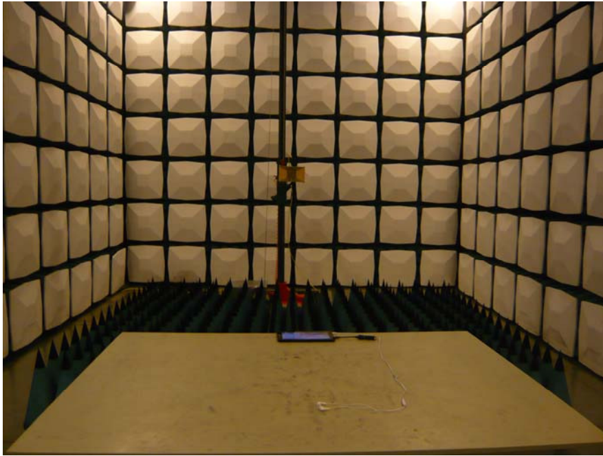
Radiated Emission –Front View (Connect to U-disk Above 1 GHz)
