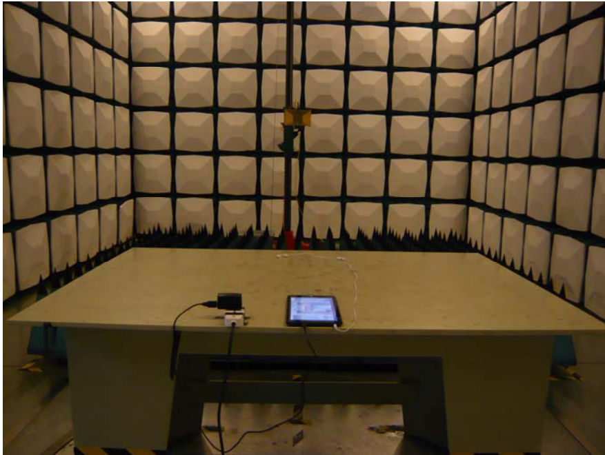
Radiated Emission –Rear View (Charging&Playing Above 1 GHz)
