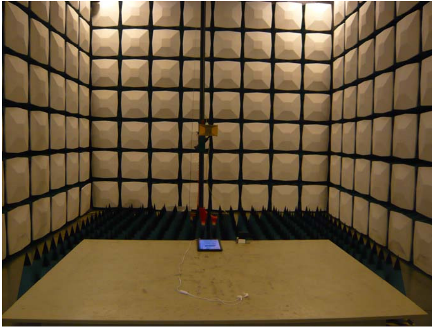
Radiated Emission –Front View (Charging&Playing Above 1 GHz)
