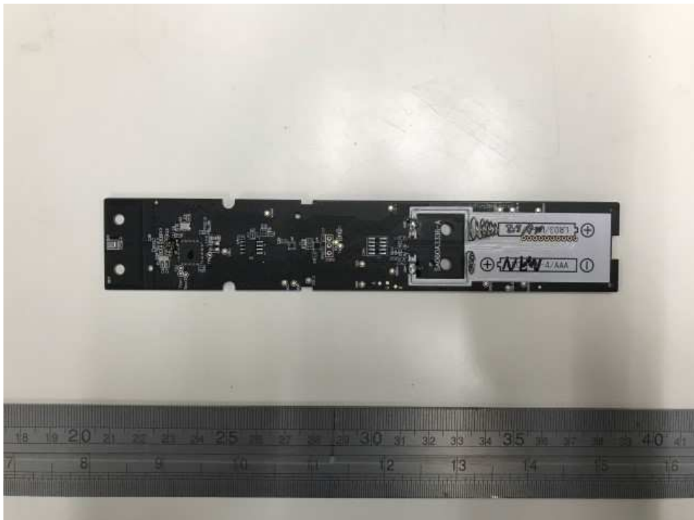
Internal View (Model: BW7630UN)
