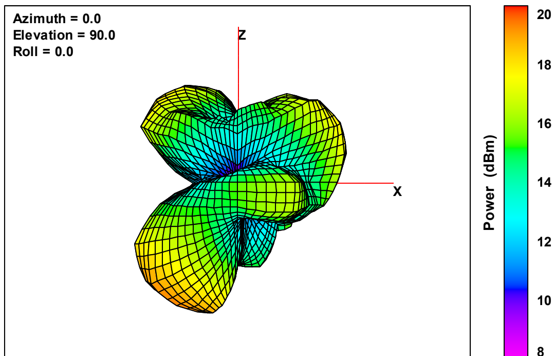
Ant. 2 Free-Space Total EIRP, Left Side View, 5180 MHz
