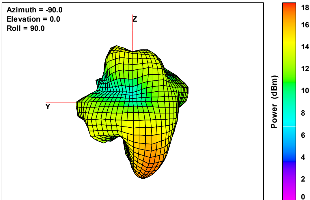
Ant. 2 Free-Space Total EIRP, Back Face View, 5700 MHz
