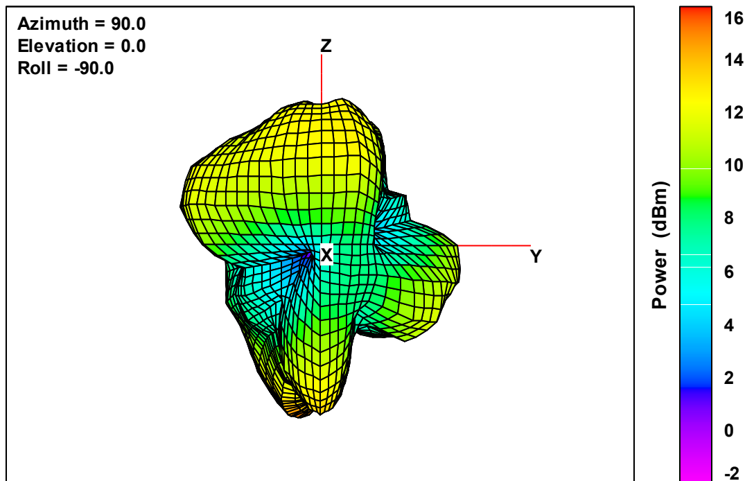
Ant. 2 Free-Space Total EIRP, Front Face View, 5785 MHz
