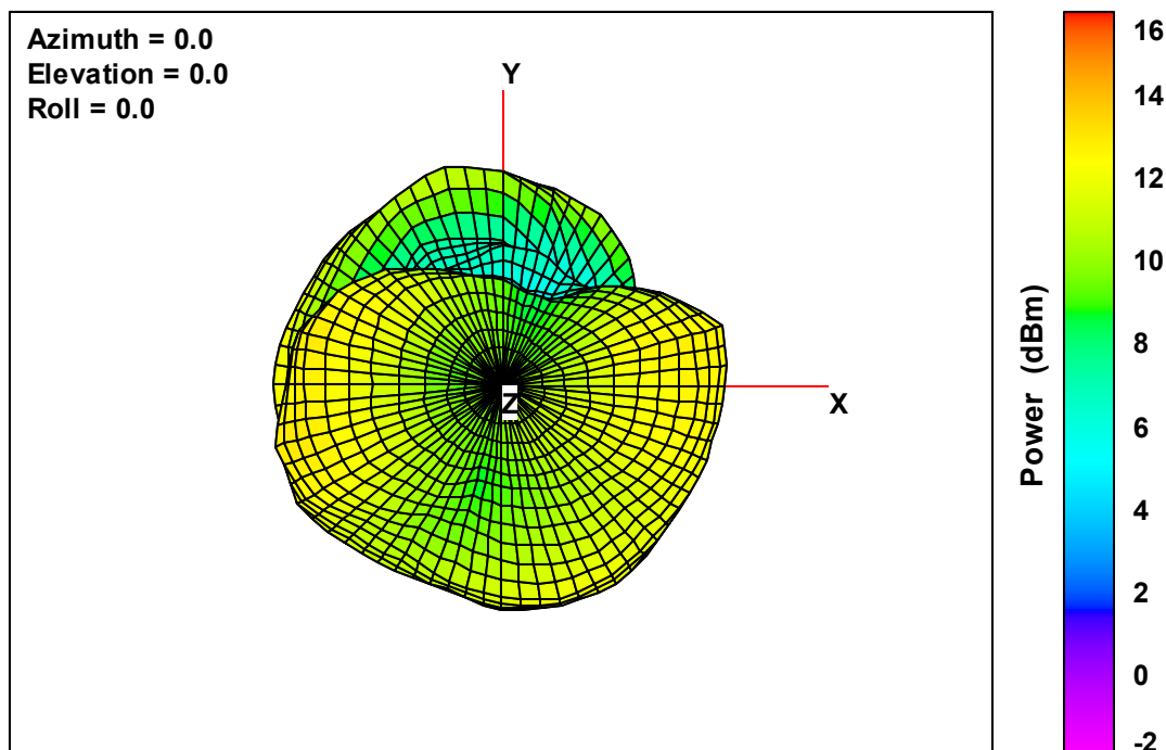
Ant. 2 Free-Space Total EIRP, Top View, 5785 MHz
