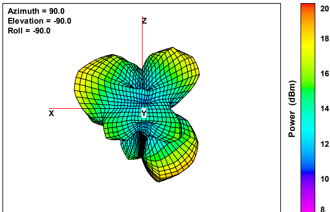
Ant. 2 Free-Space Total EIRP, Right Side View, 5240 MHz
