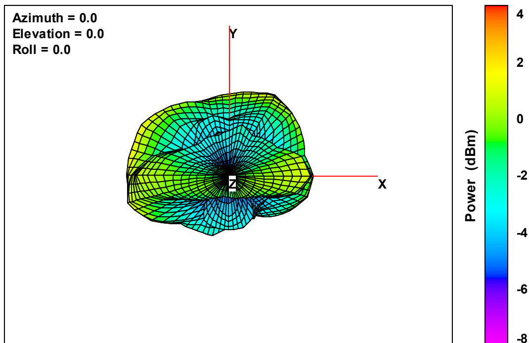
Ant. 3 Free-Space Total EIRP, Top View, 2405 MHz
