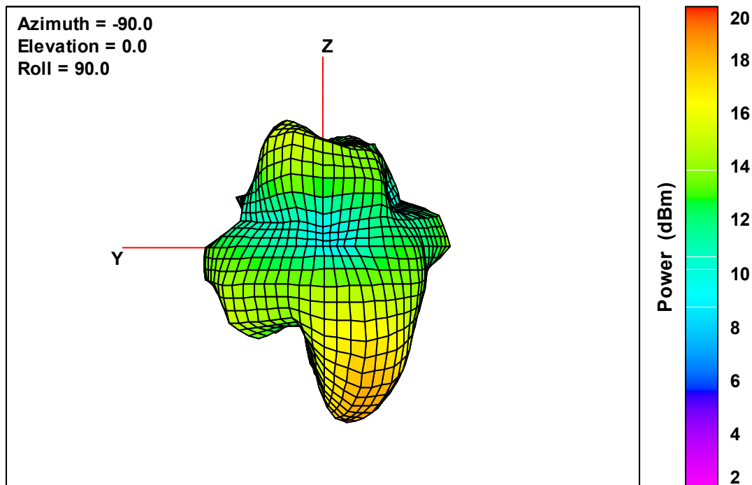
Ant. 2 Free-Space Total EIRP, Back Face View, 5500 MHz
