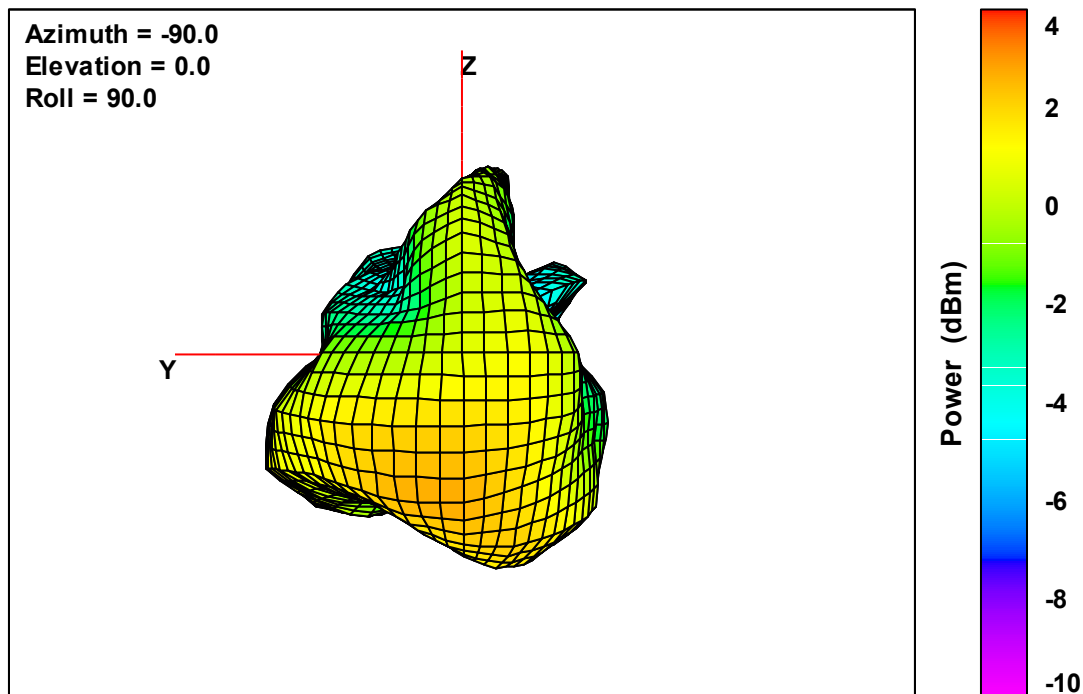
Ant. 3 Free-Space Total EIRP, Back Face View, 2445 MHz
