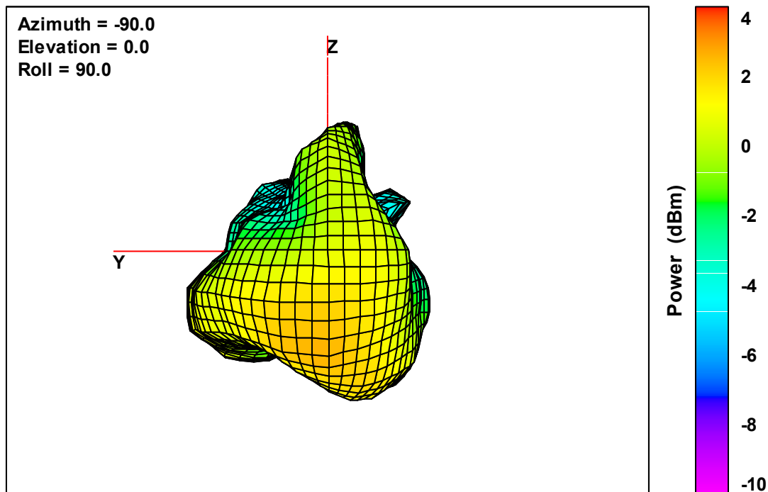
Ant. 3 Free-Space Total EIRP, Back Face View, 2480 MHz
