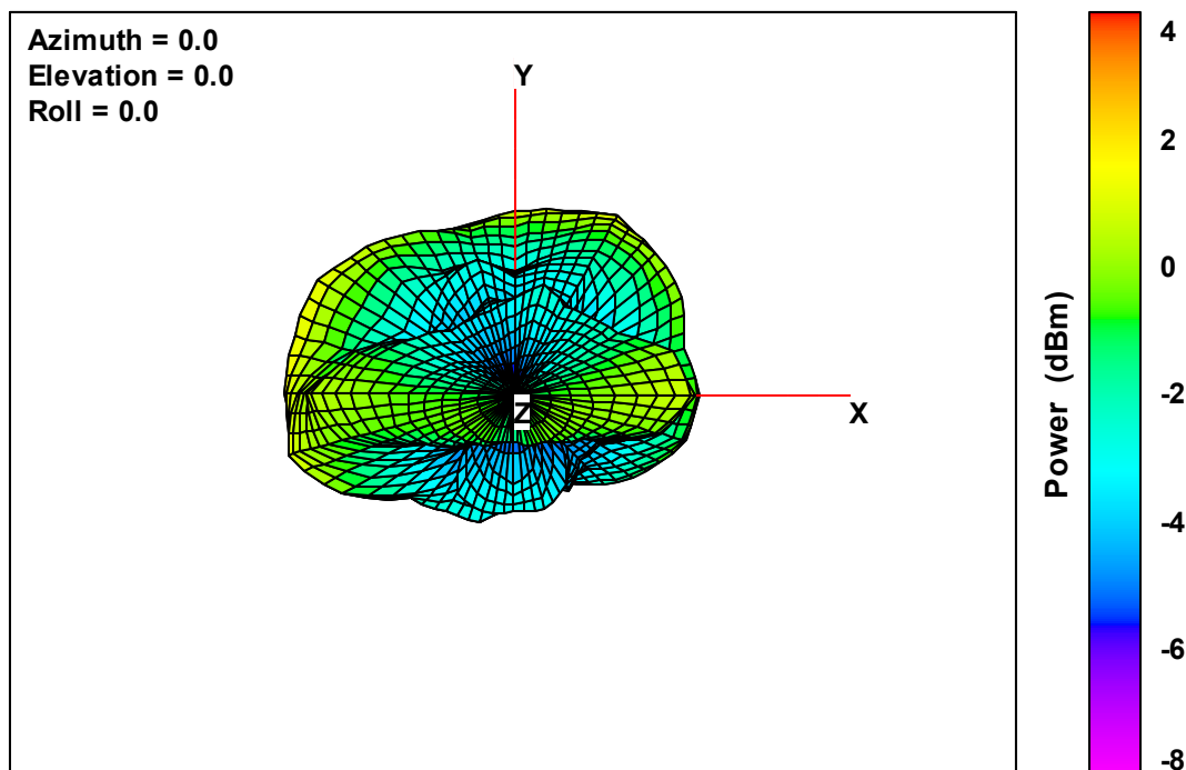
Ant. 3 Free-Space Total EIRP, Top View, 2442 MHz
