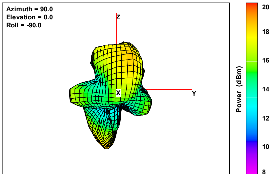
Ant. 2 Free-Space Total EIRP, Front Face View, 5180 MHz
