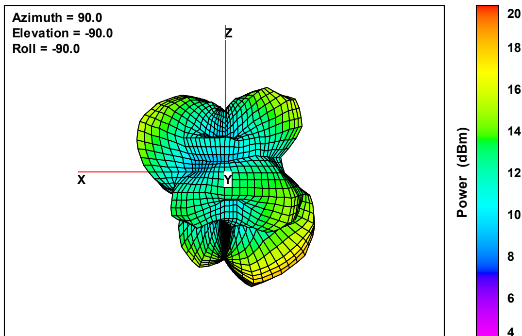
Ant. 2 Free-Space Total EIRP, Right Side View, 5320 MHz
