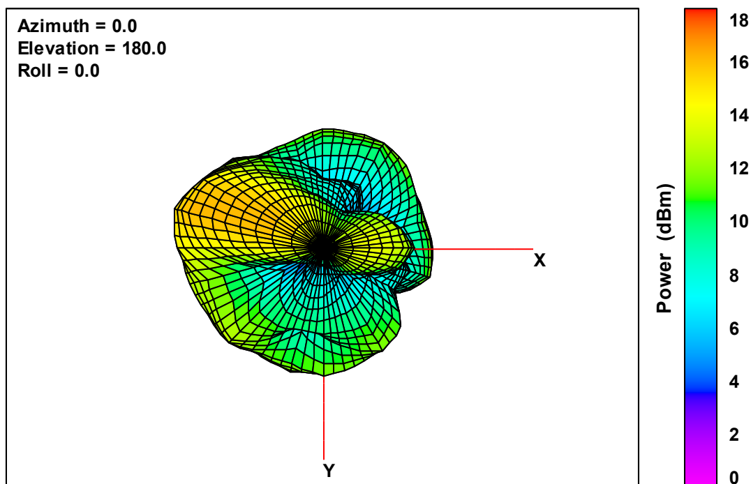
Ant. 2 Free-Space Total EIRP, Bottom View, 5745 MHz
