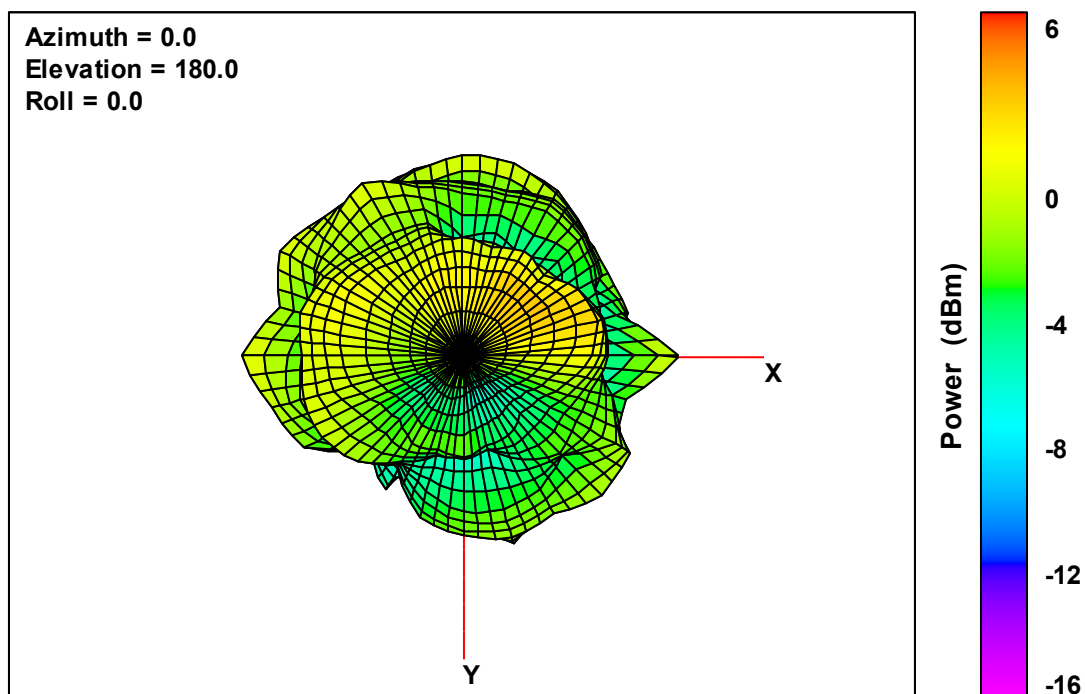
Ant. 2 Free-Space Total EIRP, Bottom View, 5825 MHz
