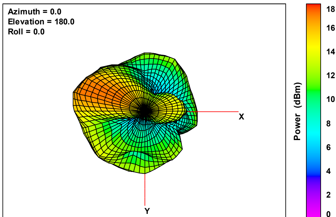
Ant. 2 Free-Space Total EIRP, Bottom View, 5700 MHz
