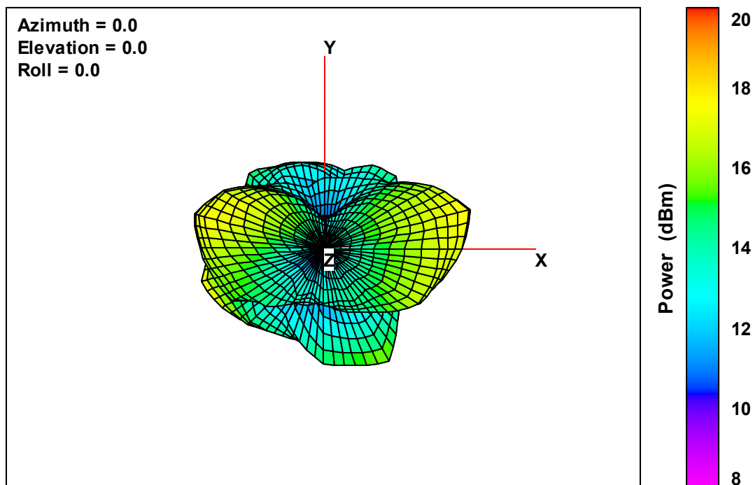
Ant. 2 Free-Space Total EIRP, Top View, 5260 MHz
