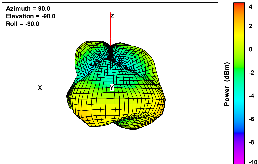
Ant. 3 Free-Space Total EIRP, Right Side View, 2475 MHz
