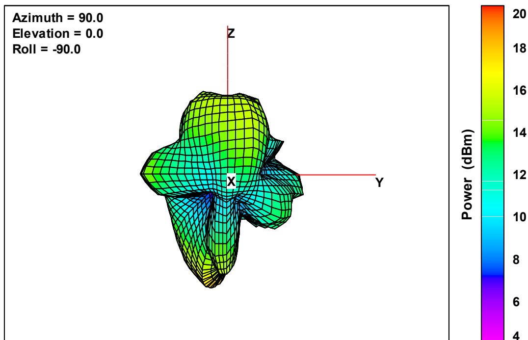
Ant. 2 Free-Space Total EIRP, Front Face View, 5320 MHz
