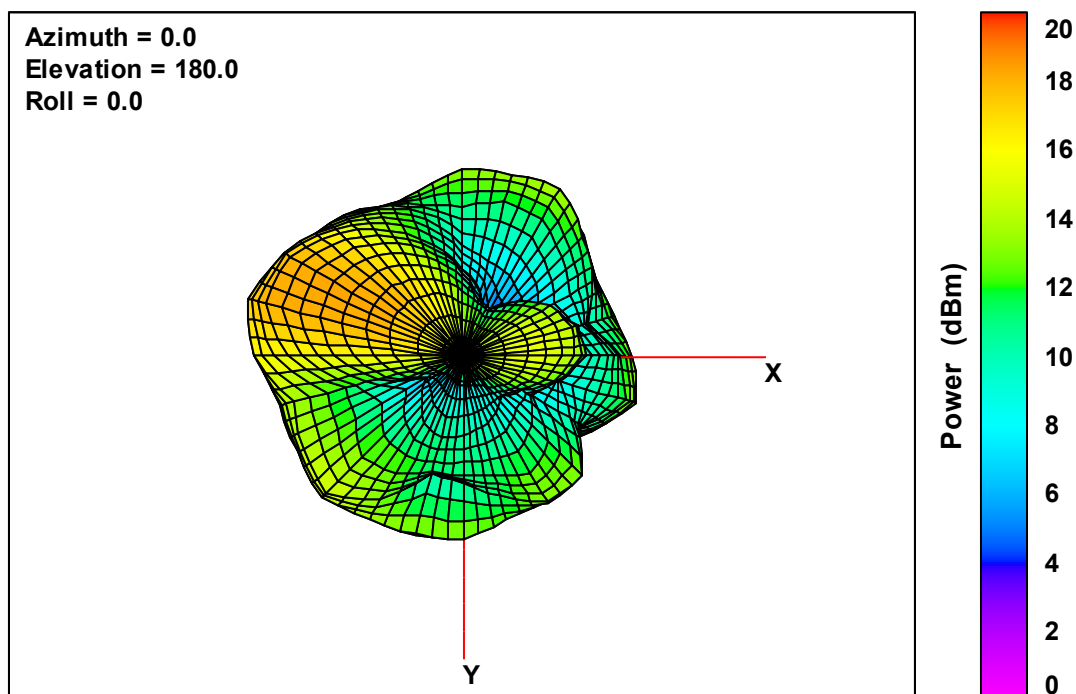
Ant. 2 Free-Space Total EIRP, Bottom View, 5600 MHz
