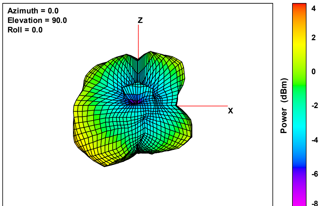
Ant. 3 Free-Space Total EIRP, Left Side View, 2402 MHz
