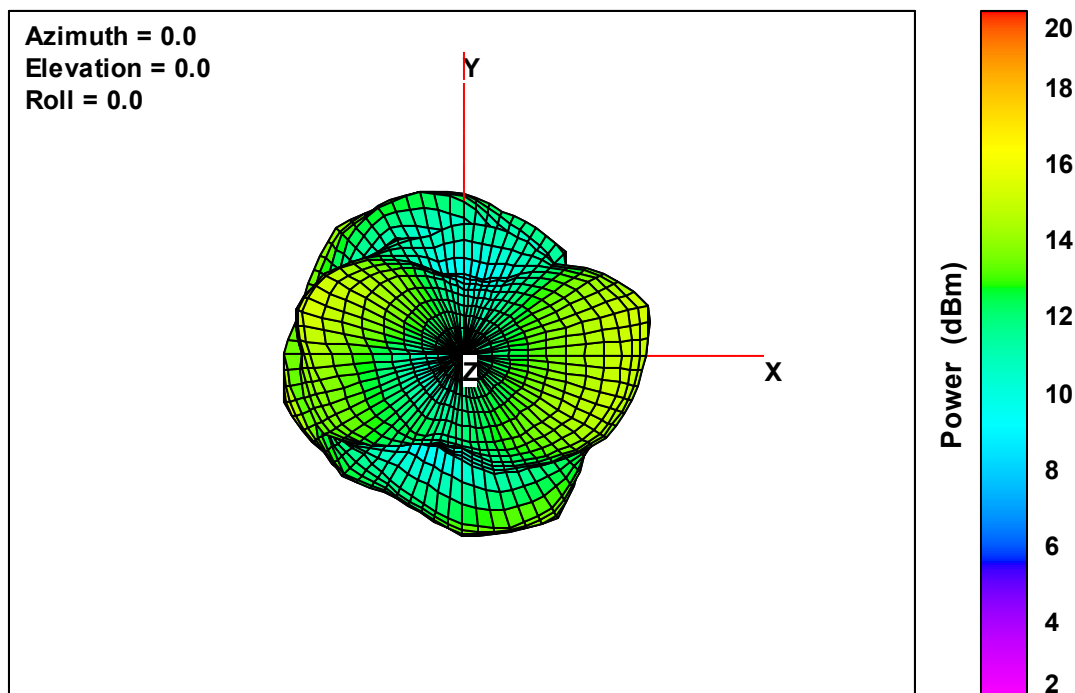
Ant. 2 Free-Space Total EIRP, Top View, 5500 MHz
