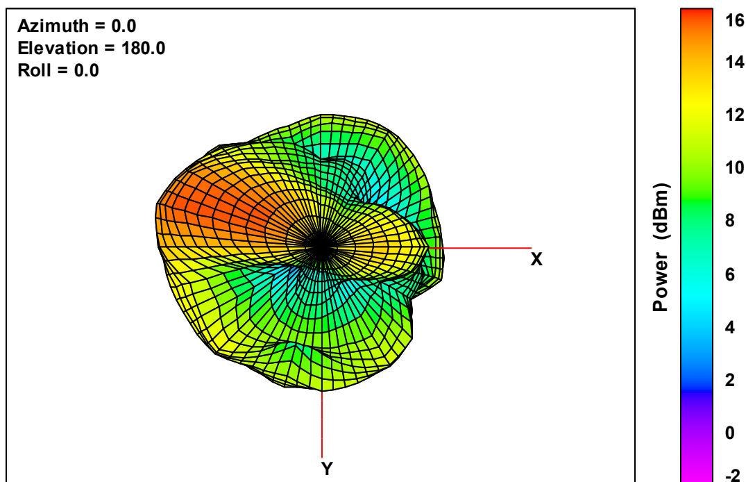
Ant. 2 Free-Space Total EIRP, Bottom View, 5785 MHz
