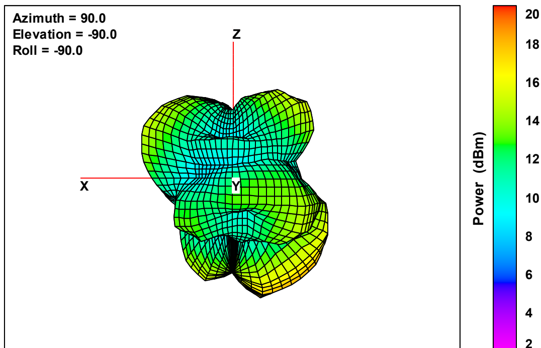
Ant. 2 Free-Space Total EIRP, Right Side View, 5500 MHz
