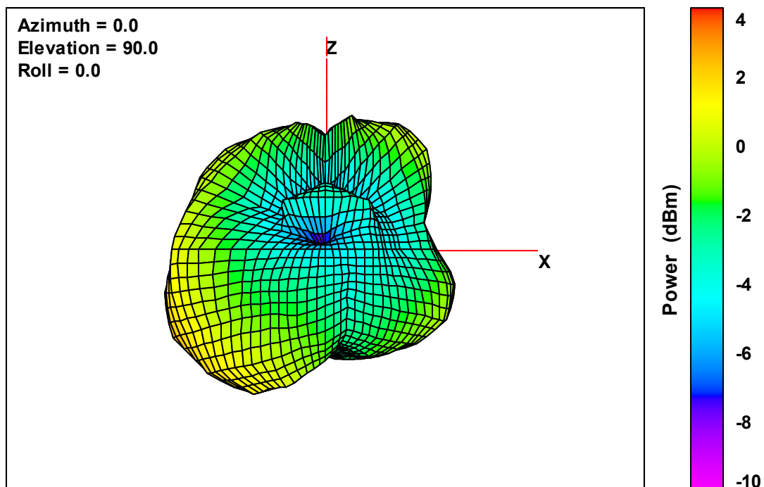
Ant. 3 Free-Space Total EIRP, Left Side View, 2475 MHz
