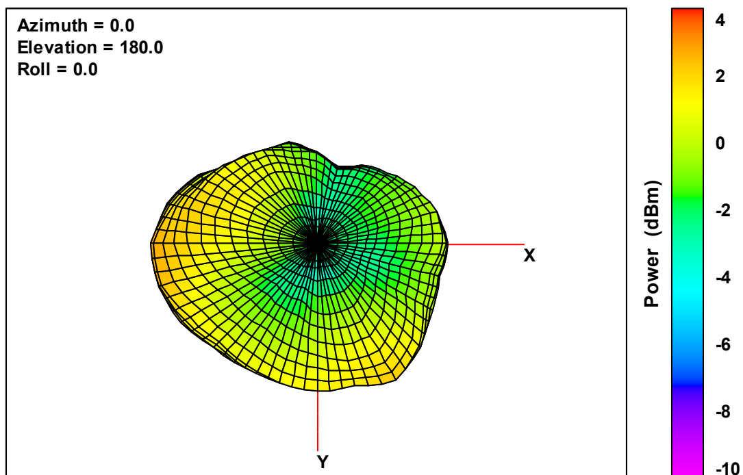
Ant. 3 Free-Space Total EIRP, Bottom View, 2475 MHz
