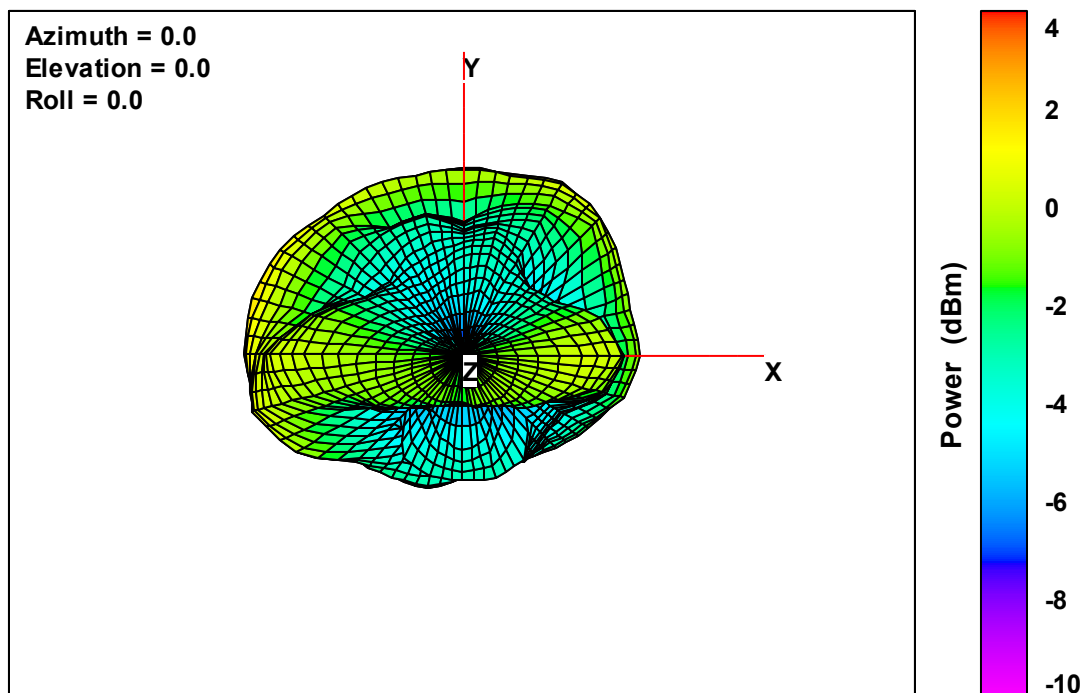
Ant. 3 Free-Space Total EIRP, Top View, 2475 MHz
