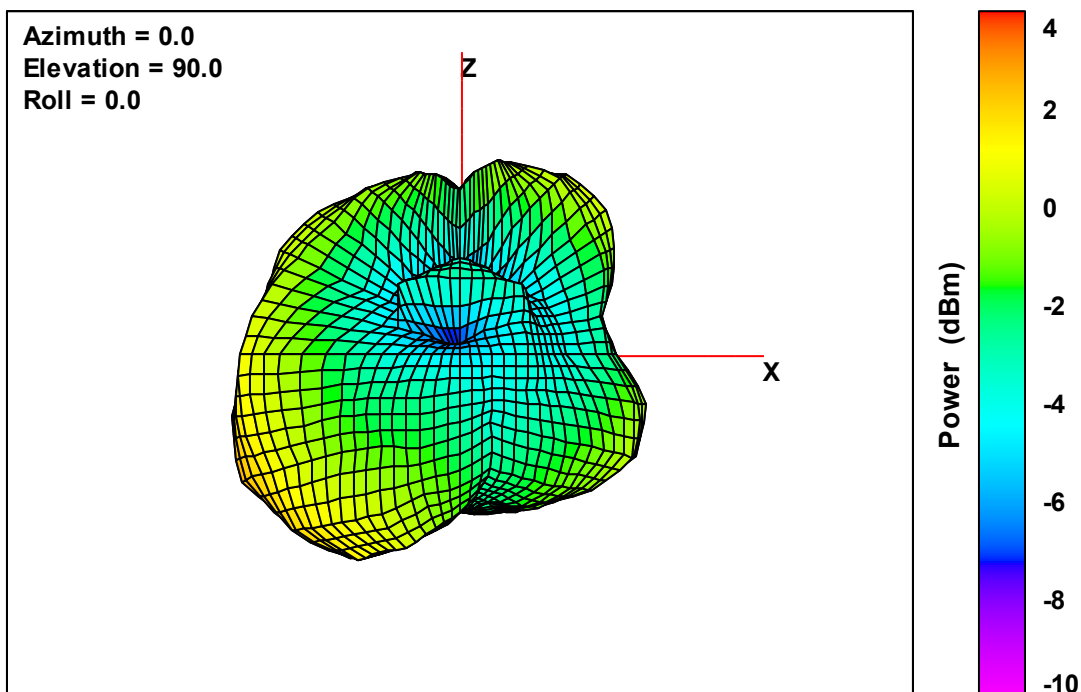
Ant. 3 Free-Space Total EIRP, Left Side View, 2445 MHz
