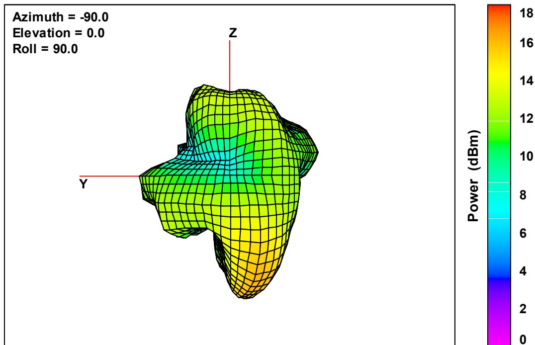
Ant. 2 Free-Space Total EIRP, Back Face View, 5745 MHz
