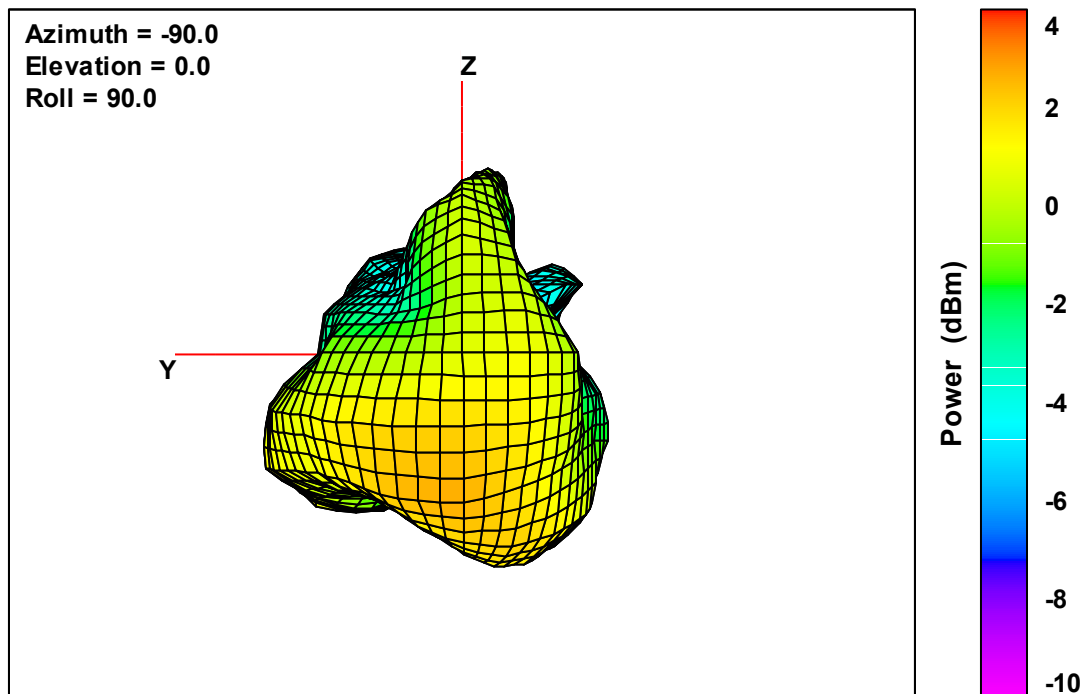
Ant. 3 Free-Space Total EIRP, Back Face View, 2475 MHz
