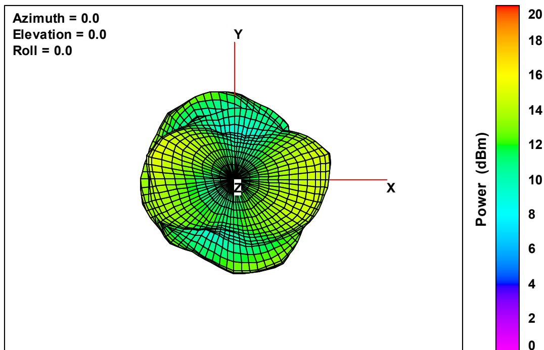
Ant. 2 Free-Space Total EIRP, Top View, 5600 MHz
