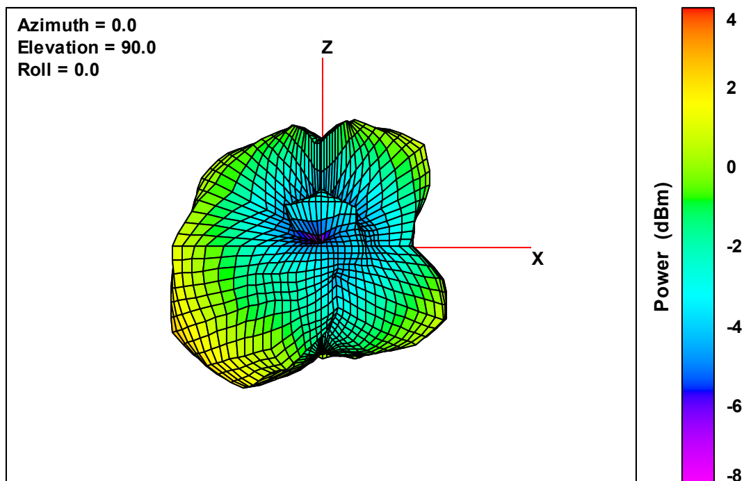
Ant. 3 Free-Space Total EIRP, Left Side View, 2405 MHz
