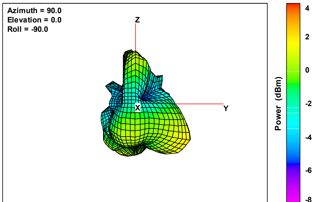
Ant. 3 Free-Space Total EIRP, Front Face View, 2442 MHz
