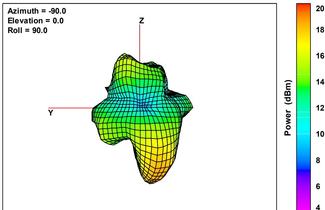
Ant. 2 Free-Space Total EIRP, Back Face View, 5320 MHz
