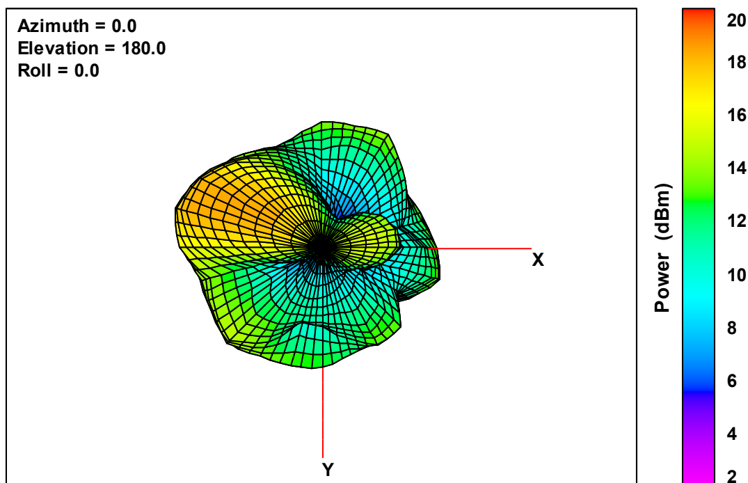
Ant. 2 Free-Space Total EIRP, Bottom View, 5500 MHz
