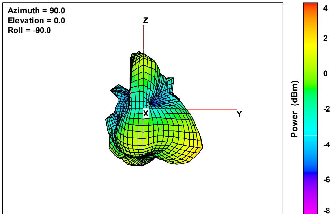
Ant. 3 Free-Space Total EIRP, Front Face View, 2405 MHz
