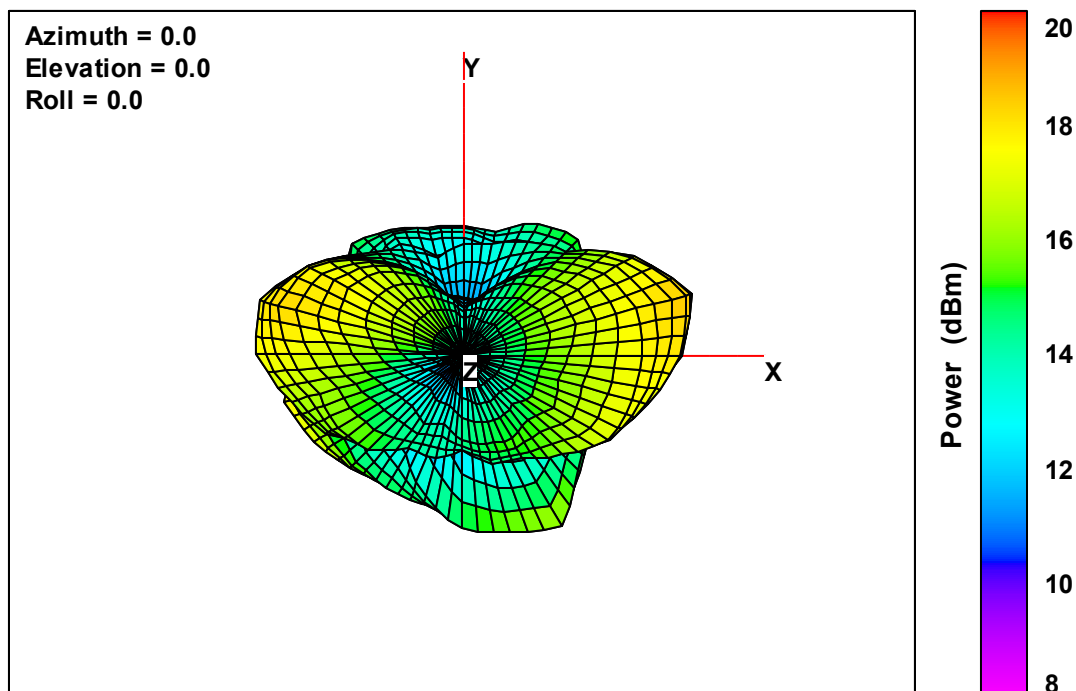
Ant. 2 Free-Space Total EIRP, Top View, 5180 MHz
