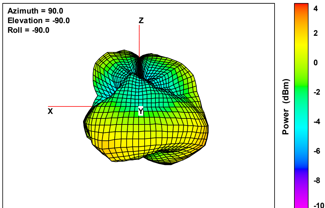
Ant. 3 Free-Space Total EIRP, Right Side View, 2445 MHz
