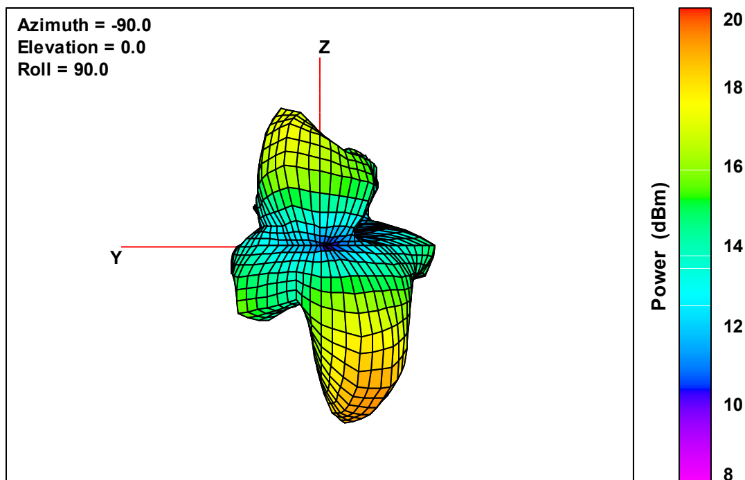
Ant. 2 Free-Space Total EIRP, Back Face View, 5260 MHz
