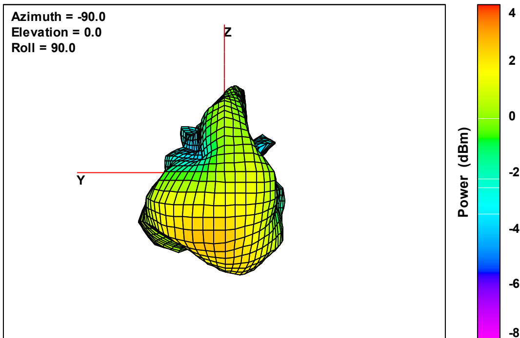
Ant. 3 Free-Space Total EIRP, Back Face View, 2442 MHz
