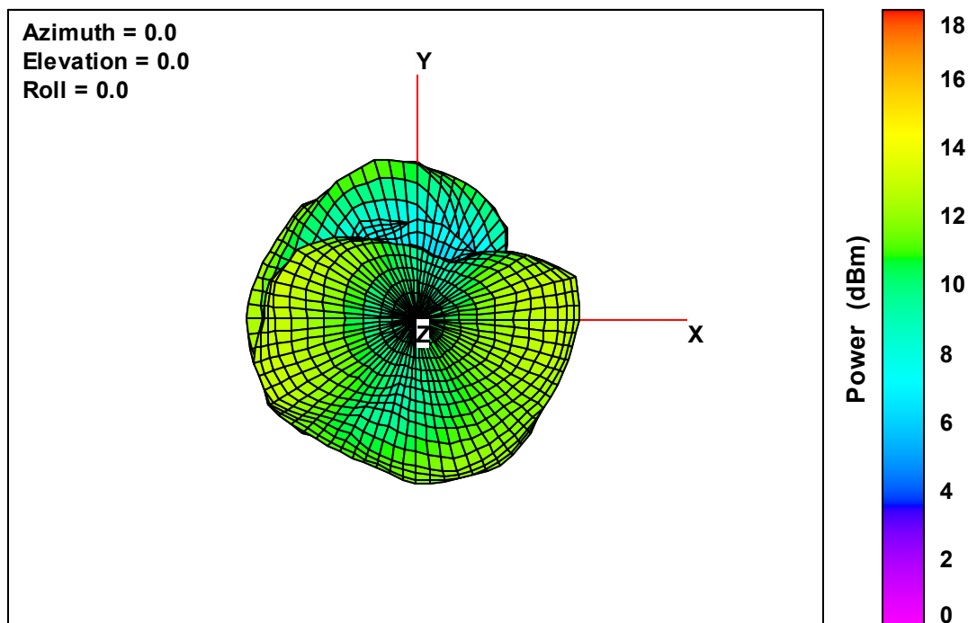
Ant. 2 Free-Space Total EIRP, Top View, 5745 MHz
