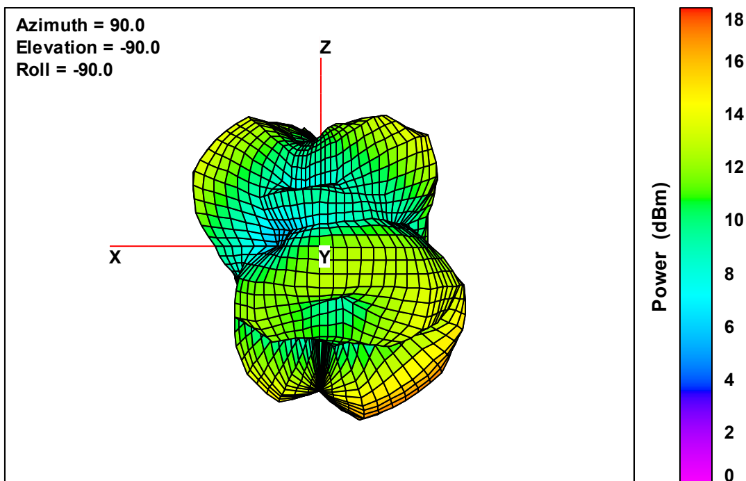
Ant. 2 Free-Space Total EIRP, Right Side View, 5700 MHz
