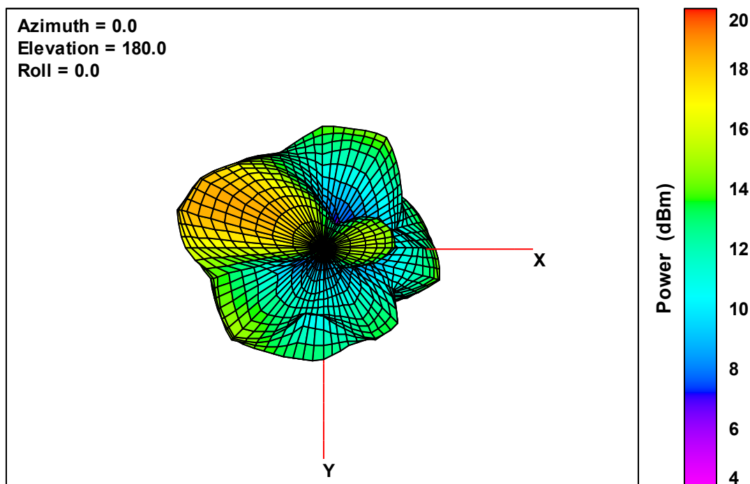
Ant. 2 Free-Space Total EIRP, Bottom View, 5320 MHz
