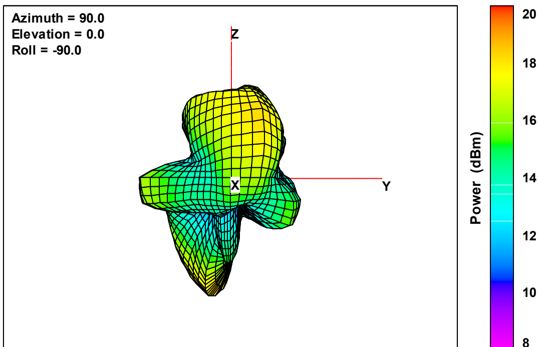
Ant. 2 Free-Space Total EIRP, Front Face View, 5240 MHz
