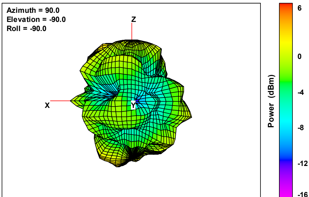
Ant. 2 Free-Space Total EIRP, Right Side View, 5825 MHz
