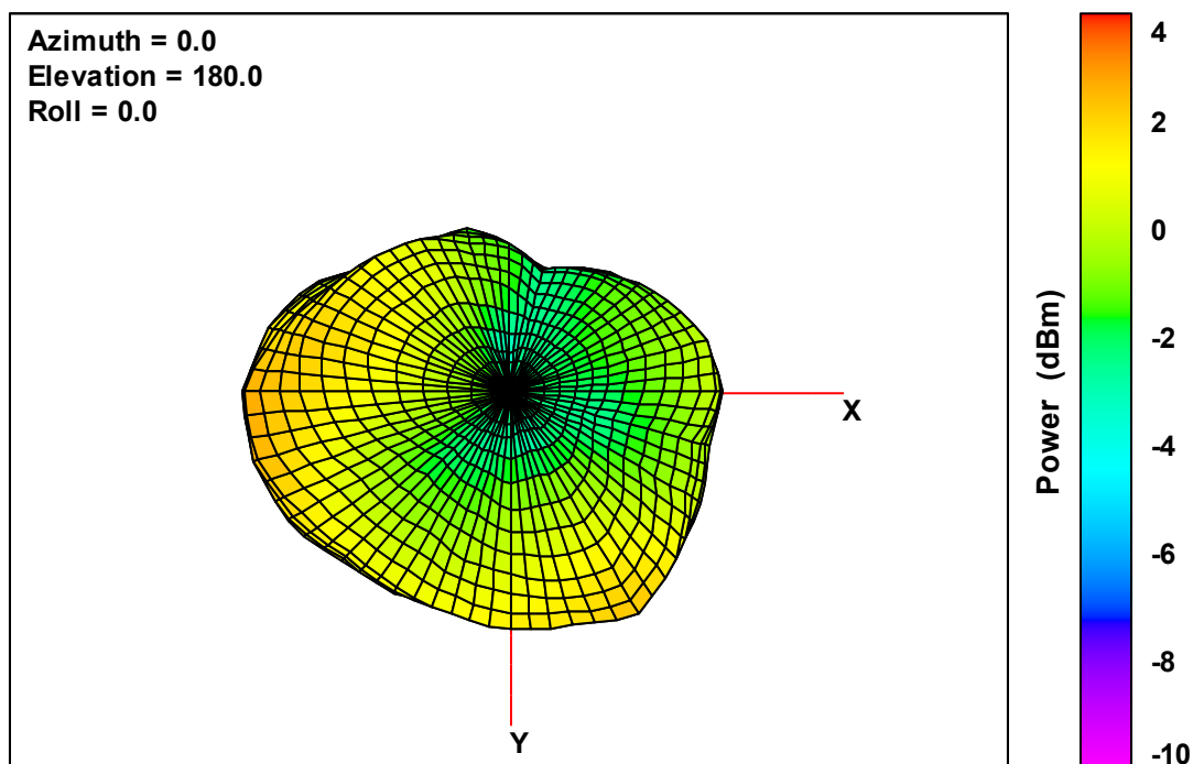
Ant. 3 Free-Space Total EIRP, Bottom View, 2445 MHz
