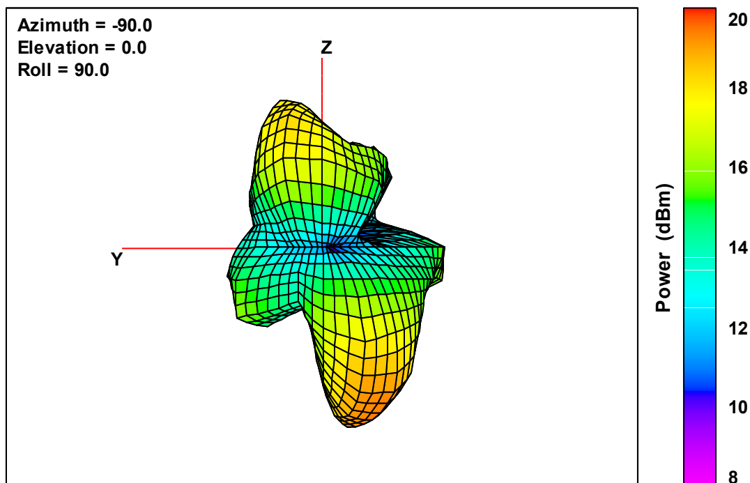
Ant. 2 Free-Space Total EIRP, Back Face View, 5180 MHz
