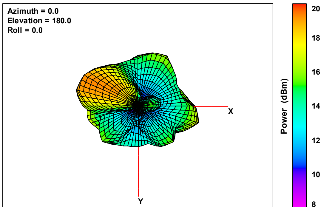
Ant. 2 Free-Space Total EIRP, Bottom View, 5240 MHz
