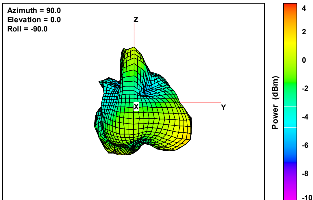
Ant. 3 Free-Space Total EIRP, Front Face View, 2480 MHz
