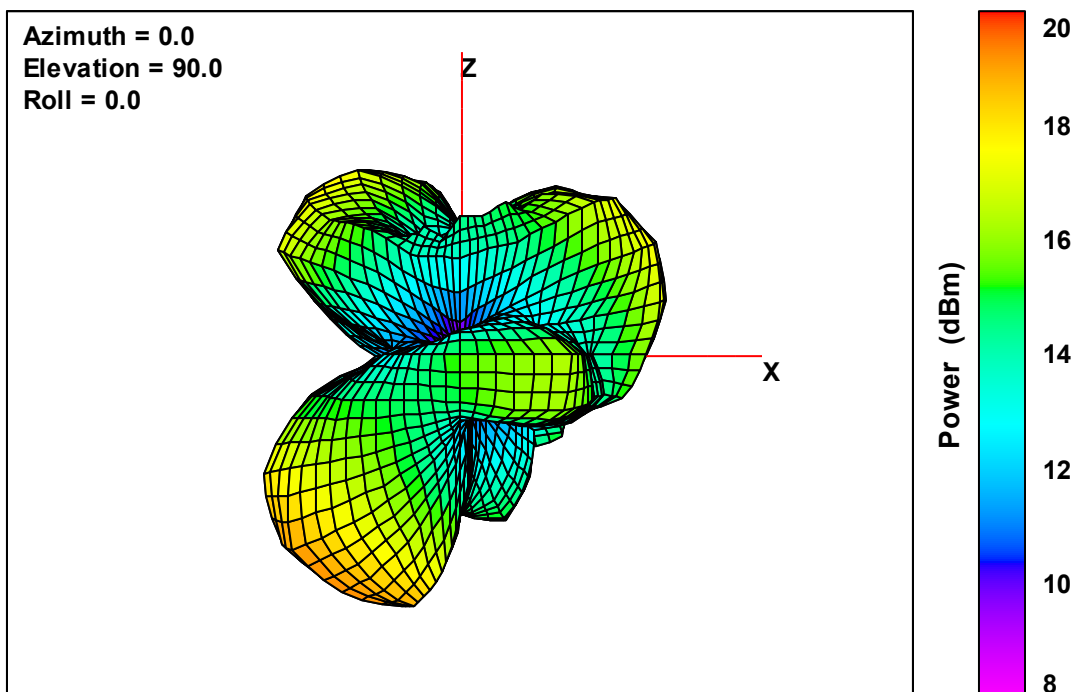
Ant. 2 Free-Space Total EIRP, Left Side View, 5240 MHz
