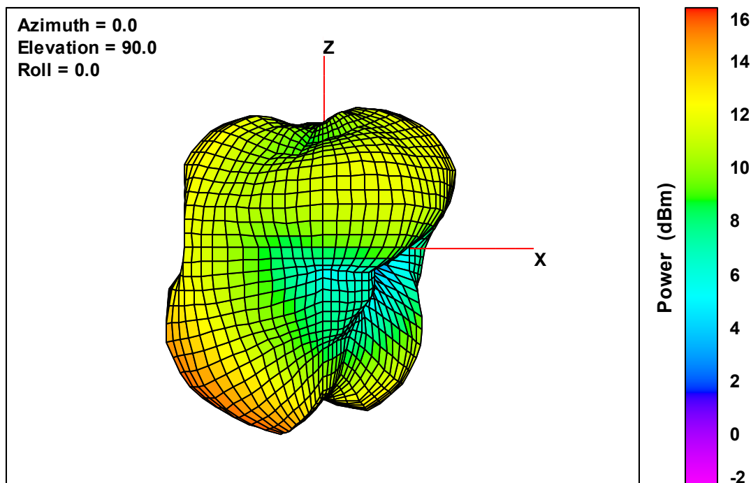
Ant. 2 Free-Space Total EIRP, Left Side View, 5785 MHz
