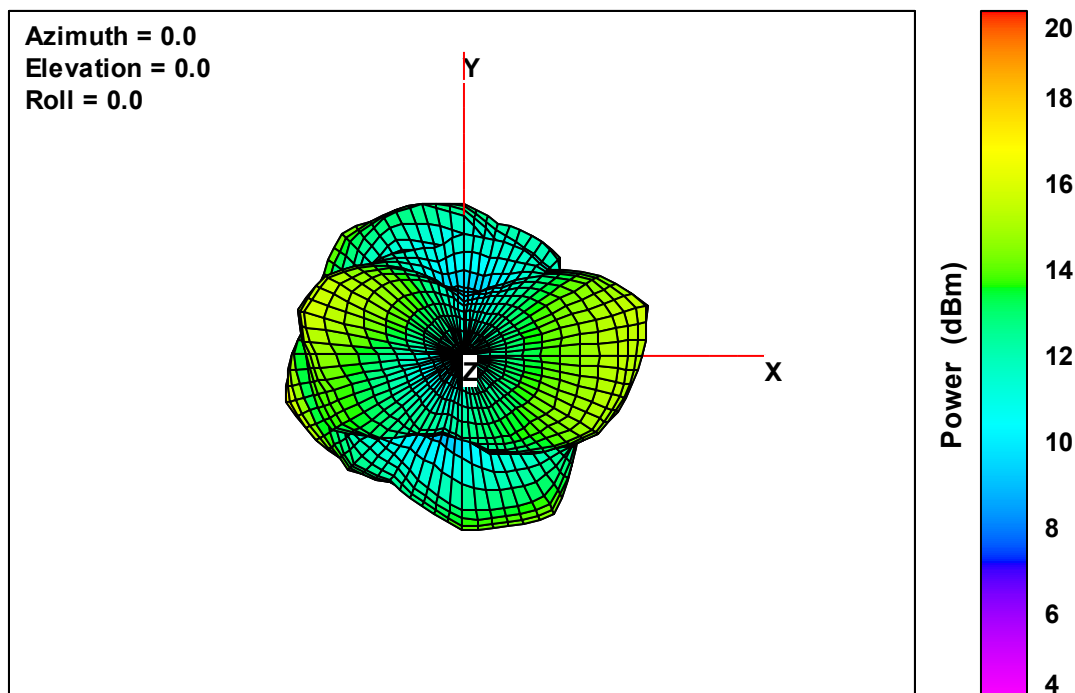
Ant. 2 Free-Space Total EIRP, Top View, 5320 MHz
