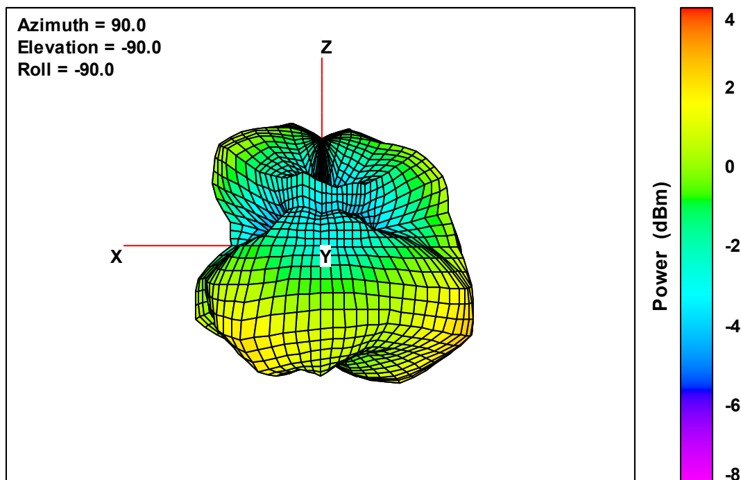
Ant. 3 Free-Space Total EIRP, Right Side View, 2402 MHz
