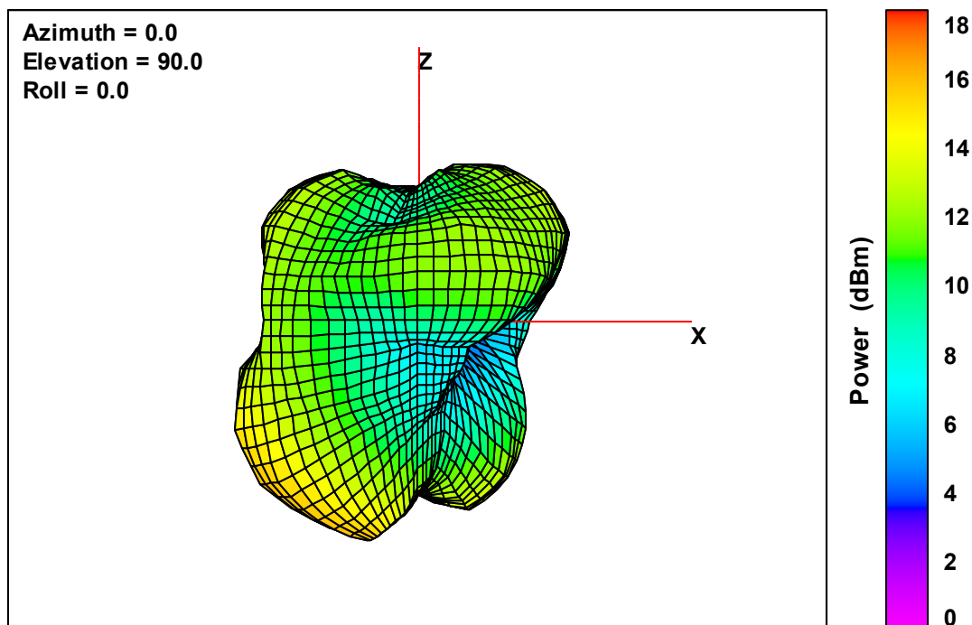
Ant. 2 Free-Space Total EIRP, Left Side View, 5745 MHz
