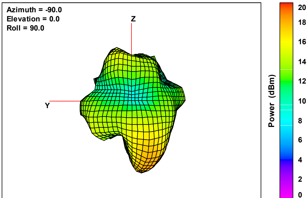
Ant. 2 Free-Space Total EIRP, Back Face View, 5600 MHz
