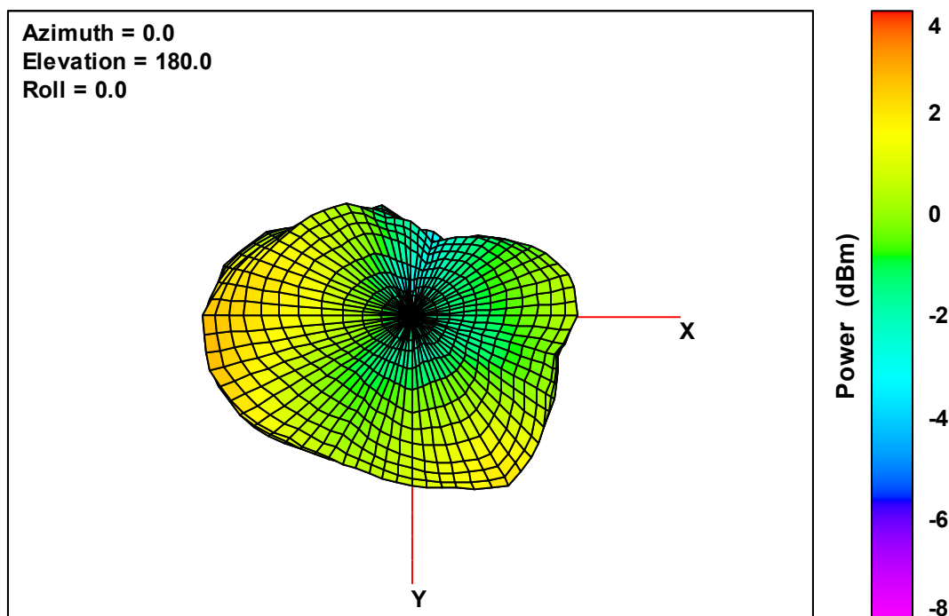
Ant. 3 Free-Space Total EIRP, Bottom View, 2442 MHz
