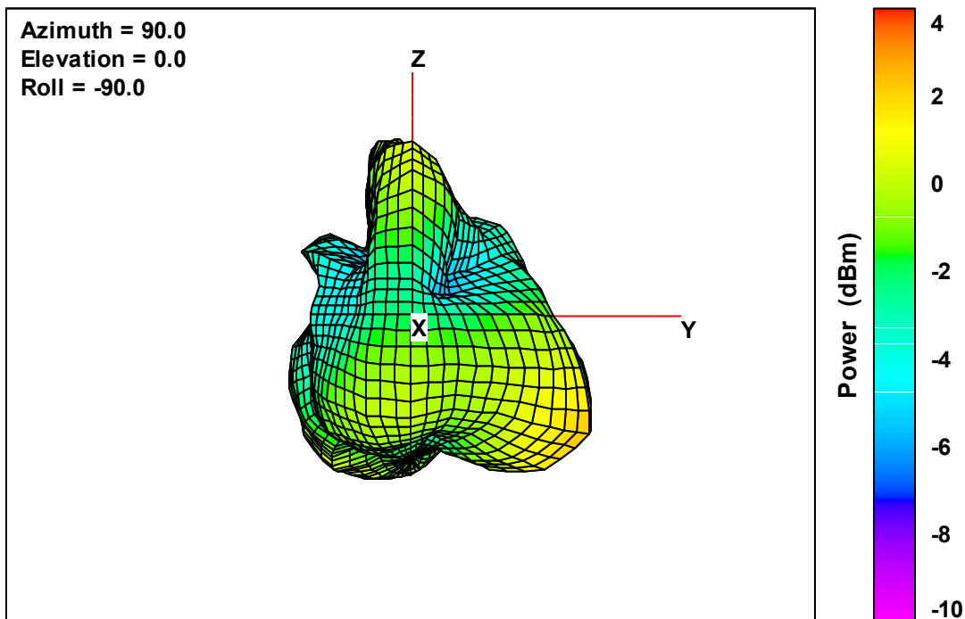
Ant. 3 Free-Space Total EIRP, Front Face View, 2445 MHz
