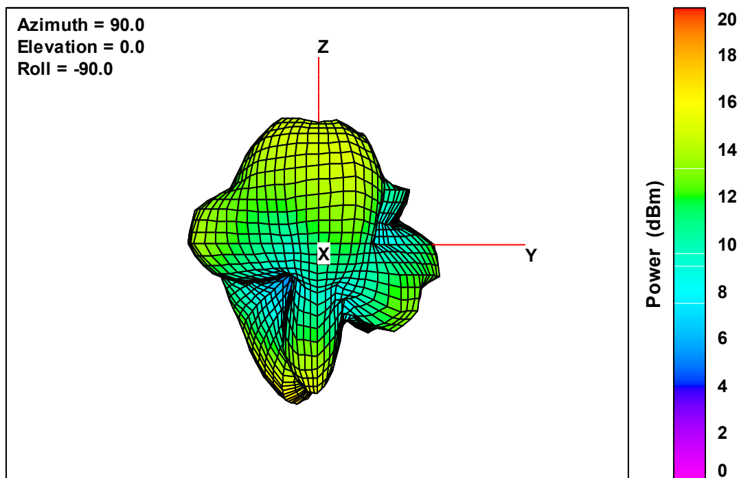
Ant. 2 Free-Space Total EIRP, Front Face View, 5600 MHz
