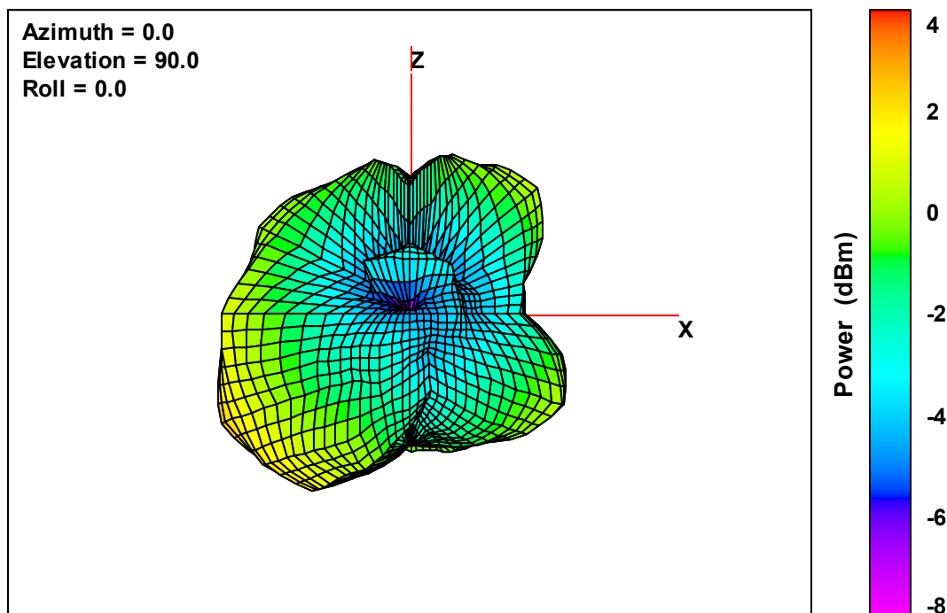
Ant. 3 Free-Space Total EIRP, Left Side View, 2442 MHz
