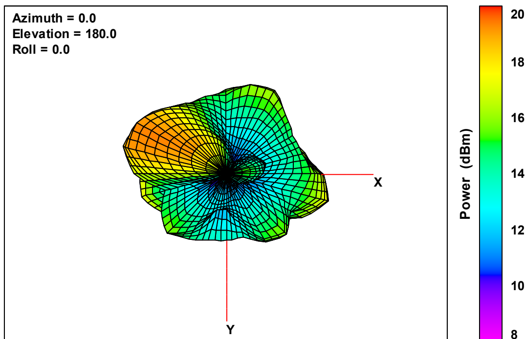
Ant. 2 Free-Space Total EIRP, Bottom View, 5180 MHz
