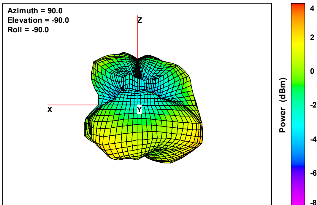
Ant. 3 Free-Space Total EIRP, Right Side View, 2405 MHz
