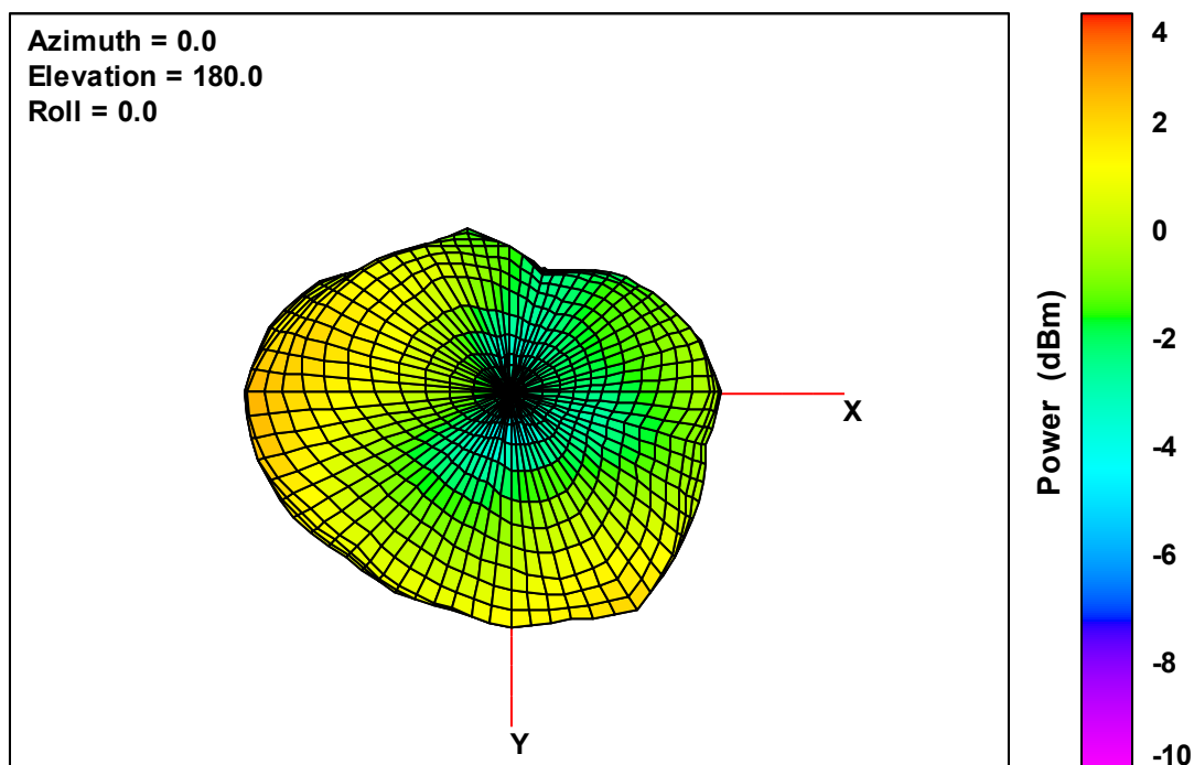
Ant. 3 Free-Space Total EIRP, Bottom View, 2480 MHz
