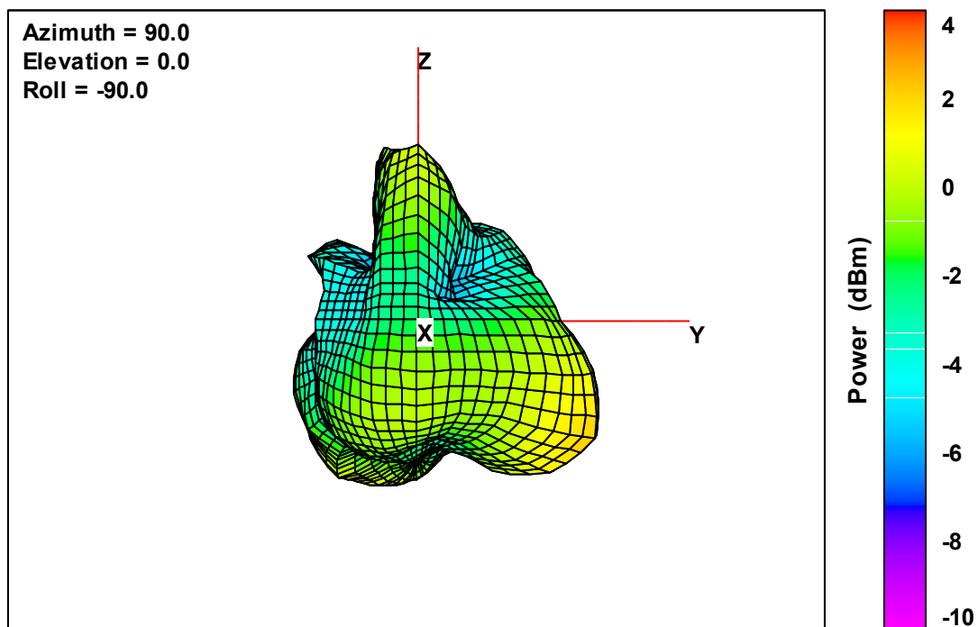
Ant. 3 Free-Space Total EIRP, Front Face View, 2475 MHz
