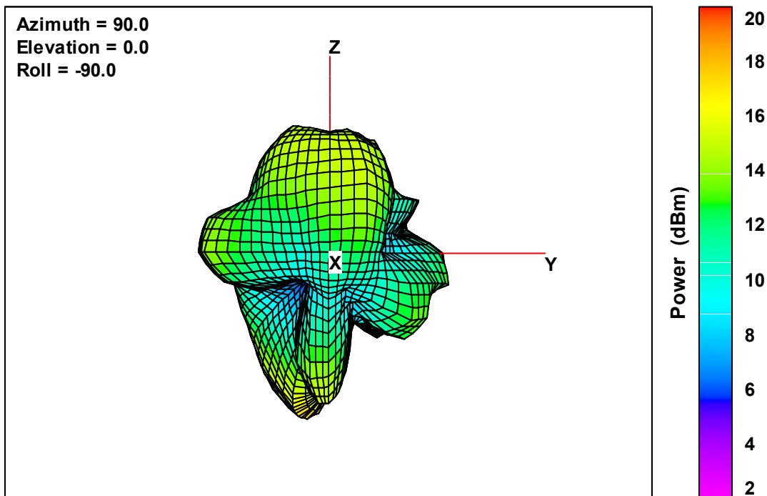
Ant. 2 Free-Space Total EIRP, Front Face View, 5500 MHz
