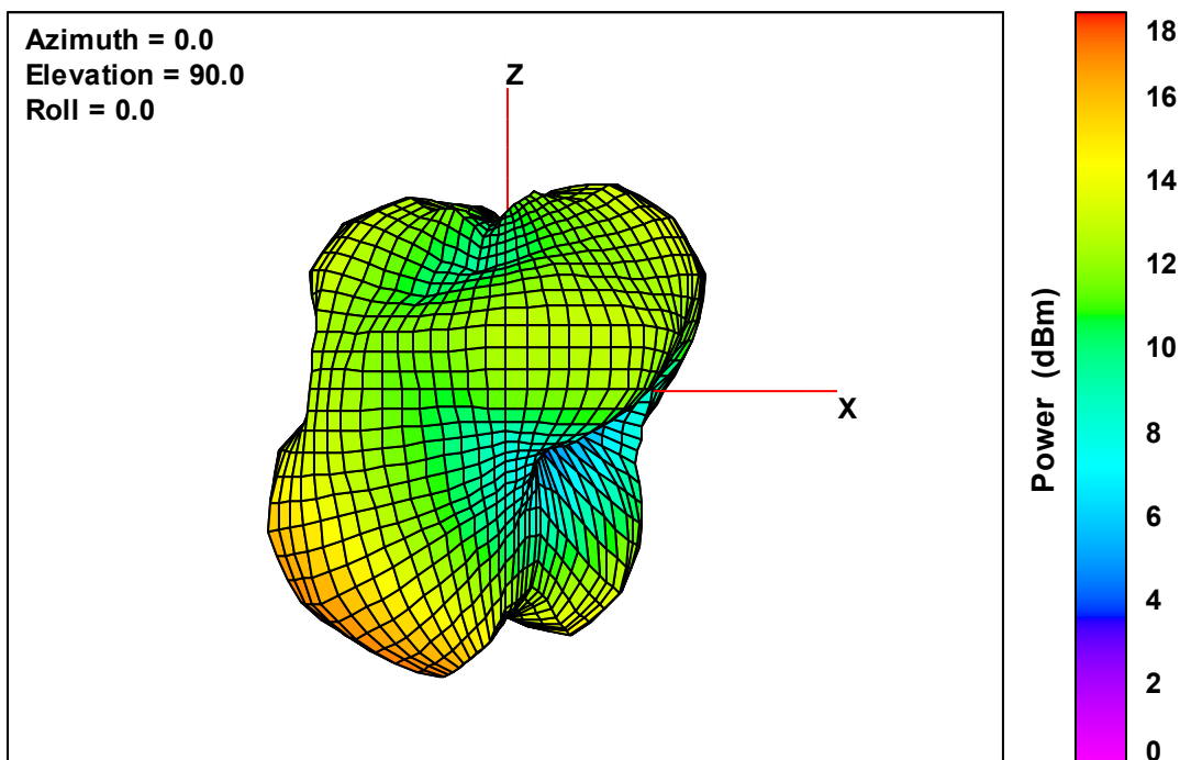
Ant. 2 Free-Space Total EIRP, Left Side View, 5700 MHz
