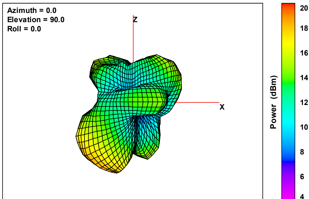
Ant. 2 Free-Space Total EIRP, Left Side View, 5320 MHz
