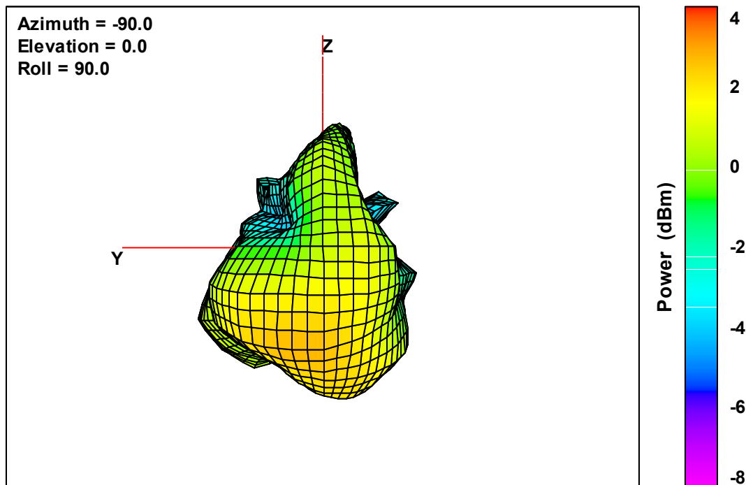
Ant. 3 Free-Space Total EIRP, Back Face View, 2402 MHz
