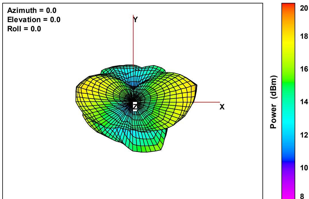
Ant. 2 Free-Space Total EIRP, Top View, 5240 MHz
