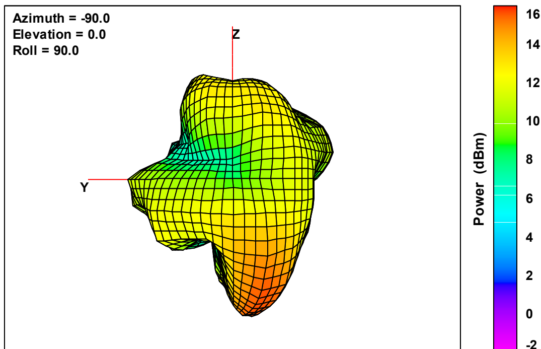
Ant. 2 Free-Space Total EIRP, Back Face View, 5785 MHz
