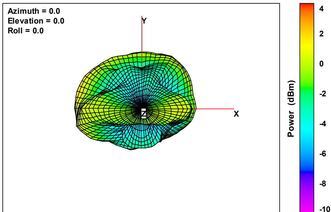
Ant. 3 Free-Space Total EIRP, Top View, 2445 MHz
