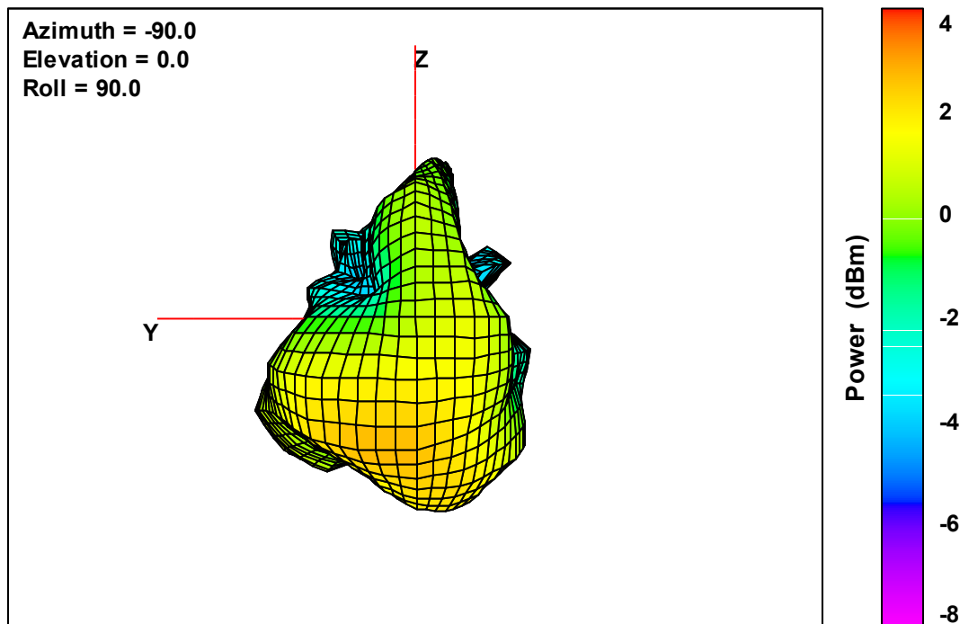
Ant. 3 Free-Space Total EIRP, Back Face View, 2405 MHz
