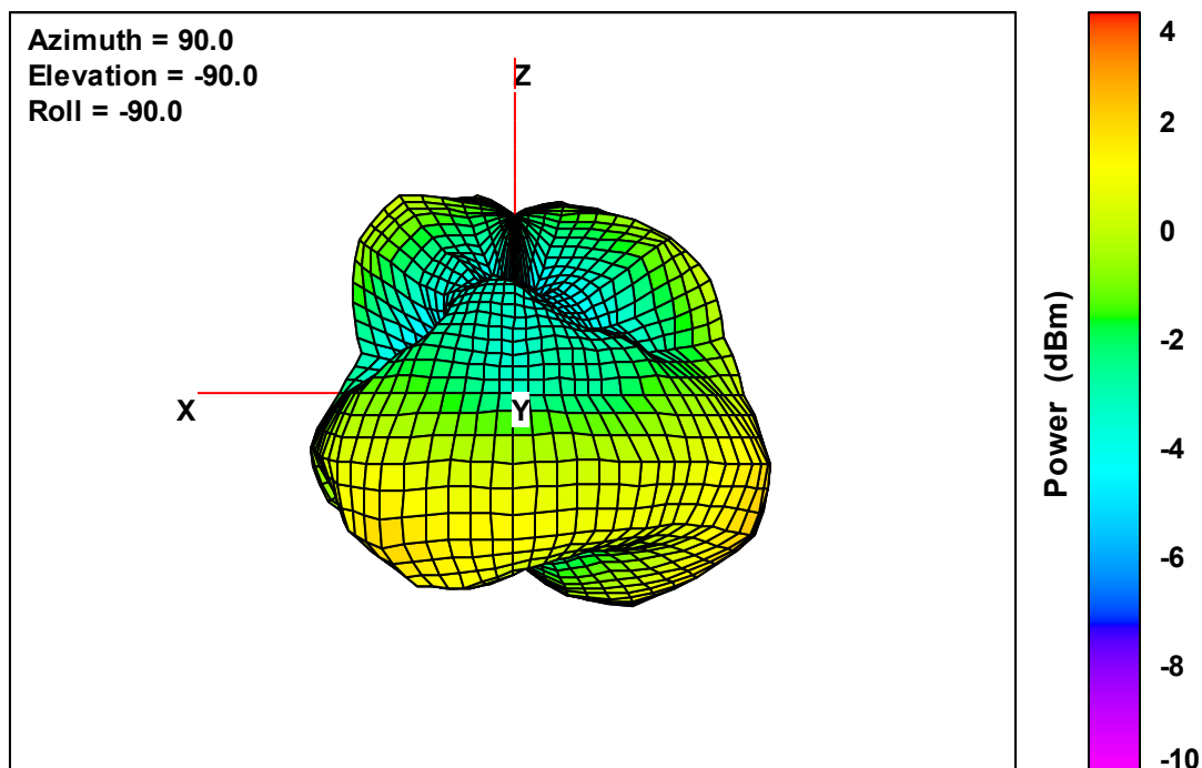
Ant. 3 Free-Space Total EIRP, Right Side View, 2480 MHz
