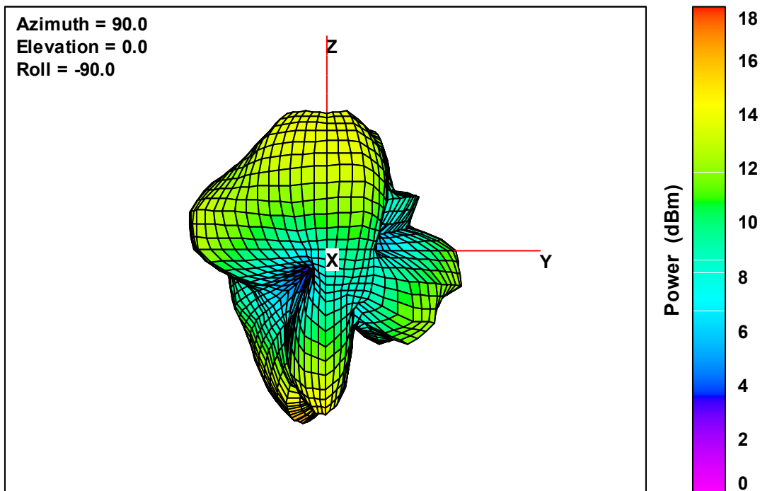
Ant. 2 Free-Space Total EIRP, Front Face View, 5700 MHz
