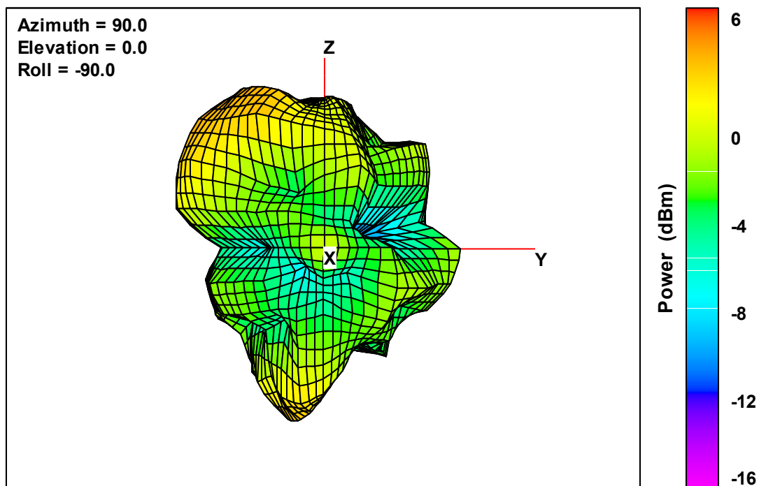
Ant. 2 Free-Space Total EIRP, Front Face View, 5825 MHz
