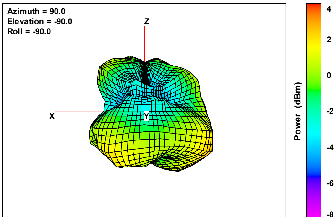
Ant. 3 Free-Space Total EIRP, Right Side View, 2442 MHz
