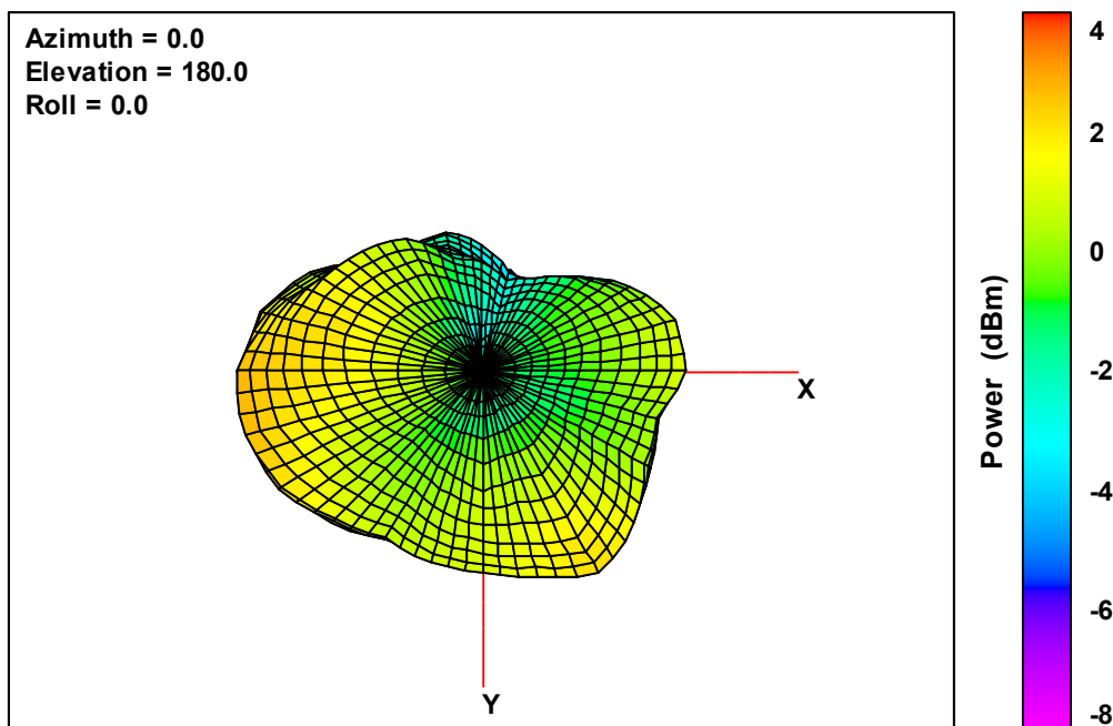
Ant. 3 Free-Space Total EIRP, Bottom View, 2402 MHz
