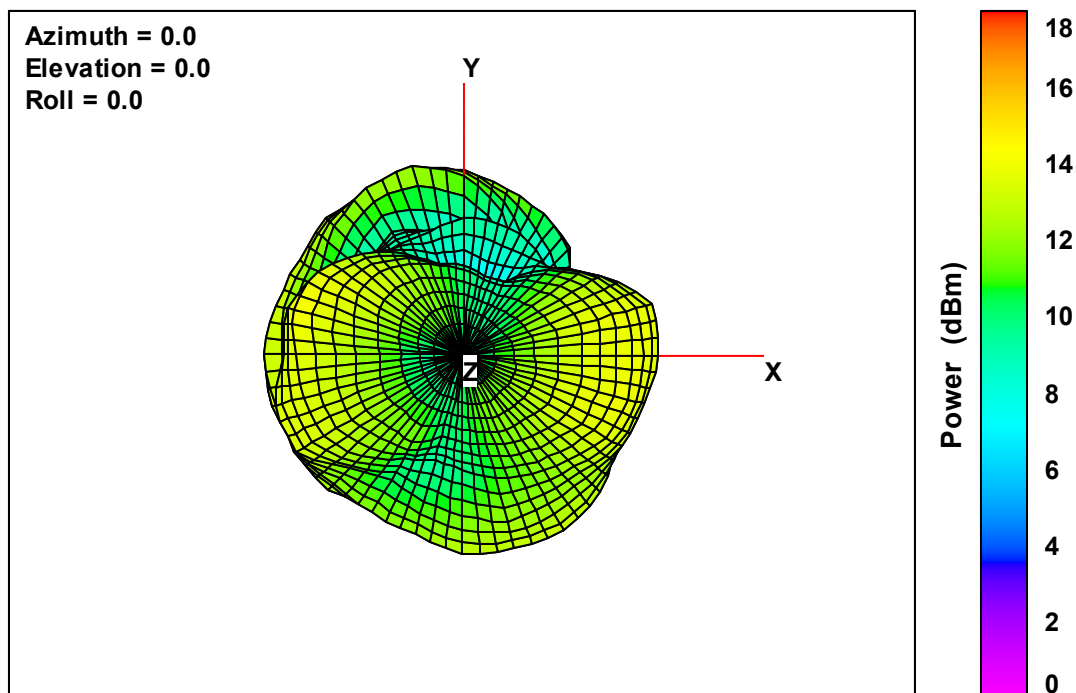
Ant. 2 Free-Space Total EIRP, Top View, 5700 MHz
