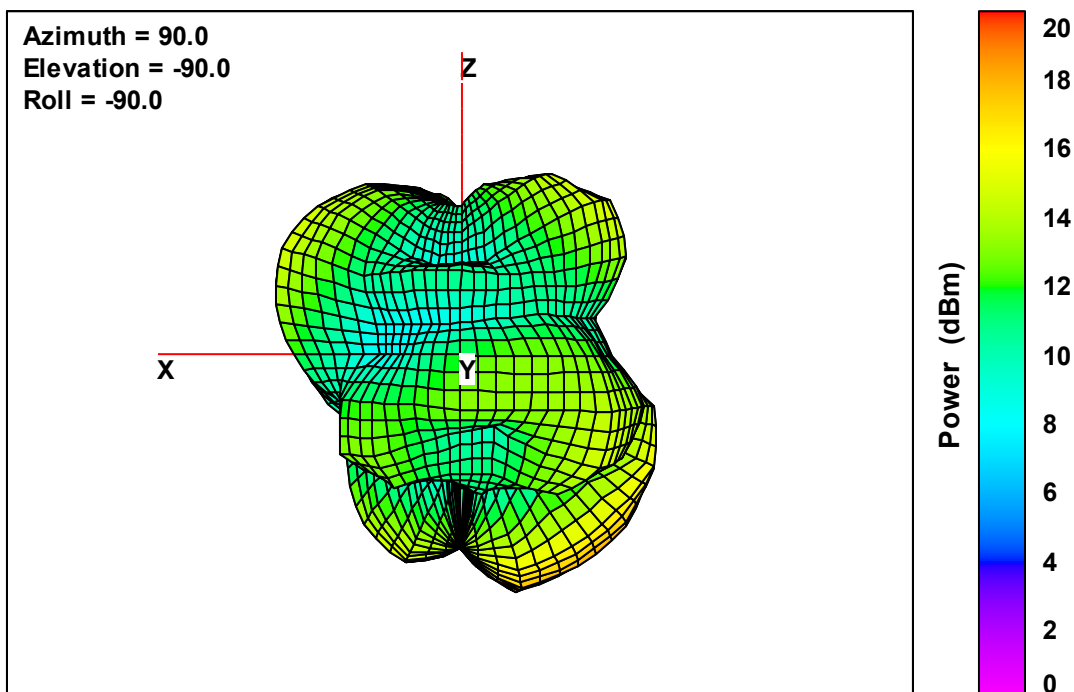
Ant. 2 Free-Space Total EIRP, Right Side View, 5600 MHz
