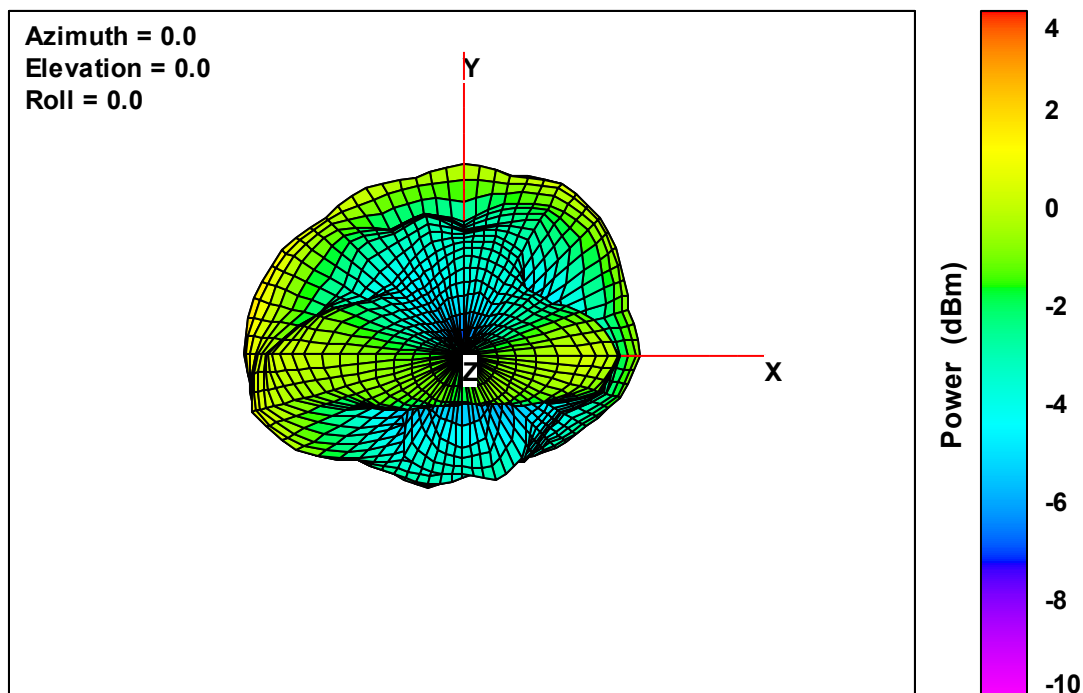
Ant. 3 Free-Space Total EIRP, Top View, 2480 MHz
