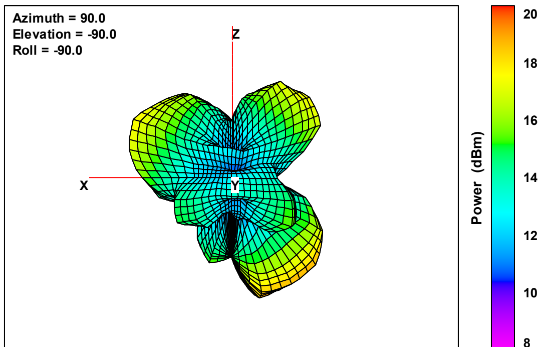
Ant. 2 Free-Space Total EIRP, Right Side View, 5260 MHz
