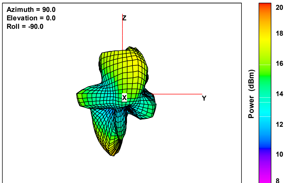
Ant. 2 Free-Space Total EIRP, Front Face View, 5260 MHz
