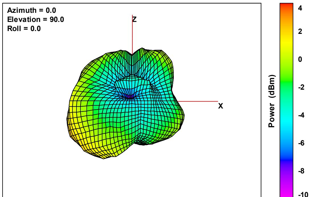
Ant. 3 Free-Space Total EIRP, Left Side View, 2480 MHz
