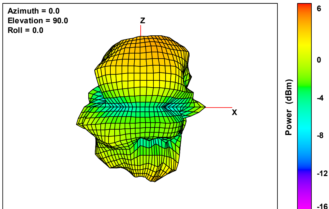
Ant. 2 Free-Space Total EIRP, Left Side View, 5825 MHz
