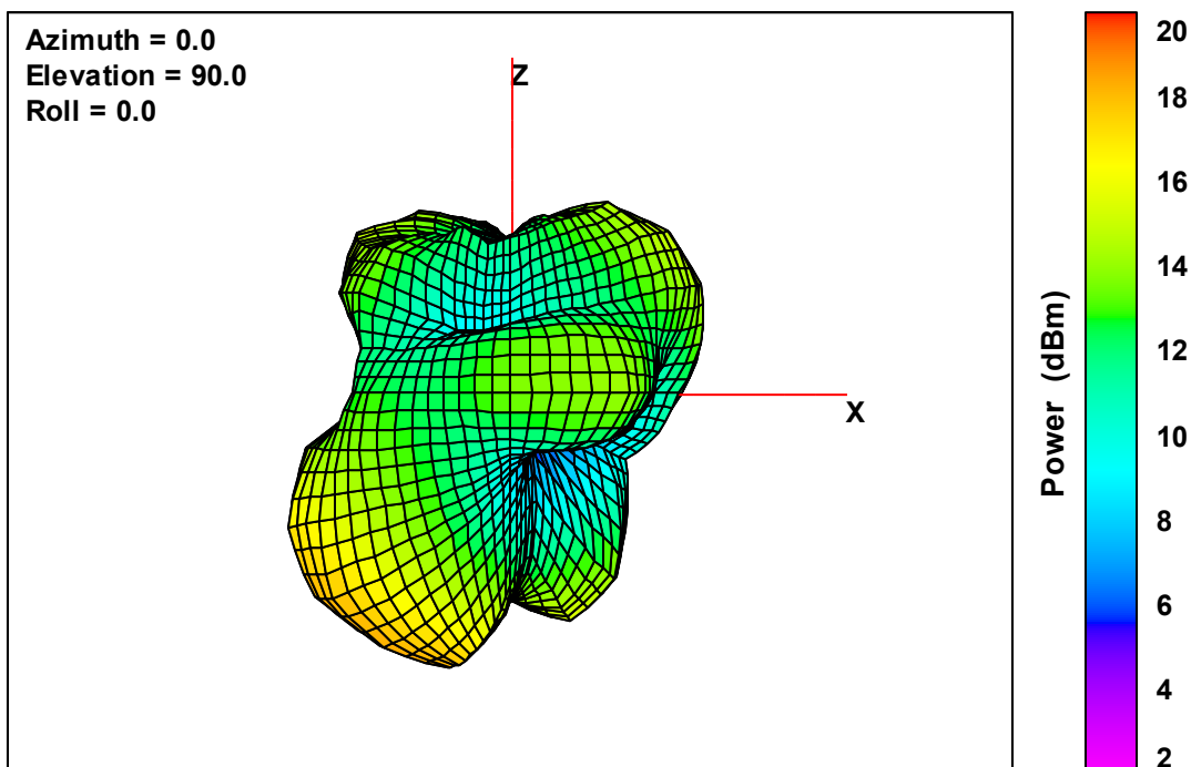
Ant. 2 Free-Space Total EIRP, Left Side View, 5500 MHz
