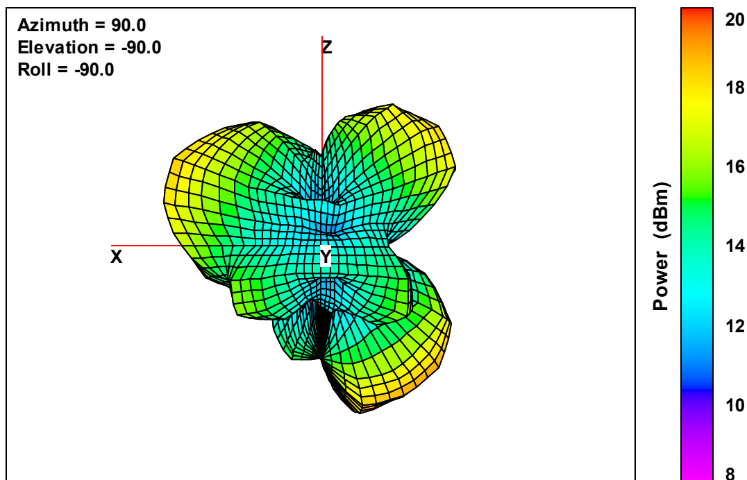
Ant. 2 Free-Space Total EIRP, Right Side View, 5180 MHz
