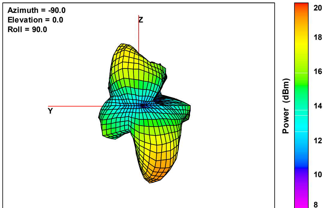
Ant. 2 Free-Space Total EIRP, Back Face View, 5240 MHz
