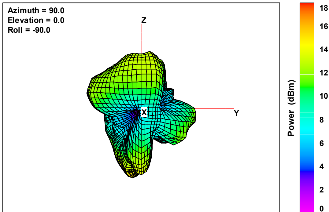
Ant. 2 Free-Space Total EIRP, Front Face View, 5745 MHz
