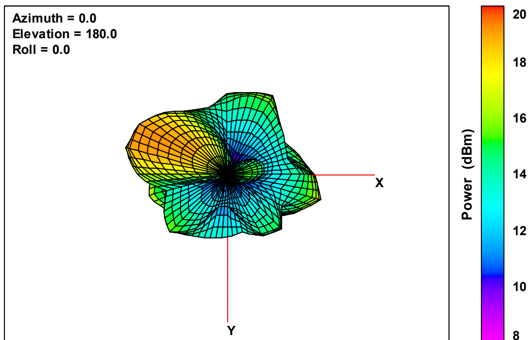
Ant. 2 Free-Space Total EIRP, Bottom View, 5260 MHz
