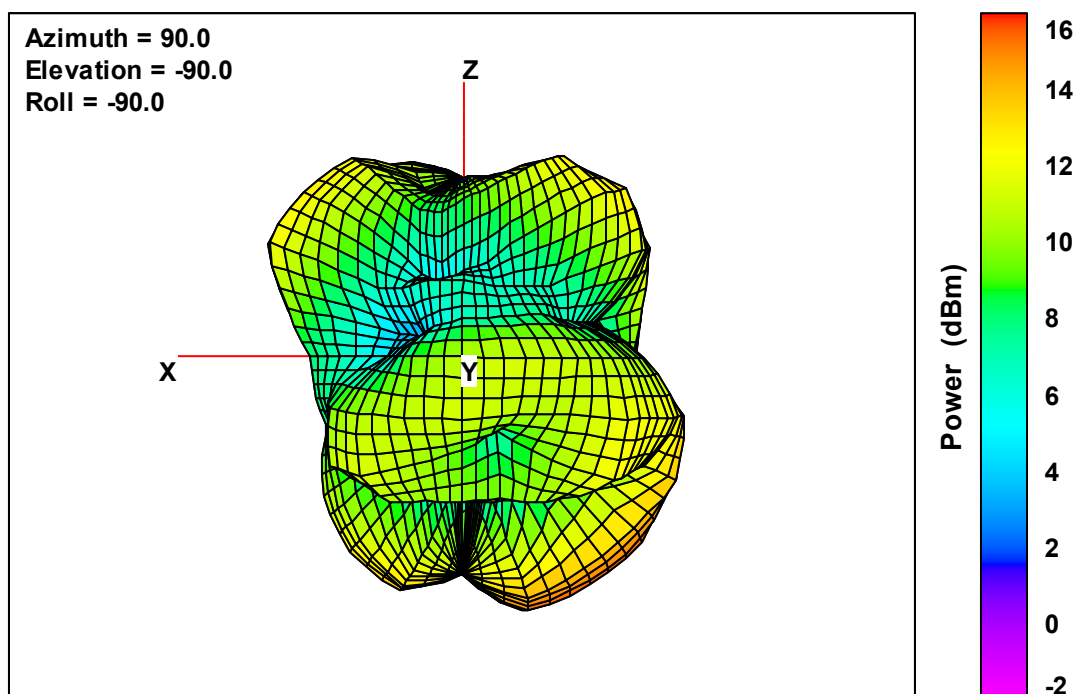
Ant. 2 Free-Space Total EIRP, Right Side View, 5785 MHz
