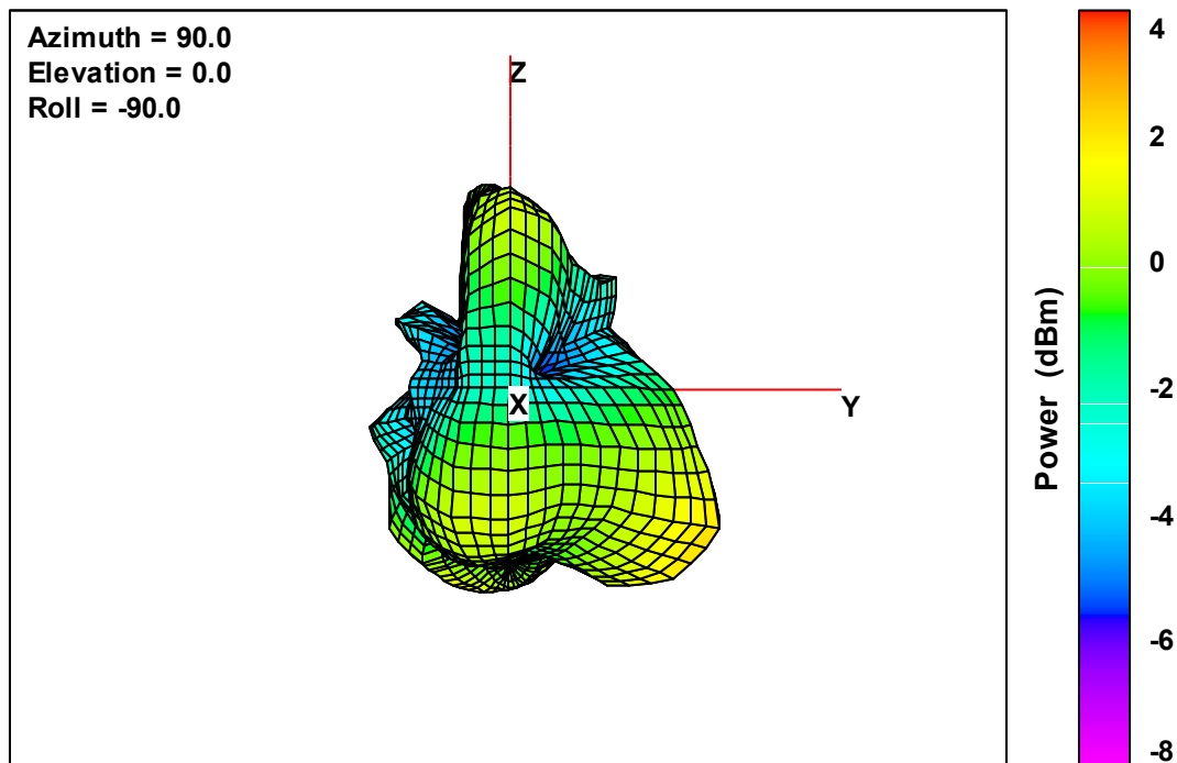
Ant. 3 Free-Space Total EIRP, Front Face View, 2402 MHz
