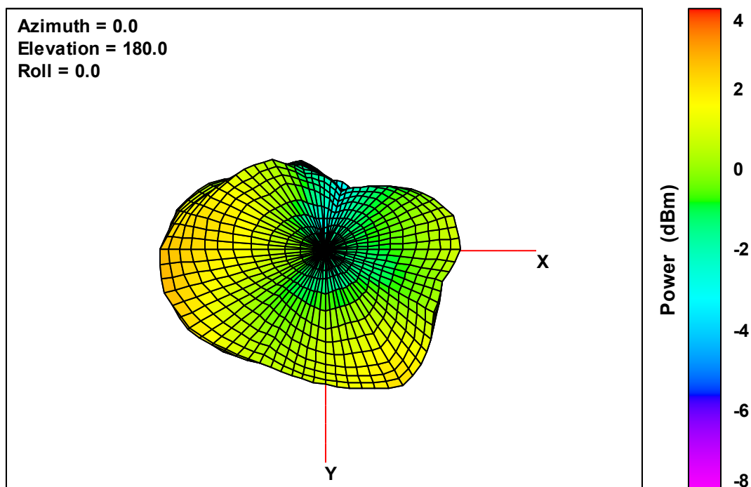
Ant. 3 Free-Space Total EIRP, Bottom View, 2405 MHz
