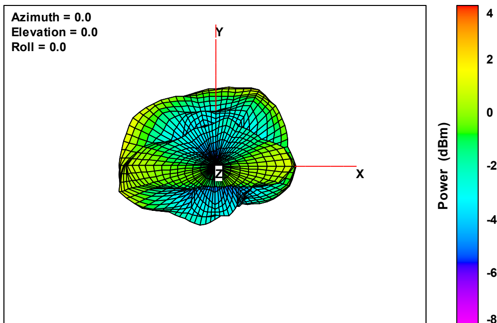
Ant. 3 Free-Space Total EIRP, Top View, 2402 MHz
