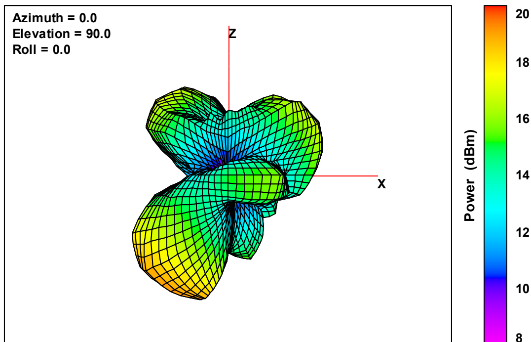
Ant. 2 Free-Space Total EIRP, Left Side View, 5260 MHz
