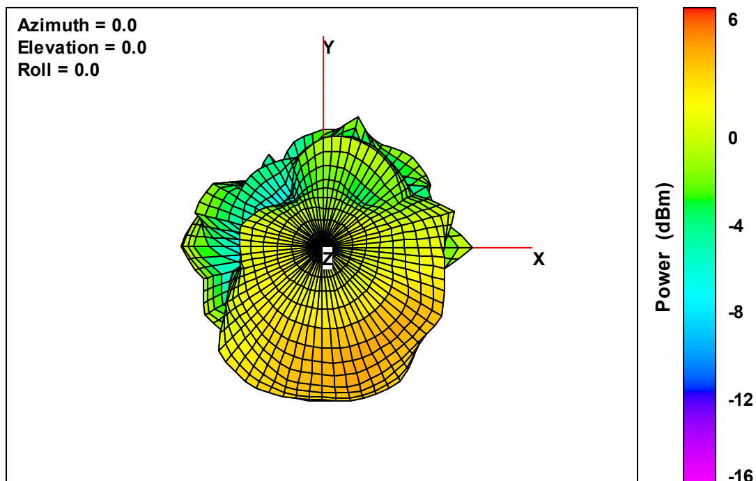
Ant. 2 Free-Space Total EIRP, Top View, 5825 MHz
