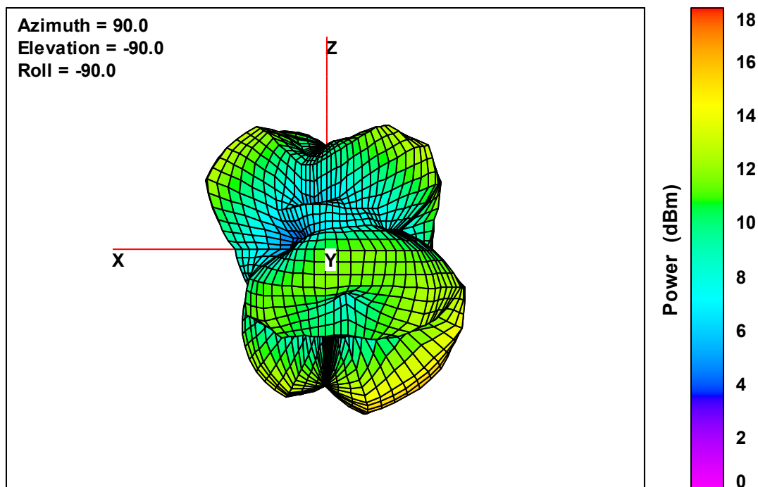
Ant. 2 Free-Space Total EIRP, Right Side View, 5745 MHz
