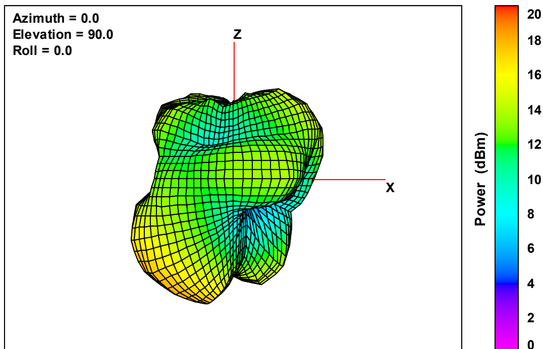
Ant. 2 Free-Space Total EIRP, Left Side View, 5600 MHz
