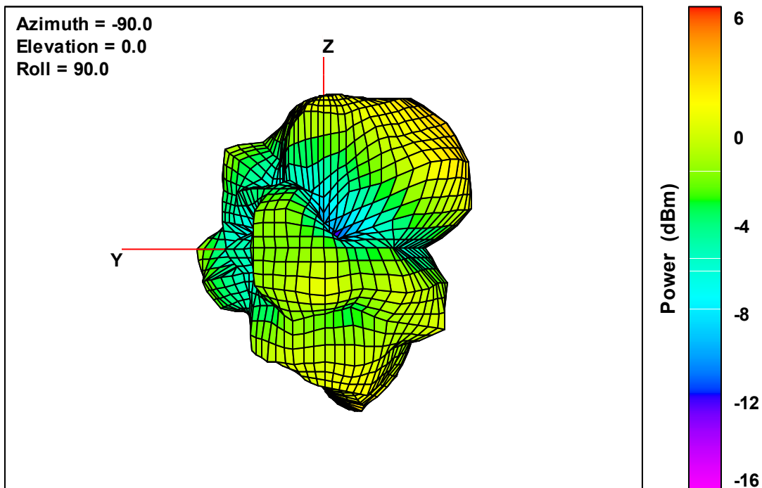
Ant. 2 Free-Space Total EIRP, Back Face View, 5825 MHz
