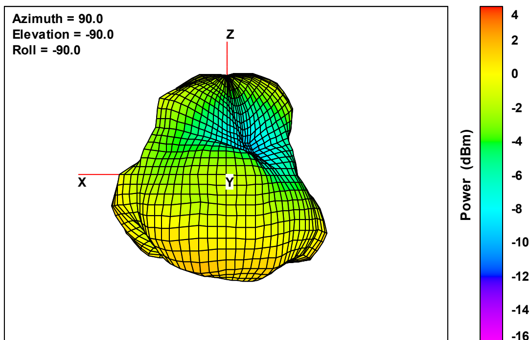
Ant. 4 Free-Space Total EIRP, Right Side View, 2475 MHz
