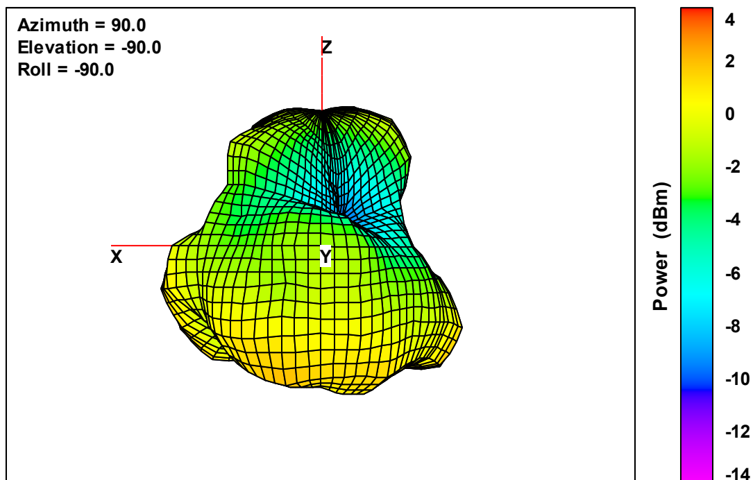
Ant. 4 Free-Space Total EIRP, Right Side View, 2445 MHz
