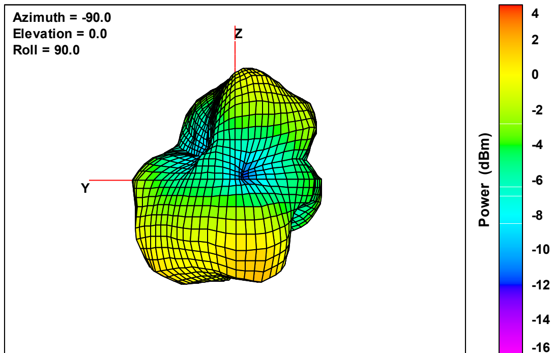
Ant. 4 Free-Space Total EIRP, Back Face View, 2480 MHz
