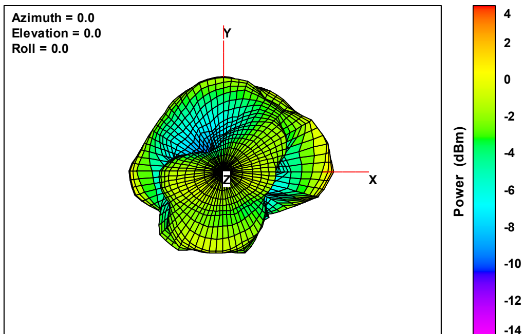
Ant. 4 Free-Space Total EIRP, Top View, 2402 MHz
