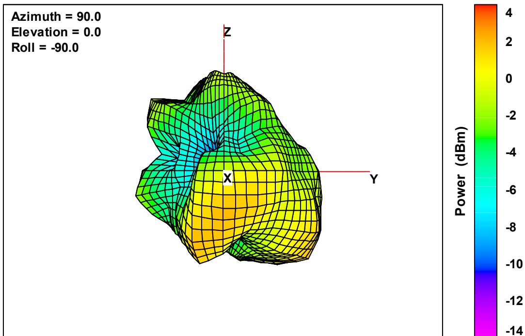
Ant. 4 Free-Space Total EIRP, Front Face View, 2402 MHz
