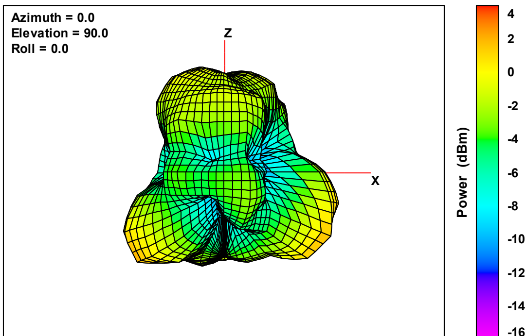
Ant. 4 Free-Space Total EIRP, Left Side View, 2475 MHz
