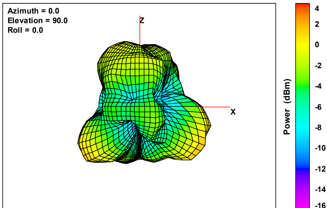
Ant. 4 Free-Space Total EIRP, Left Side View, 2480 MHz
