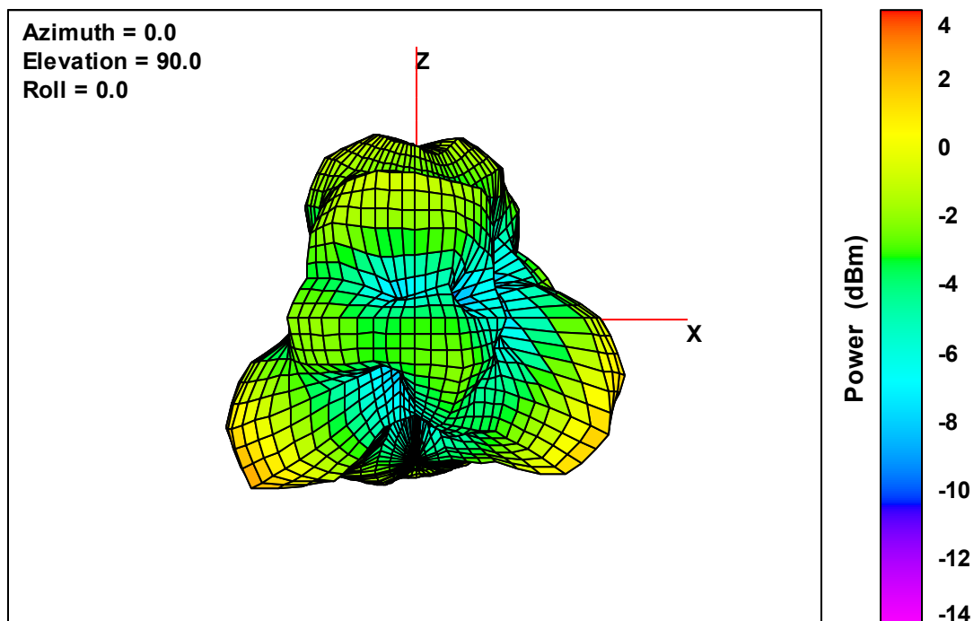
Ant. 4 Free-Space Total EIRP, Left Side View, 2405 MHz
