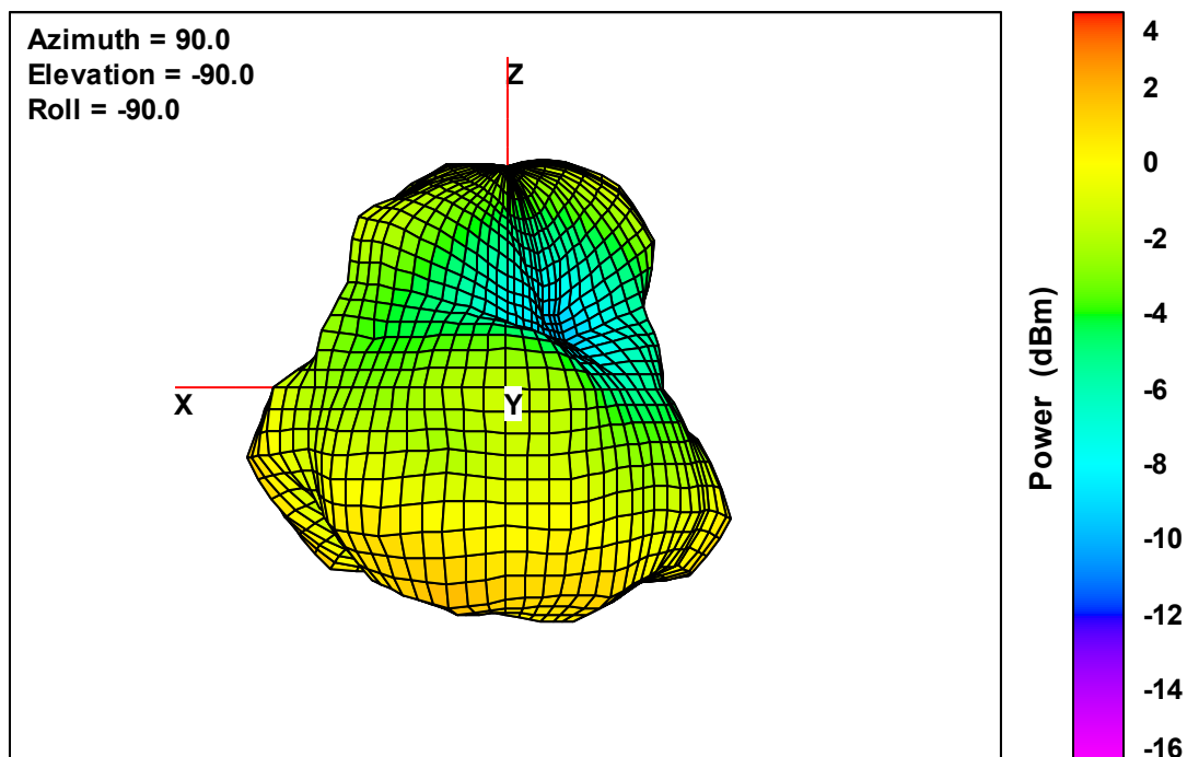
Ant. 4 Free-Space Total EIRP, Right Side View, 2480 MHz
