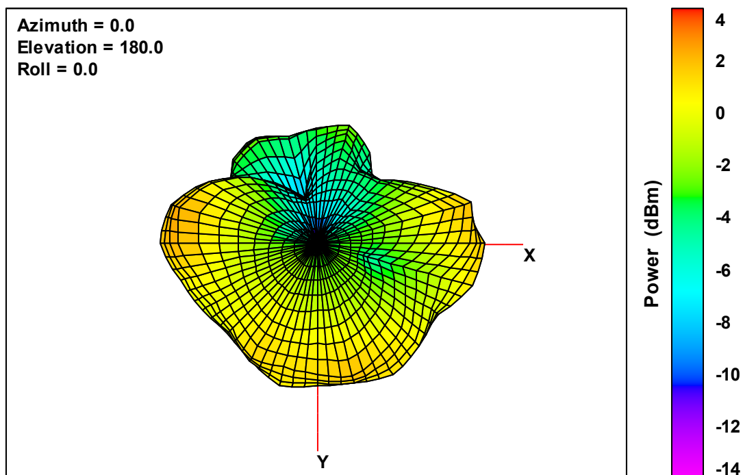
Ant. 4 Free-Space Total EIRP, Bottom View, 2442 MHz
