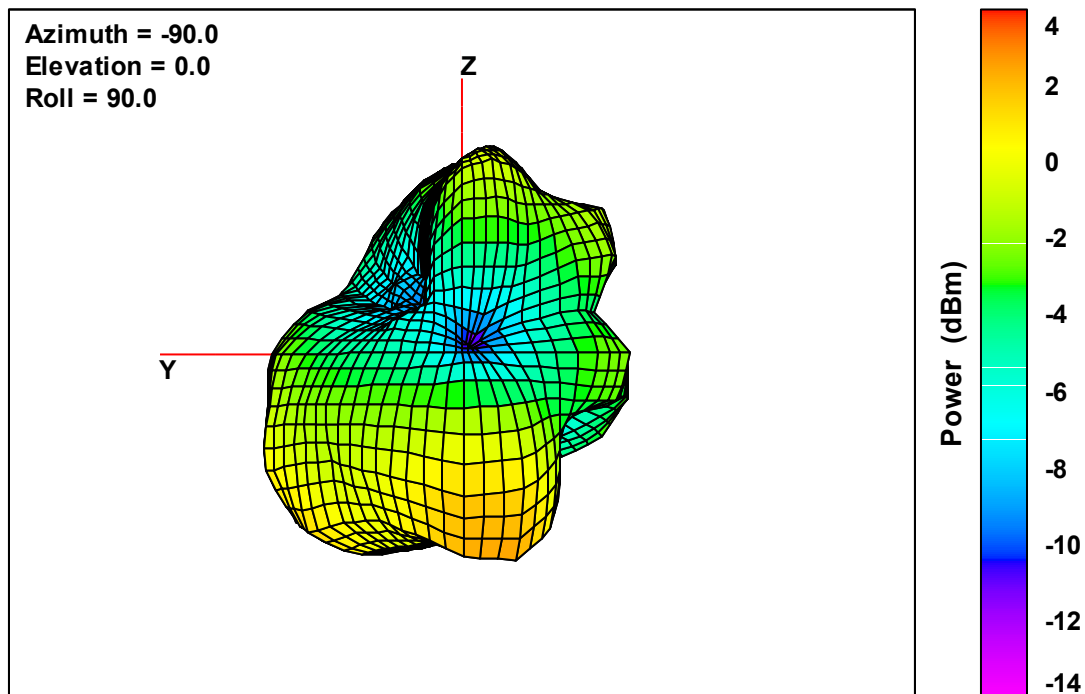
Ant. 4 Free-Space Total EIRP, Back Face View, 2442 MHz
