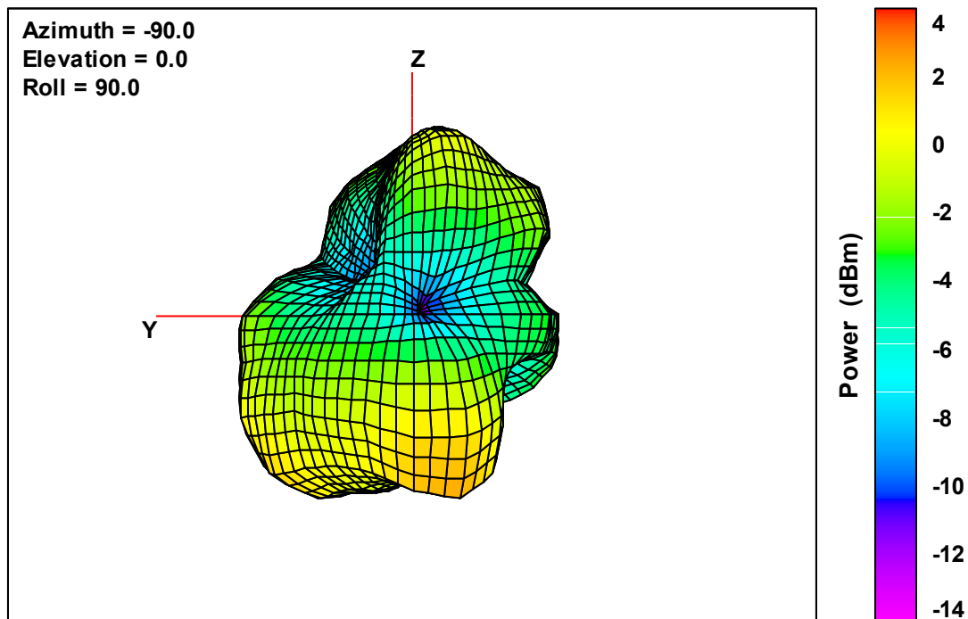
Ant. 4 Free-Space Total EIRP, Back Face View, 2445 MHz
