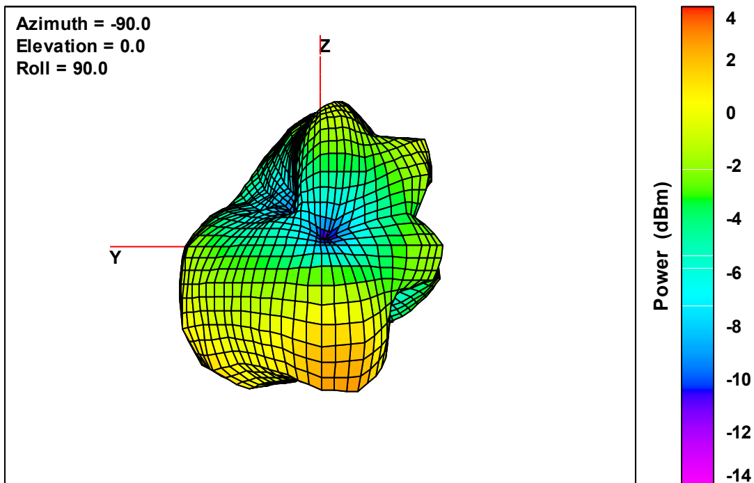
Ant. 4 Free-Space Total EIRP, Back Face View, 2402 MHz
