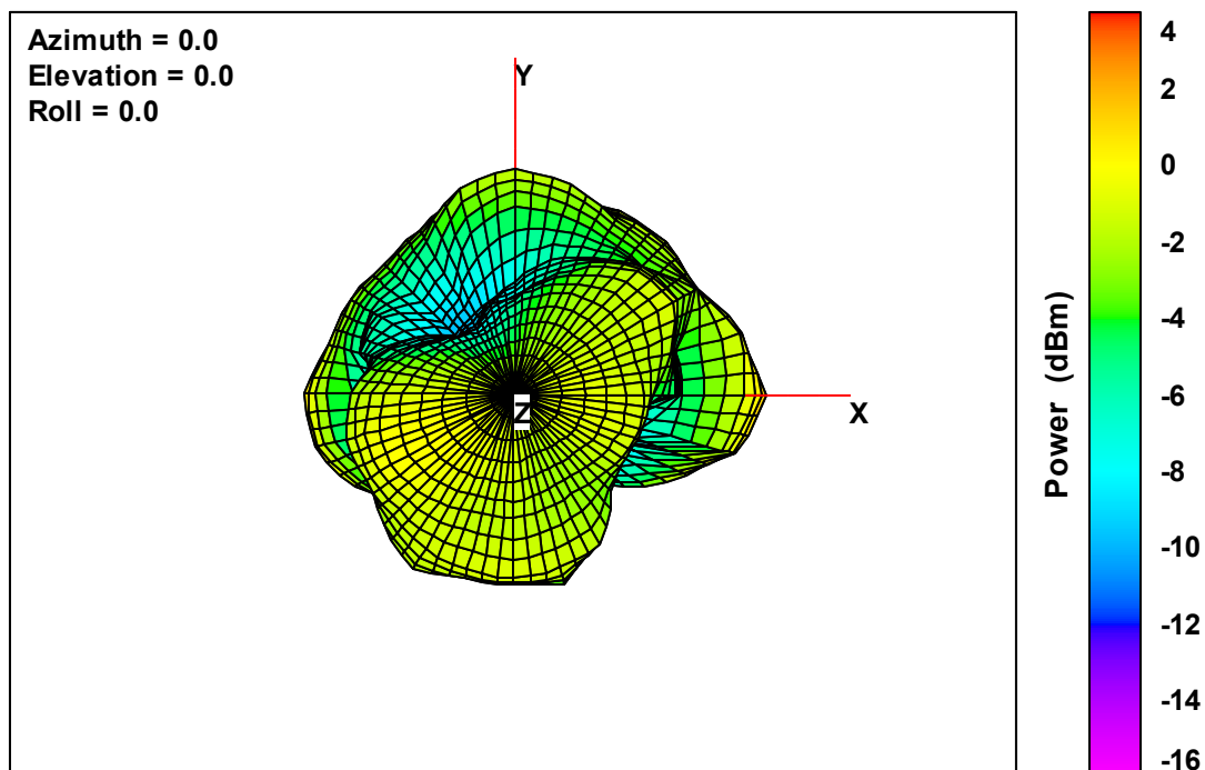
Ant. 4 Free-Space Total EIRP, Top View, 2480 MHz
