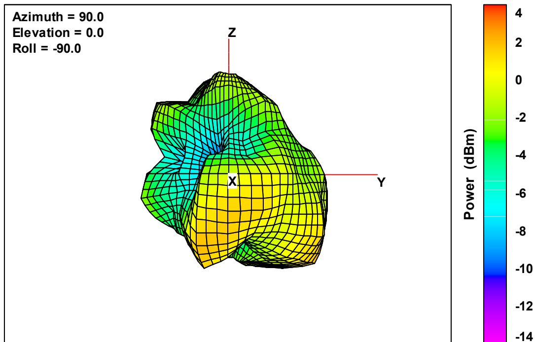
Ant. 4 Free-Space Total EIRP, Front Face View, 2405 MHz
