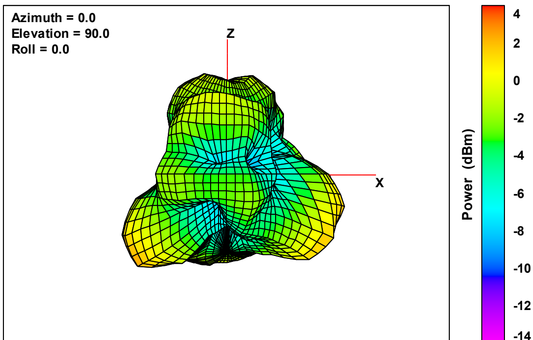
Ant. 4 Free-Space Total EIRP, Left Side View, 2402 MHz
