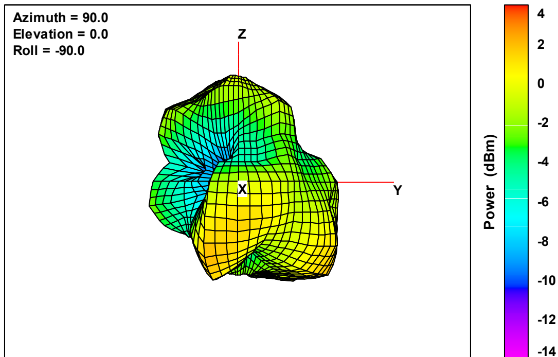
Ant. 4 Free-Space Total EIRP, Front Face View, 2445 MHz
