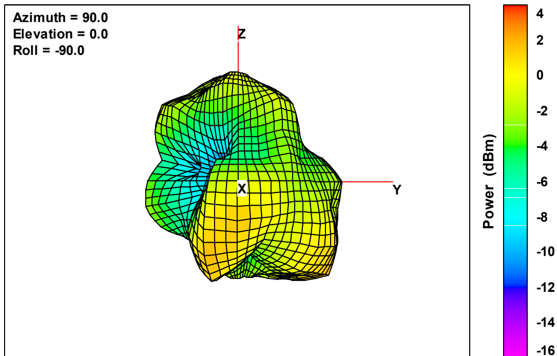
Ant. 4 Free-Space Total EIRP, Front Face View, 2480 MHz
