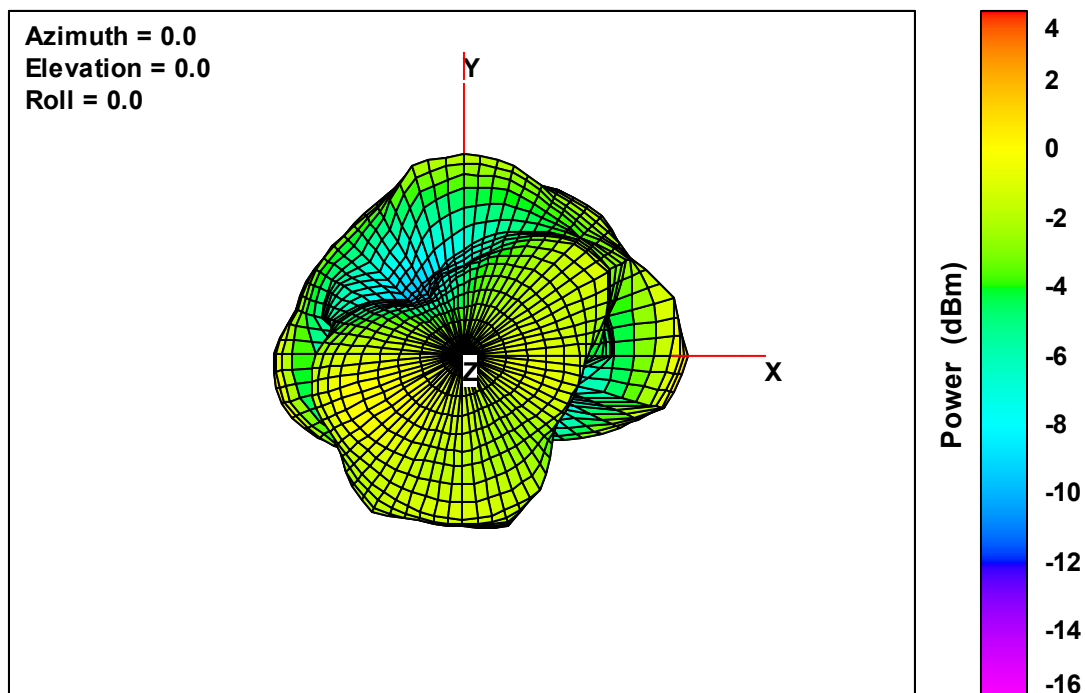
Ant. 4 Free-Space Total EIRP, Top View, 2475 MHz
