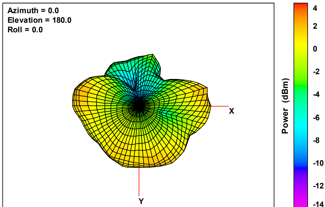
Ant. 4 Free-Space Total EIRP, Bottom View, 2445 MHz
