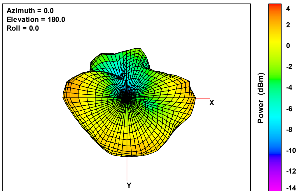
Ant. 4 Free-Space Total EIRP, Bottom View, 2402 MHz
