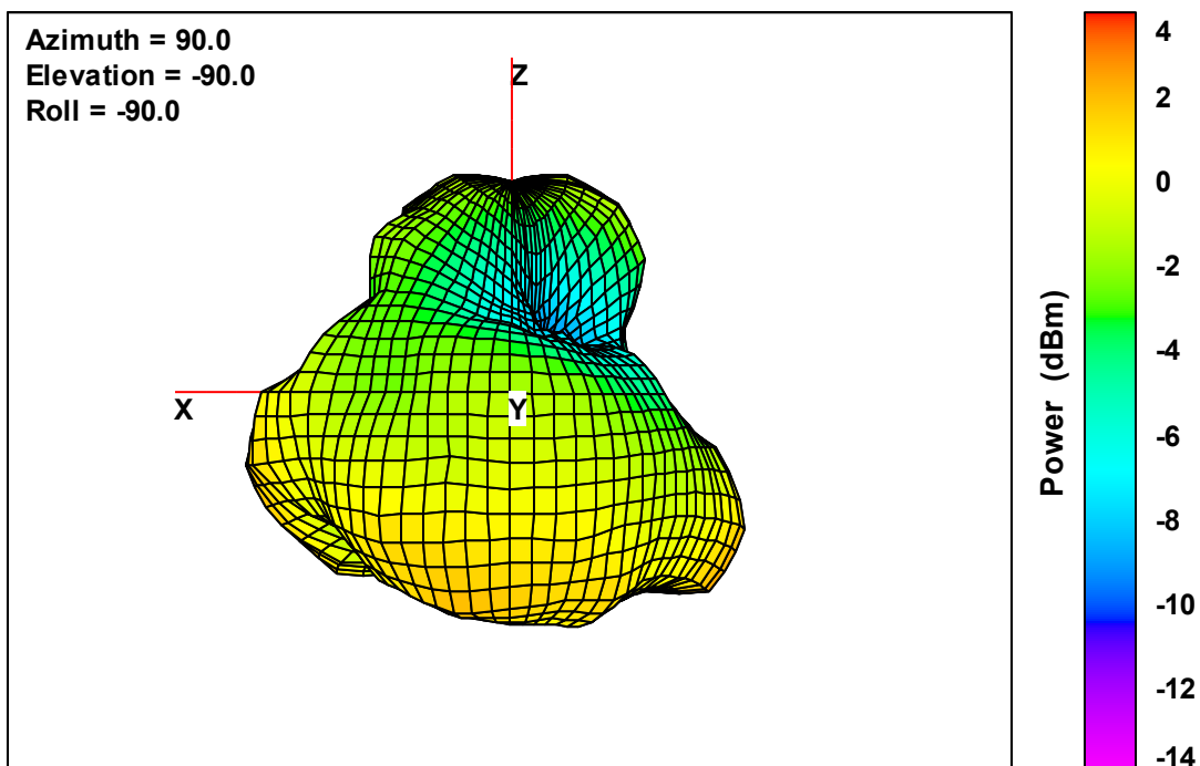
Ant. 4 Free-Space Total EIRP, Right Side View, 2402 MHz
