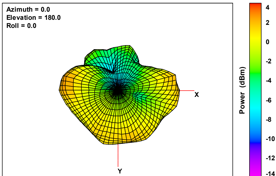
Ant. 4 Free-Space Total EIRP, Bottom View, 2405 MHz
