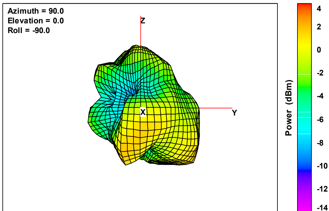
Ant. 4 Free-Space Total EIRP, Front Face View, 2442 MHz
