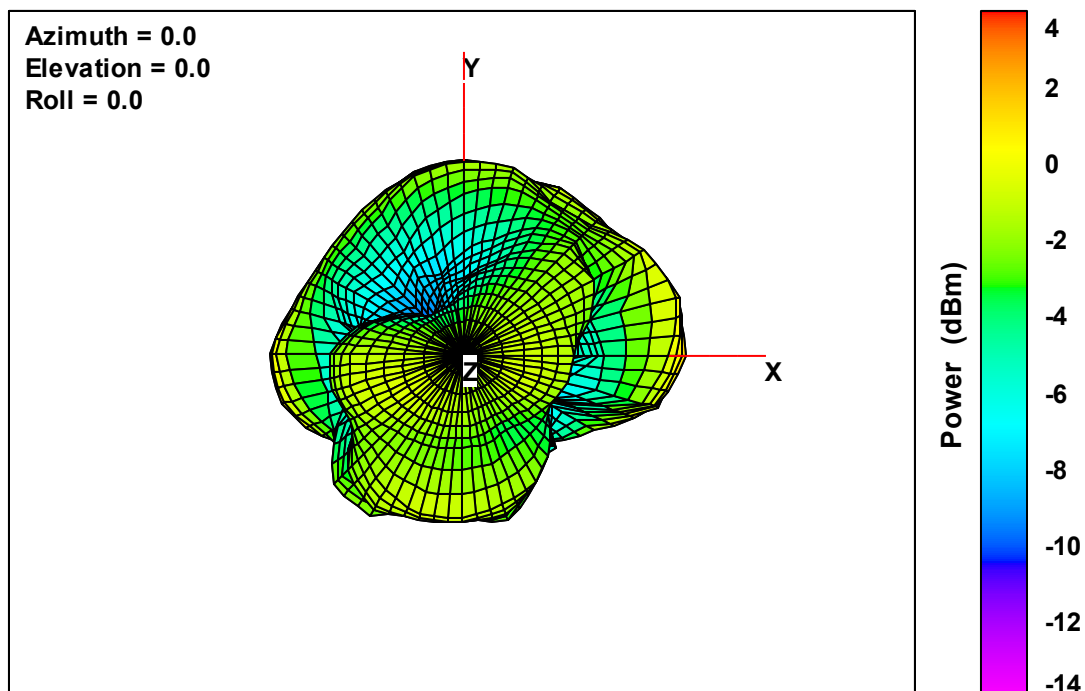
Ant. 4 Free-Space Total EIRP, Top View, 2405 MHz
