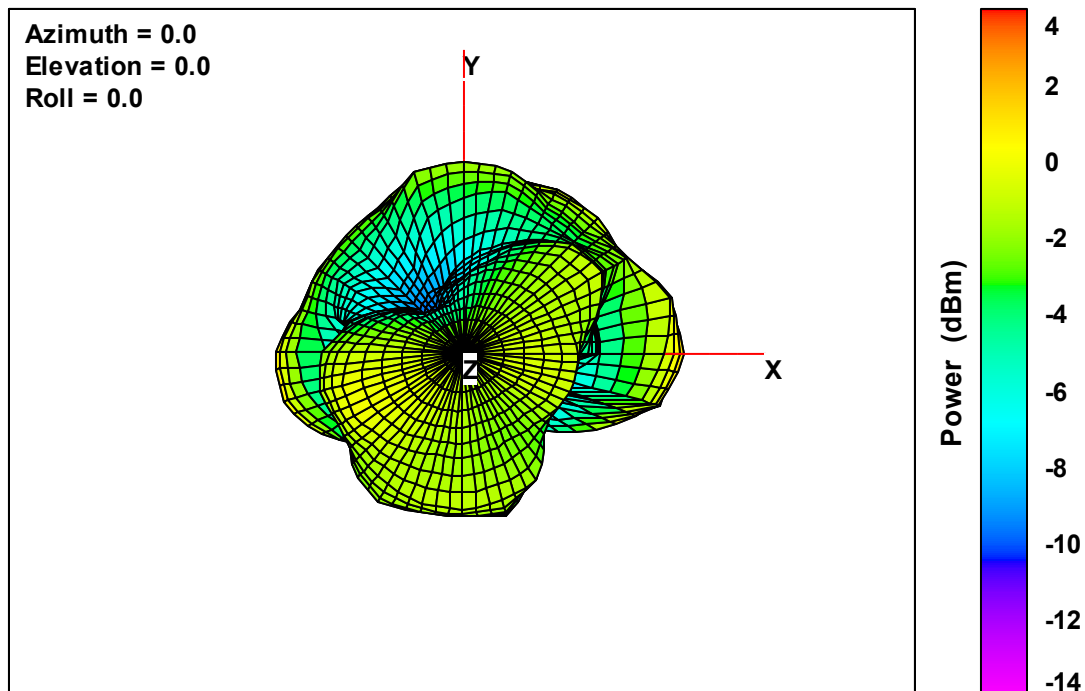
Ant. 4 Free-Space Total EIRP, Top View, 2445 MHz
