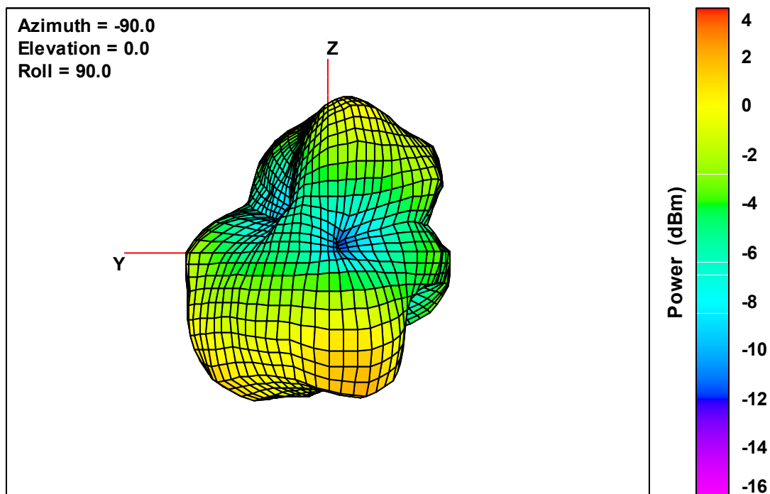
Ant. 4 Free-Space Total EIRP, Back Face View, 2475 MHz
