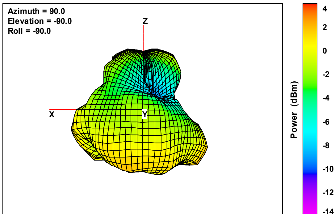
Ant. 4 Free-Space Total EIRP, Right Side View, 2442 MHz
