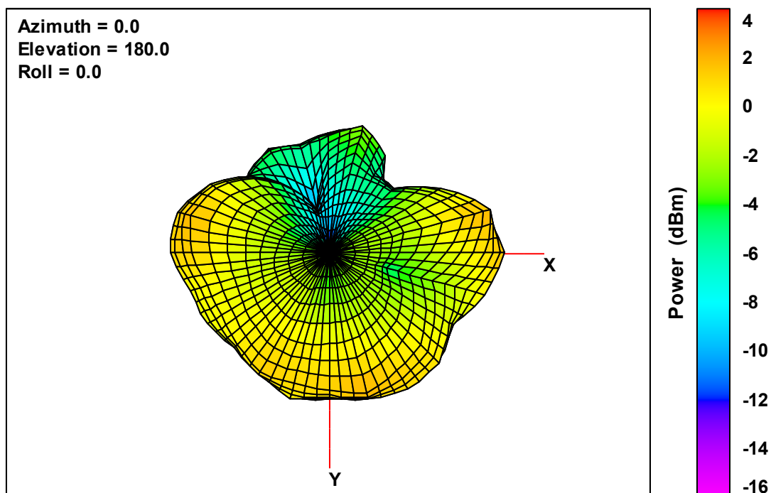
Ant. 4 Free-Space Total EIRP, Bottom View, 2480 MHz
