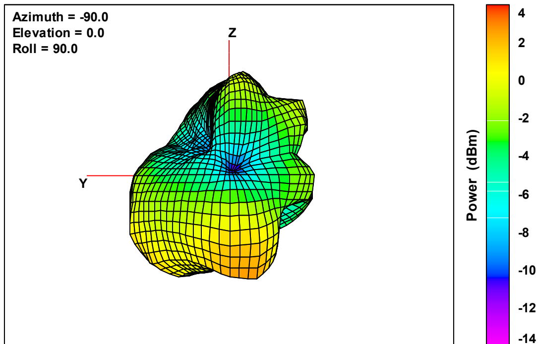
Ant. 4 Free-Space Total EIRP, Back Face View, 2405 MHz
