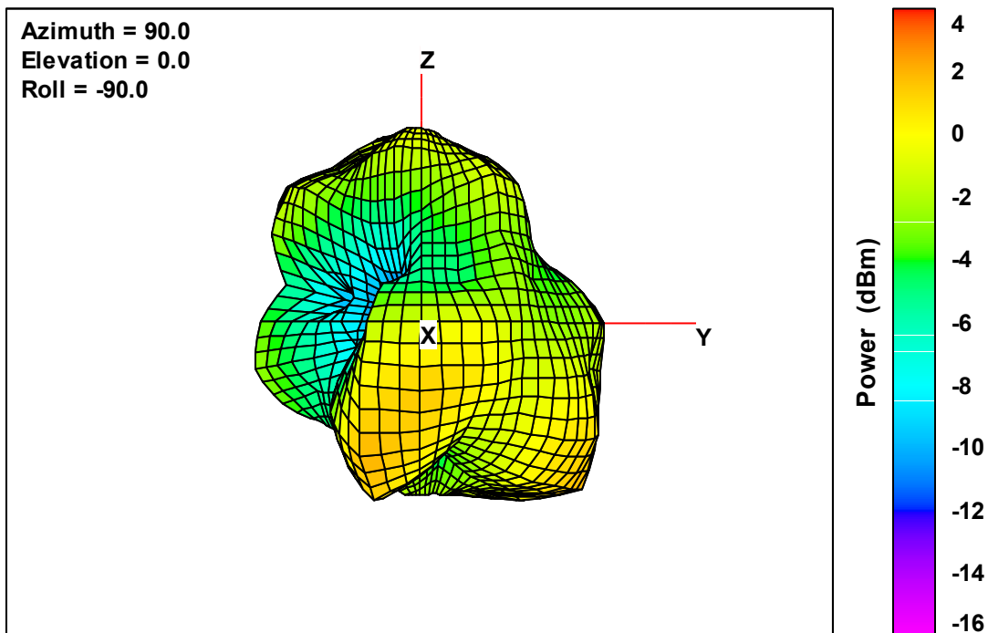
Ant. 4 Free-Space Total EIRP, Front Face View, 2475 MHz
