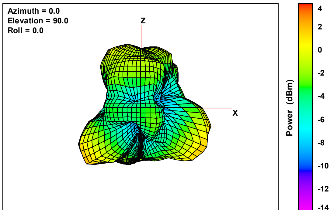
Ant. 4 Free-Space Total EIRP, Left Side View, 2445 MHz
