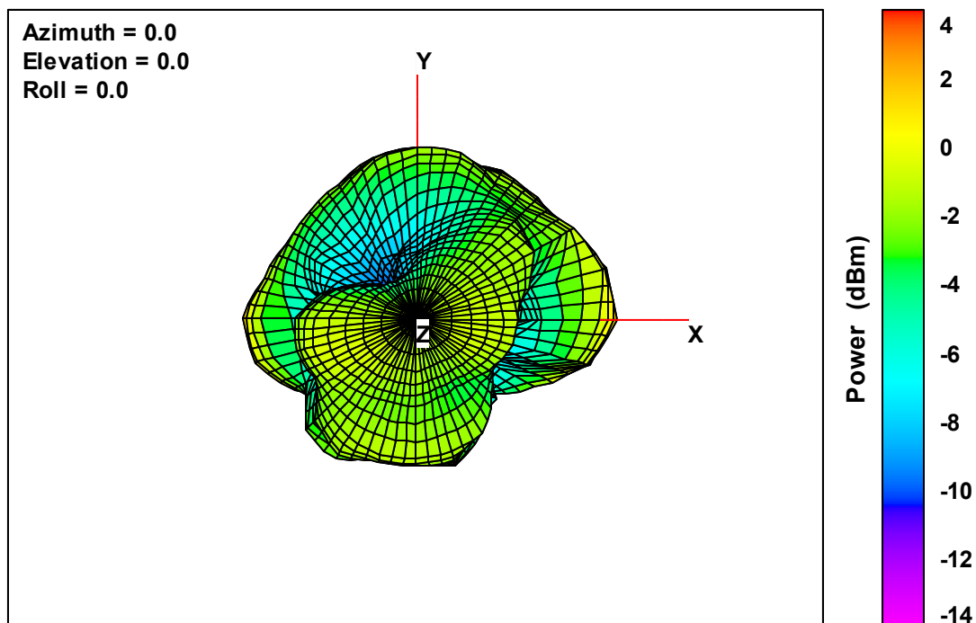
Ant. 4 Free-Space Total EIRP, Top View, 2442 MHz
