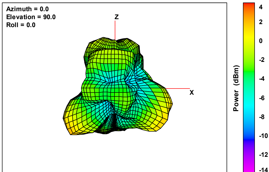
Ant. 4 Free-Space Total EIRP, Left Side View, 2442 MHz
