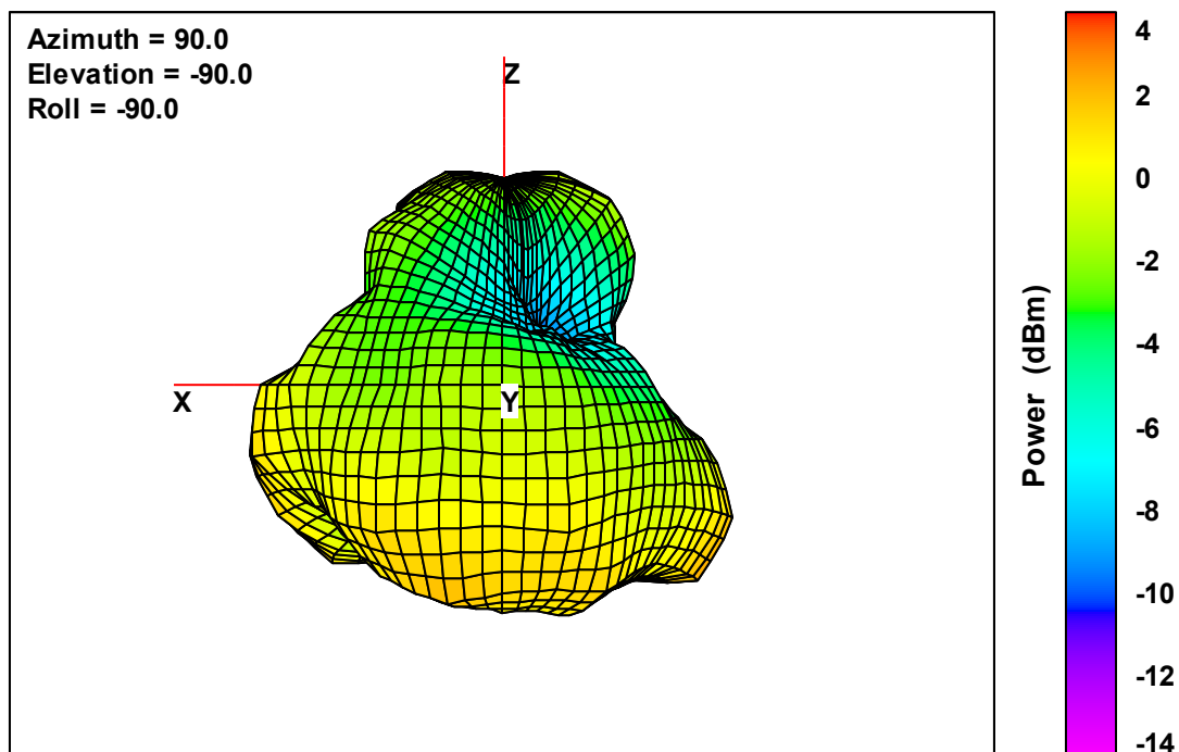
Ant. 4 Free-Space Total EIRP, Right Side View, 2405 MHz
