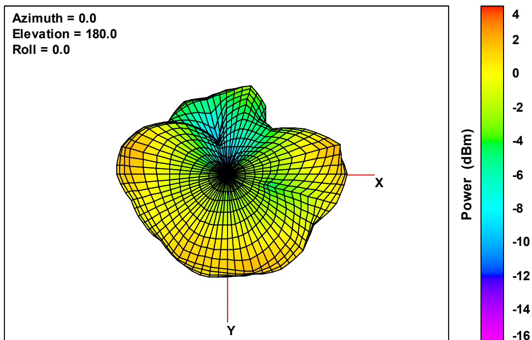
Ant. 4 Free-Space Total EIRP, Bottom View, 2475 MHz
