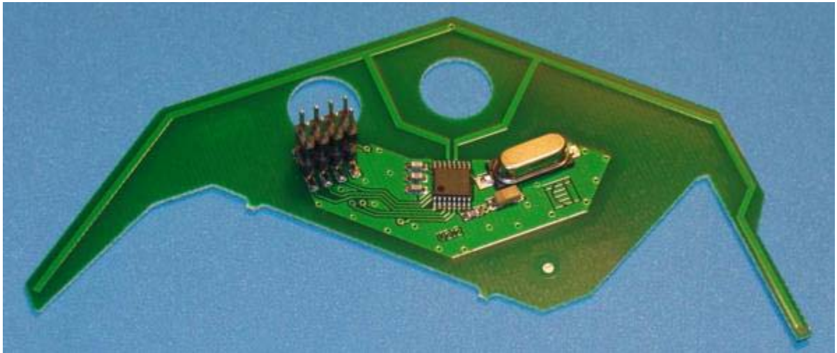
RF PCB
