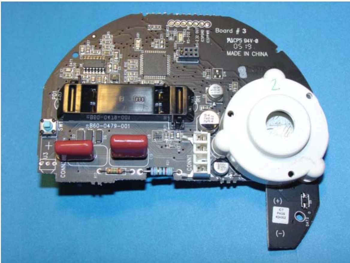
Main Board
