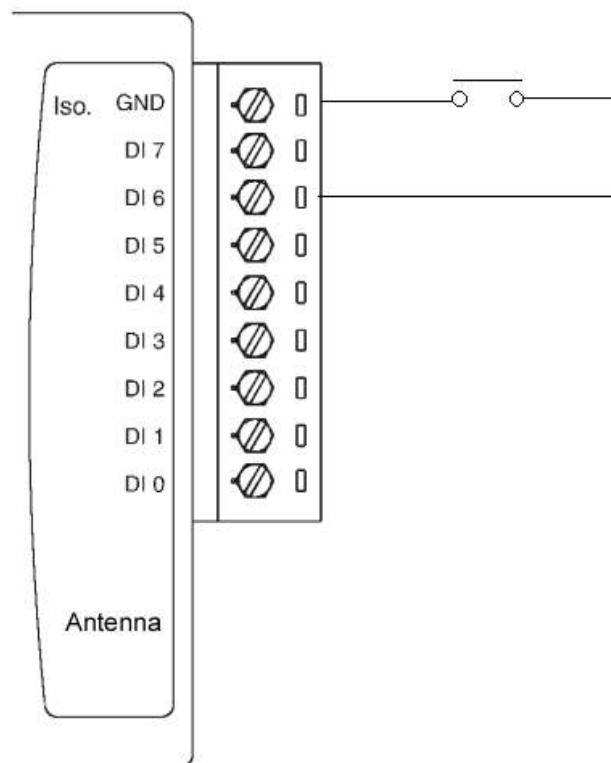
Figure 3: ADAM-6050W Digital Input (Dry Contact) Wiring
