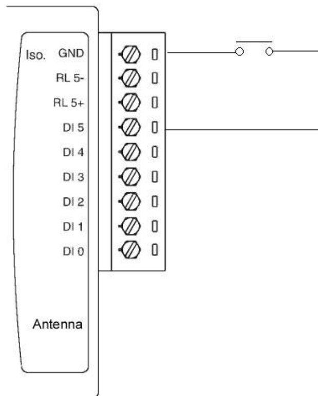
Figure 3: ADAM-6060W Digital Input (Dry Contact) Wiring
