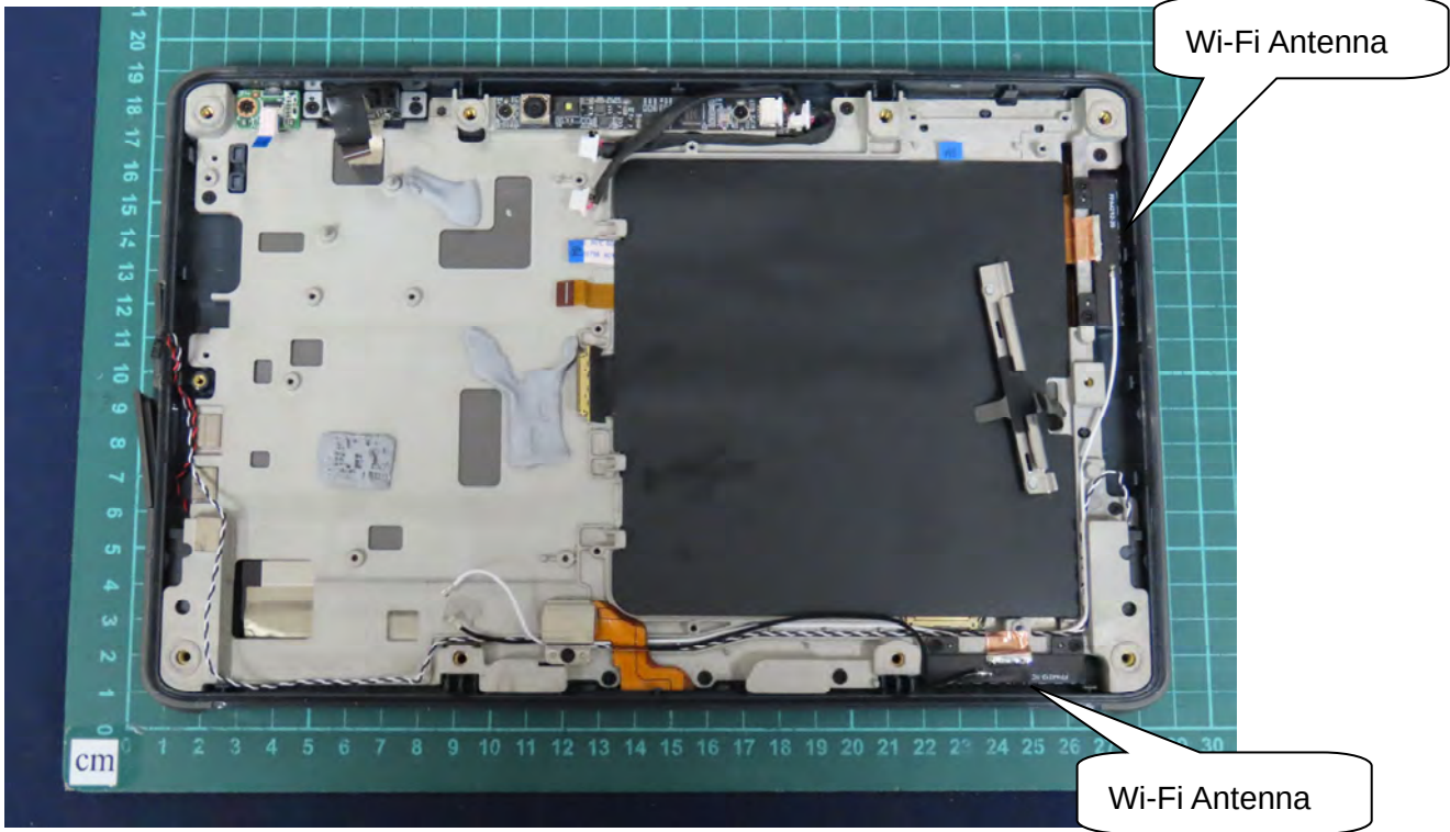
(28) EUT Photo
