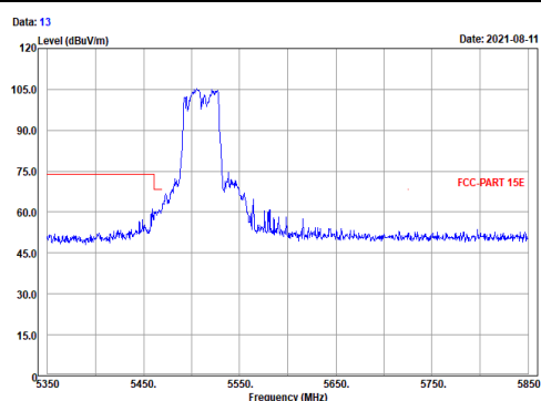
Vertical (Peak)
