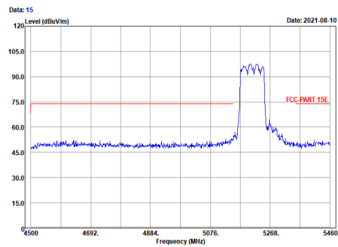
Vertical (Peak)
