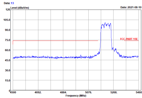
Vertical (Peak)
