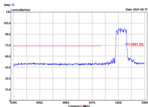
Vertical (Peak)
