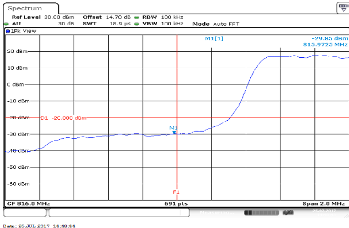
Figure 12-1: Band Edge emissions –CDMA / BC10 / CH 476
