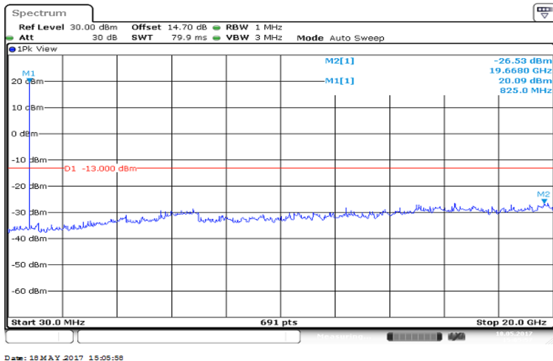
Figure 7-1: Out of Band emission at antenna terminals –CDMA / BC0 / CH 1013
