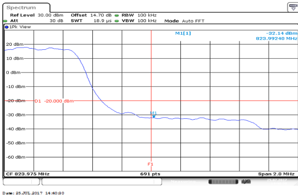
Figure 12-2: Band Edge emissions –CDMA / BC10 / CH 684
