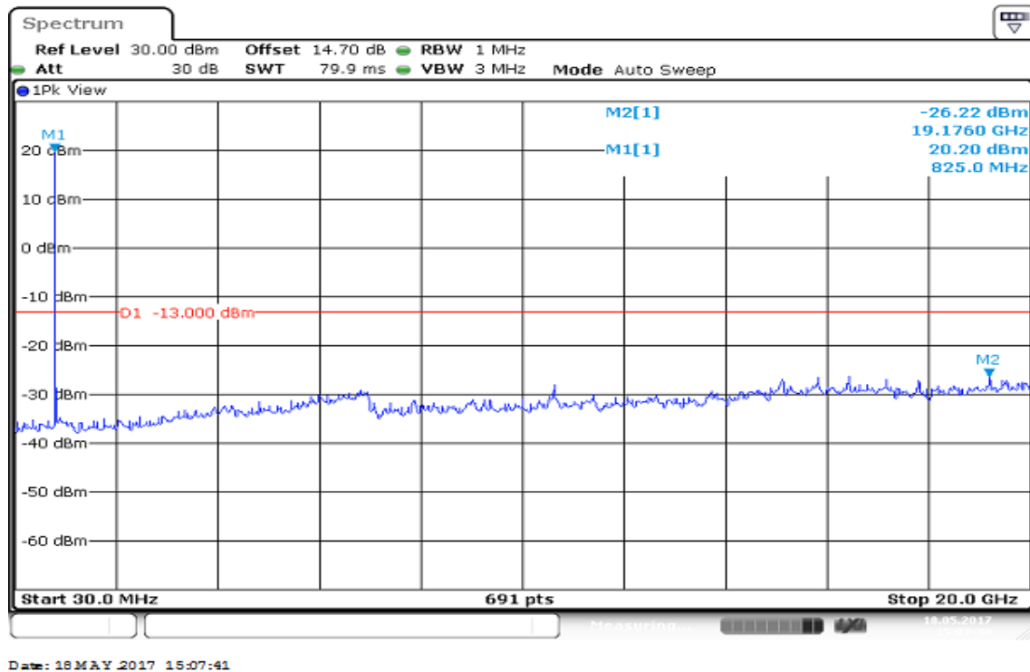
Figure 7-2: Out of Band emission at antenna terminals –CDMA / BC0 / CH 384
