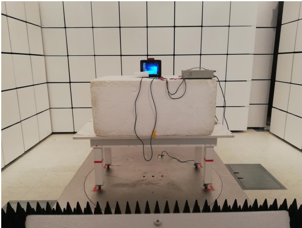
Radiated emissions test photos Above 1 GHz Antenna: Integrated Plane: Z
