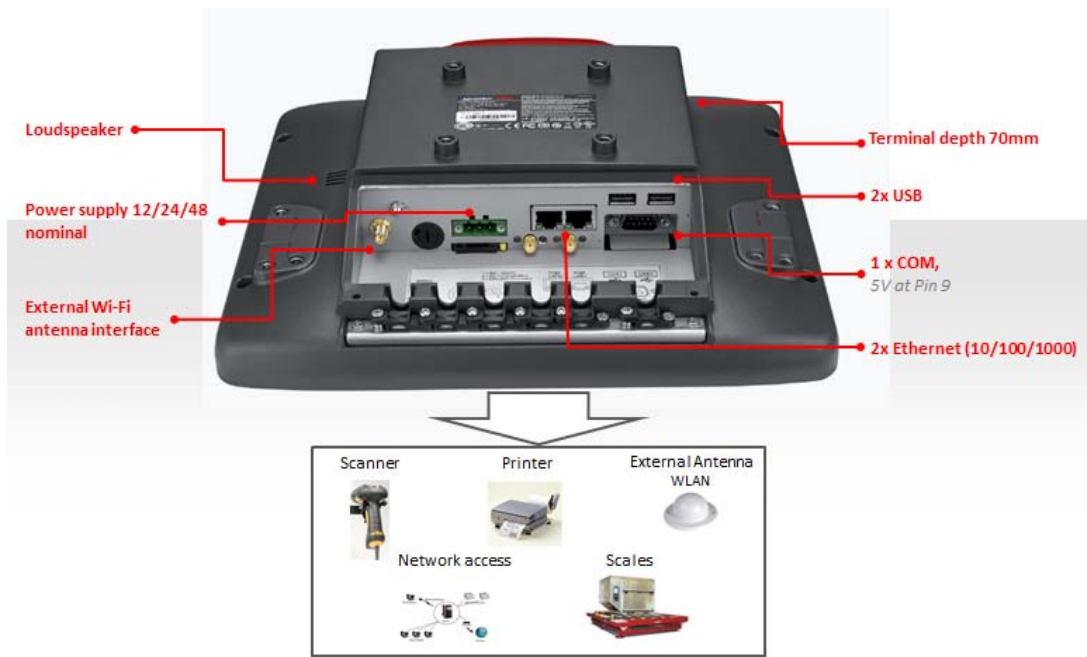
Fig. 8.4: External connectors of DLT-V6210
