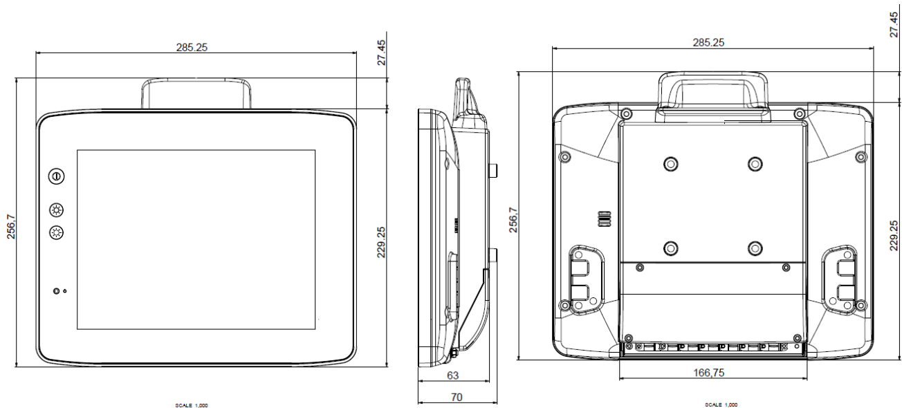
Fig. 11.2: Dimensions of DLT-V6210
