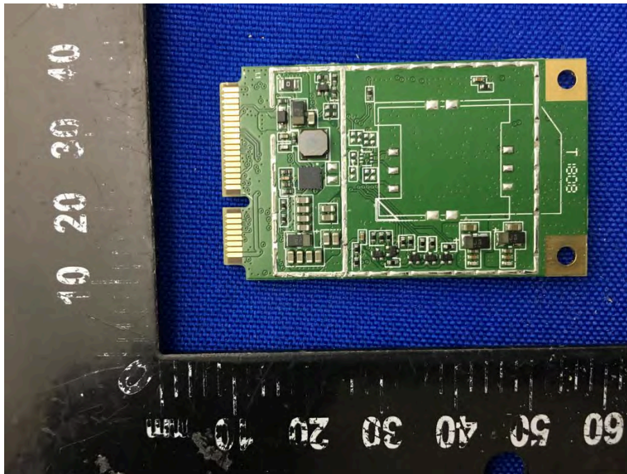
MAIN BOARD 6 REAR VIEW (WITHOUT SHIELDING)(DLT-V7212P+)
