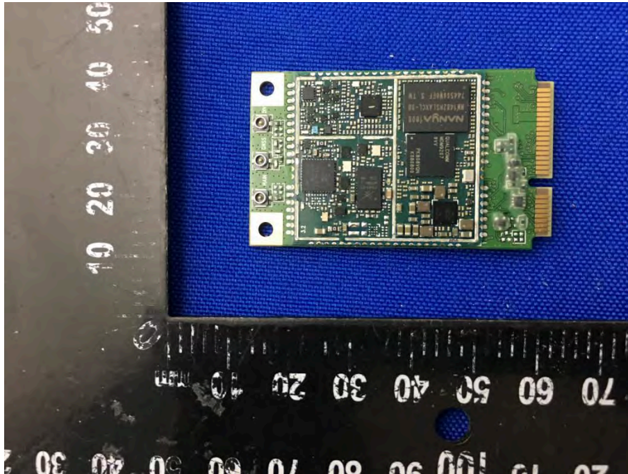
MAIN BOARD 5 TOP VIEW (WITHOUT SHIELDING) (DLT-V7210P)
