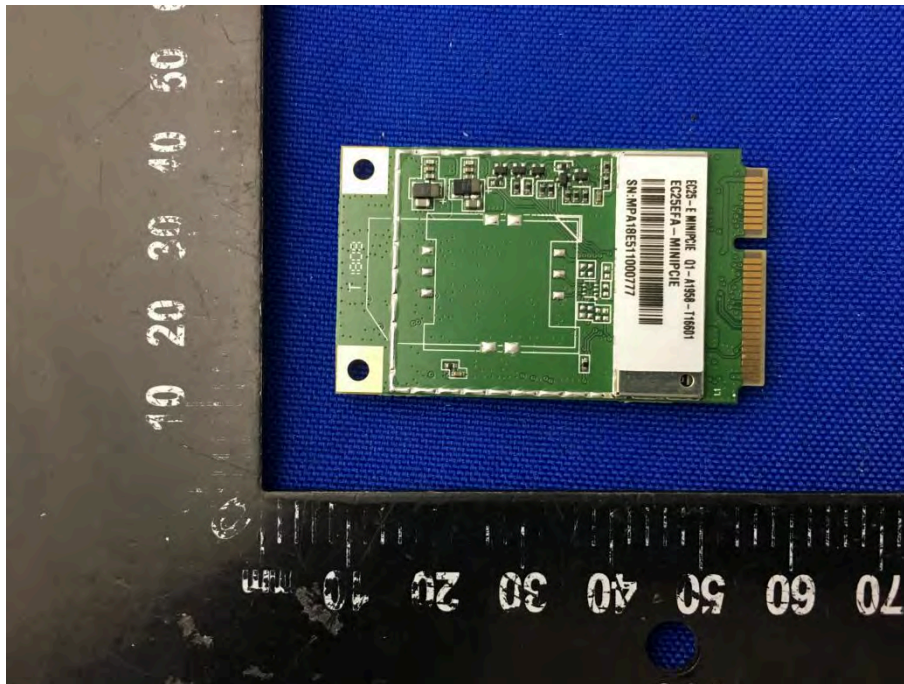
MAIN BOARD 6 REAR VIEW (WITH SHIELDING)(DLT-V7212P+)
