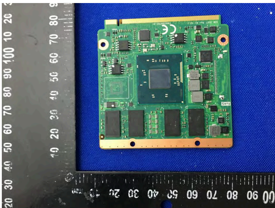
MAIN BOARD 8 TOP VIEW (DLT-V7212P+)
