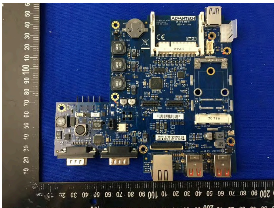
MAIN BOARD 7 TOP VIEW (DLT-V7212P+)
