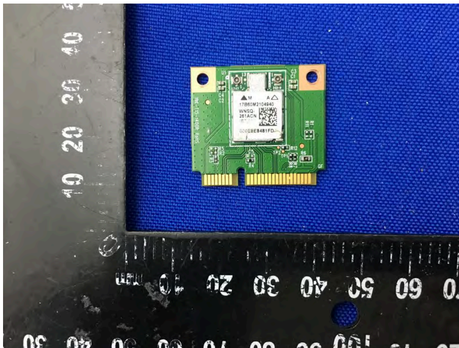
MAIN BOARD 8 TOP VIEW (WITH SHIELDING) (DLT-V7210P)
