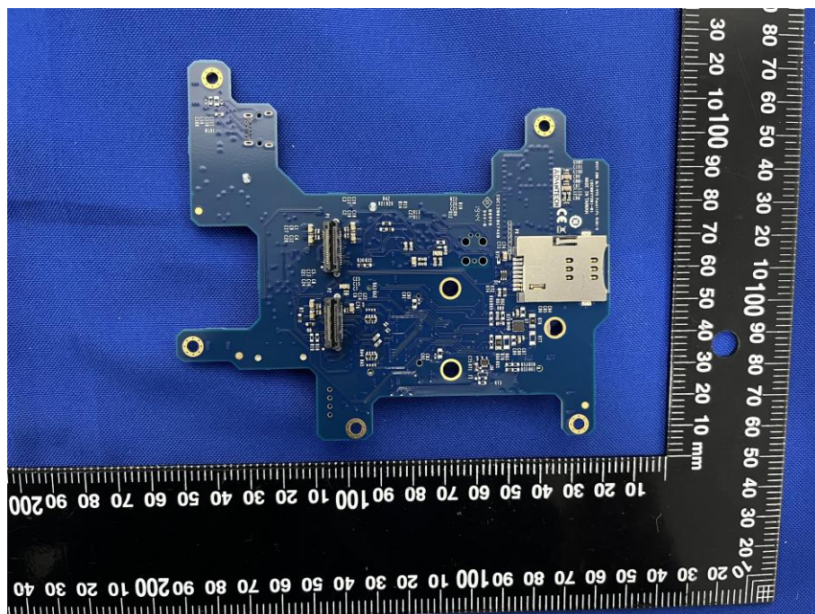
MAINBOARD-4 REAR VIEW
