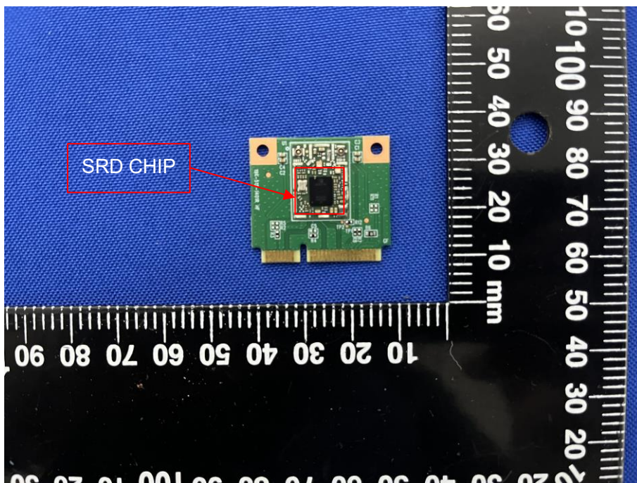
WLAN/BLEETOOTH MODULE TOP VIEW-REMOVE SHIELDING
