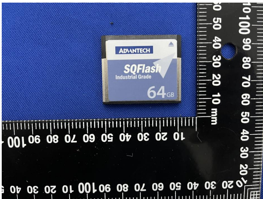
SQFlash TOP VIEW
