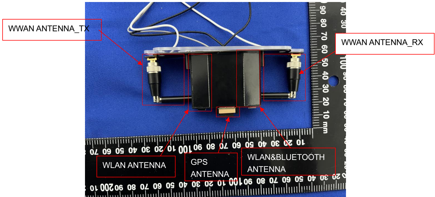
EUT ANTENNA VIEW-1
