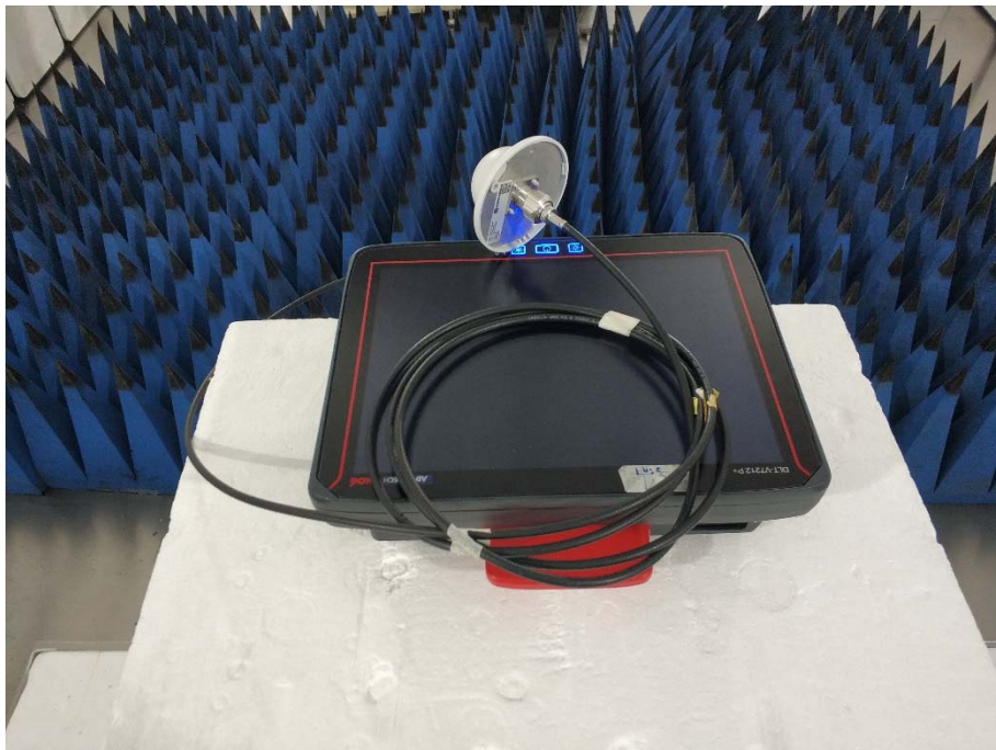
Close-up- BT/BLE(External Antenna)
