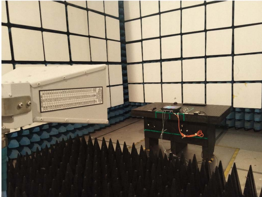
Above 1GHz-2/3/4G
