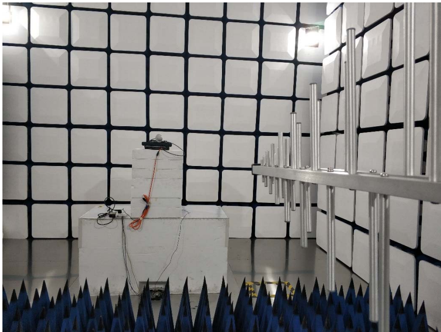
30 MHz-1 GHz- BT/BLE(External Antenna)
