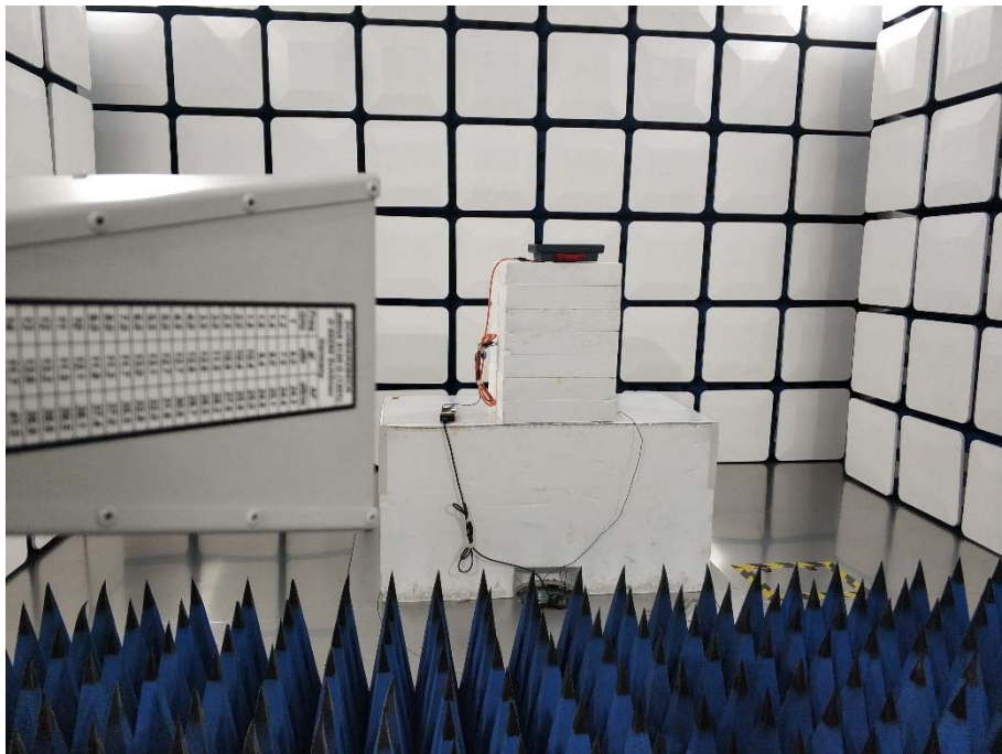
Above 1GHz- BT/BLE(Internal Antenna)
