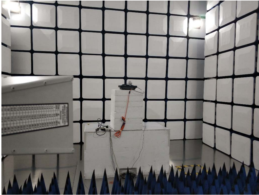
Above 1GHz- BT/BLE(External Antenna)
