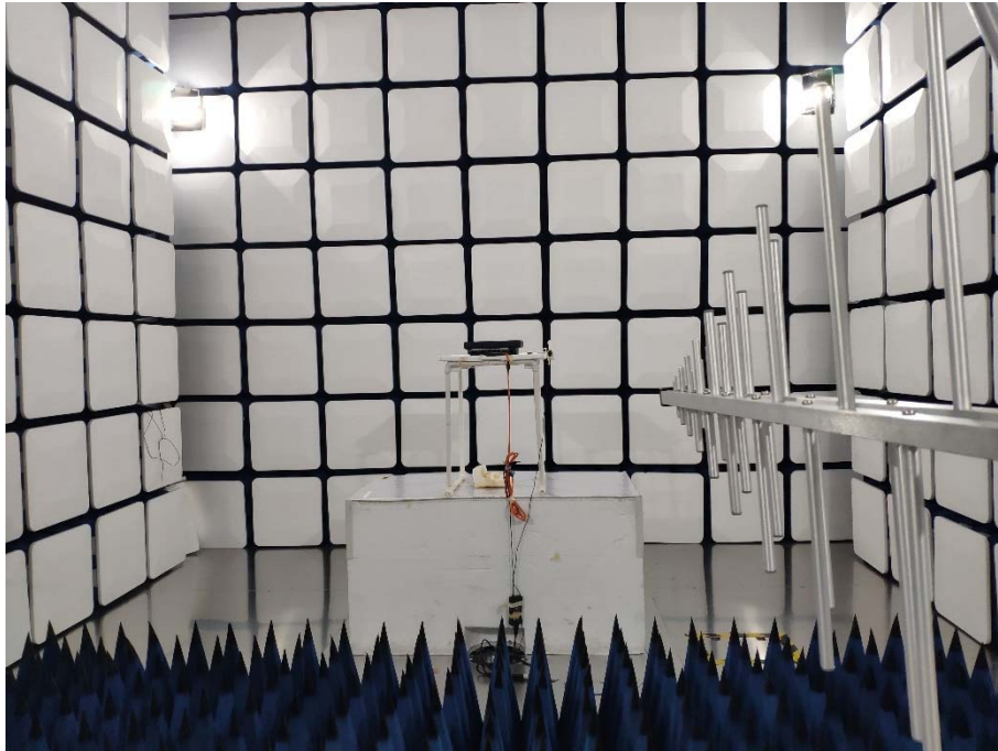
30 MHz-1 GHz-WIFI
