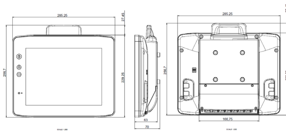
Fig. 11.2: Dimensions of DLT-V6210
