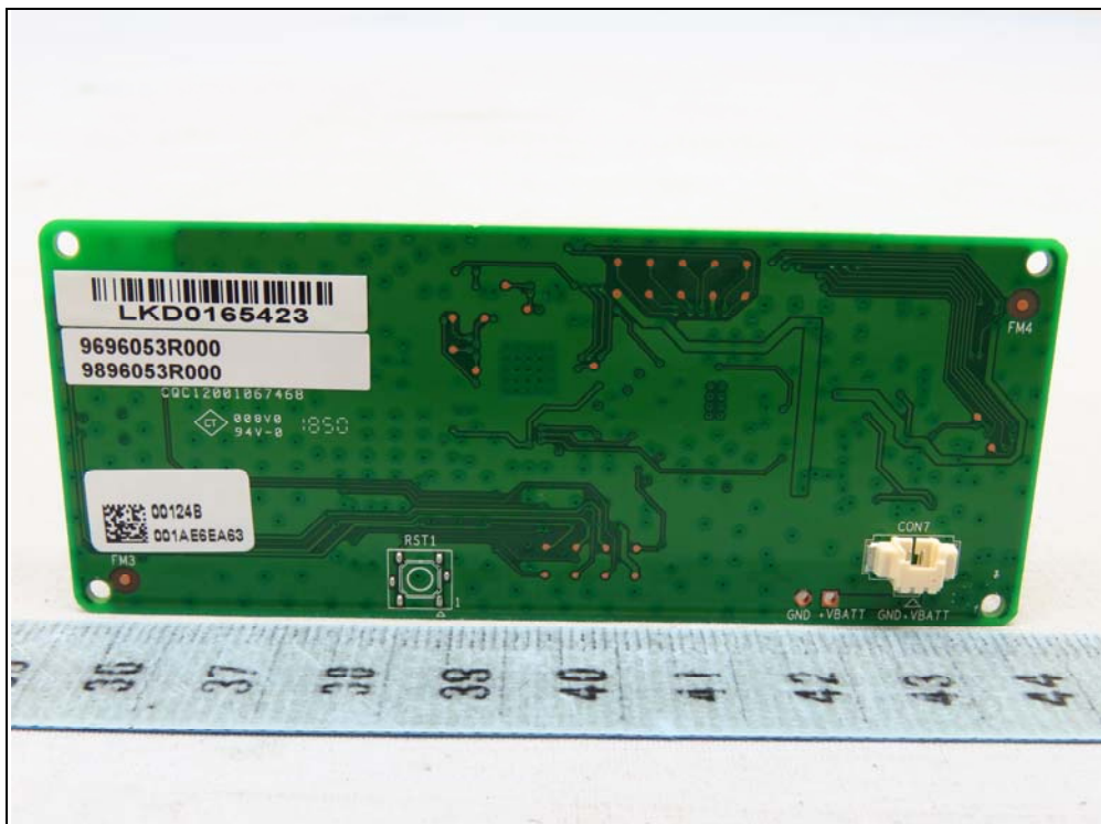
End-Product (Model: EPD-053R2)
