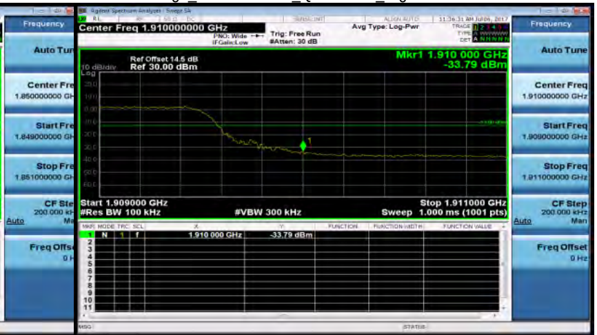
Band Edge Band2 10MHz QPSK 50 0 HighCH19150-1905
