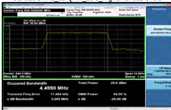
Band26 5MHz_16-QAM_25_0_HighCH27015-846.5
