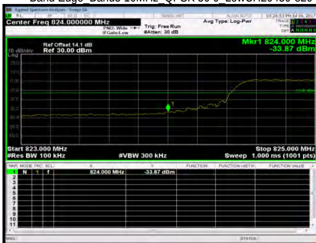
Band Edge Band5 10MHz QPSK 50 0 LowCH20450-829
