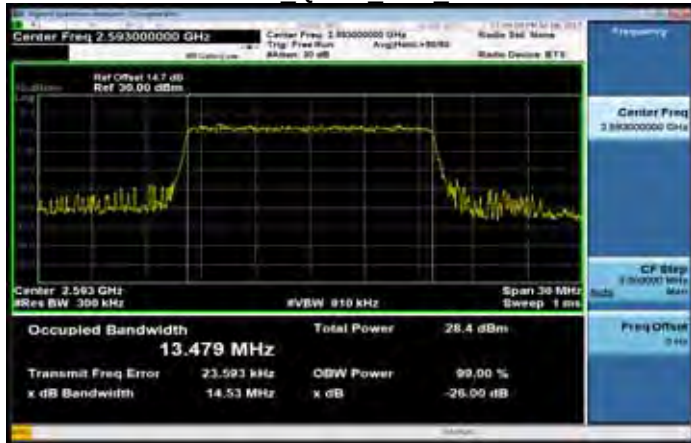
Band41 15MHz QPSK 75 0 MidCH40620
