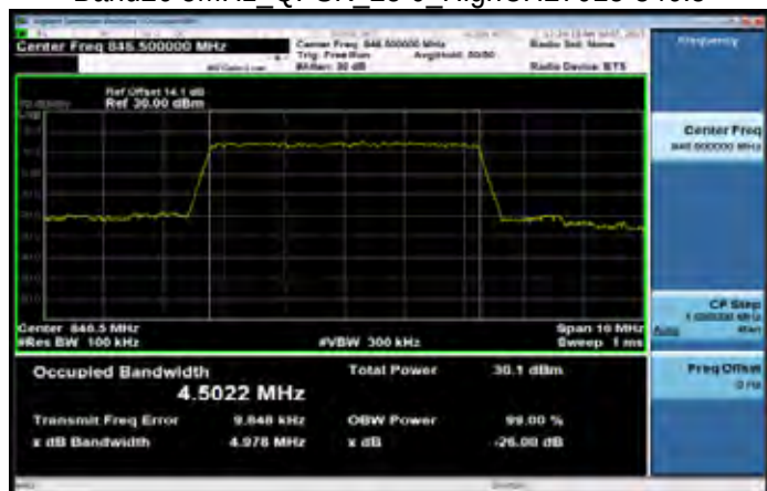
Band26 5MHz_QPSK_25_0_HighCH27015-846.5
