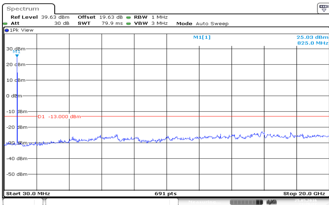
Figure 21-2: Out of Band emission at antenna terminals – HSDPA CH Mid
