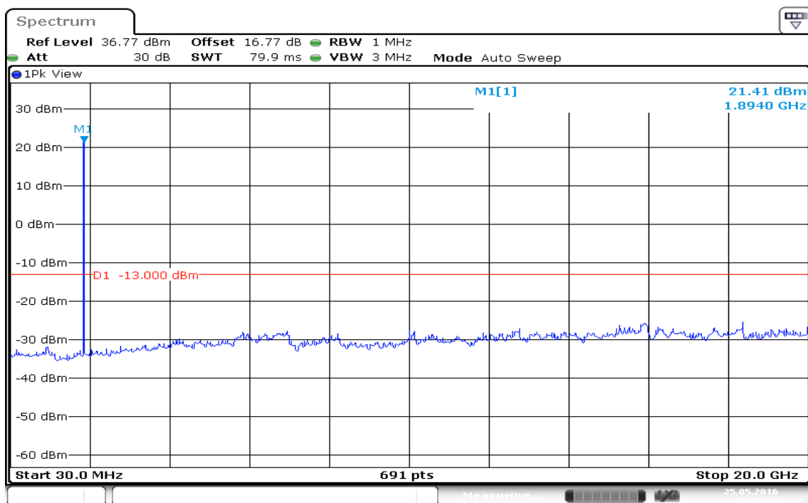
Figure 16-2: Out of Band emission at antenna terminals – WCDMA CH Mid
