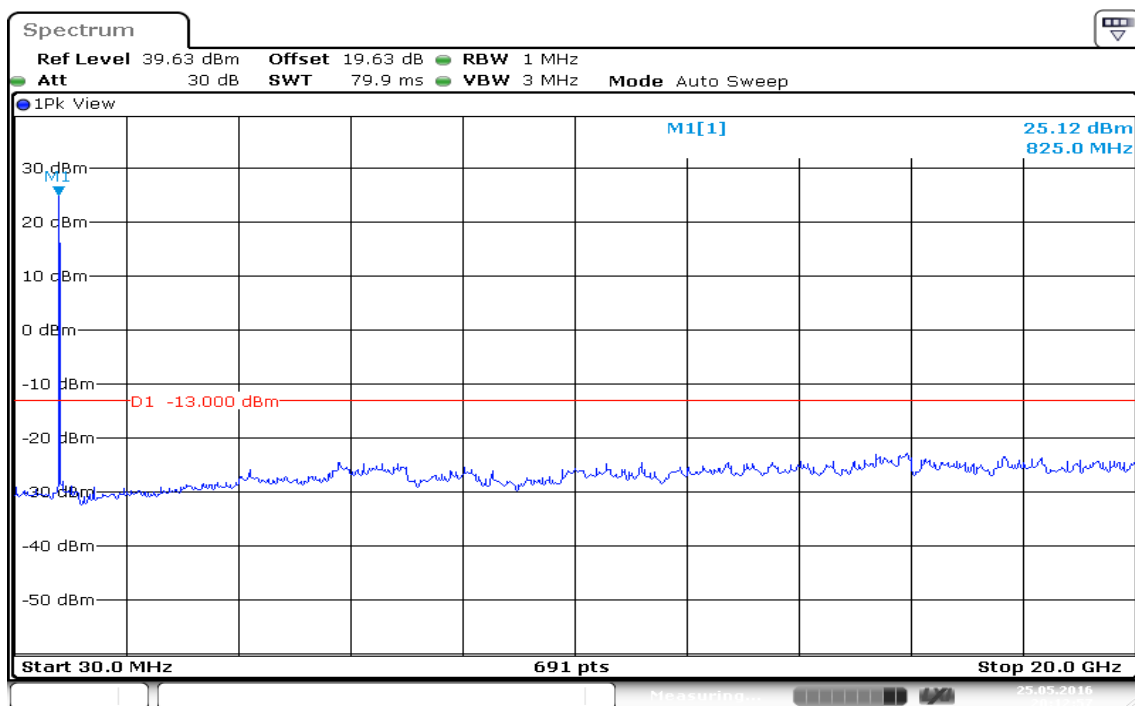
Figure 17-2: Out of Band emission at antenna terminals – WCDMA CH Mid
