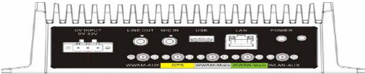
Figure 2.2 Rear view of TREK-572
