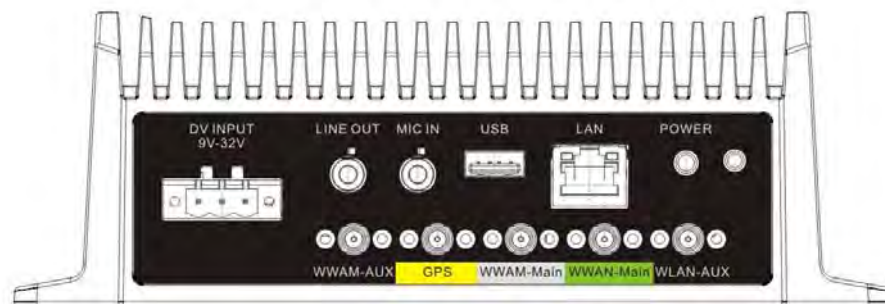
Figure 2.2 Rear view of TREK-572
