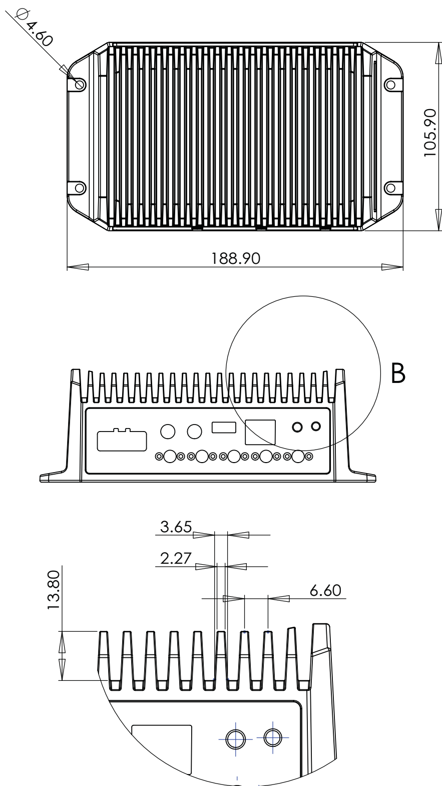
Figure 1.1 TREK-572 dimensions
