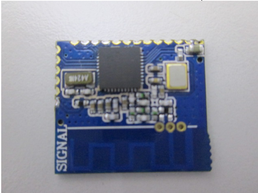
Figure 9 Internal View (BLE Module, Front View)
