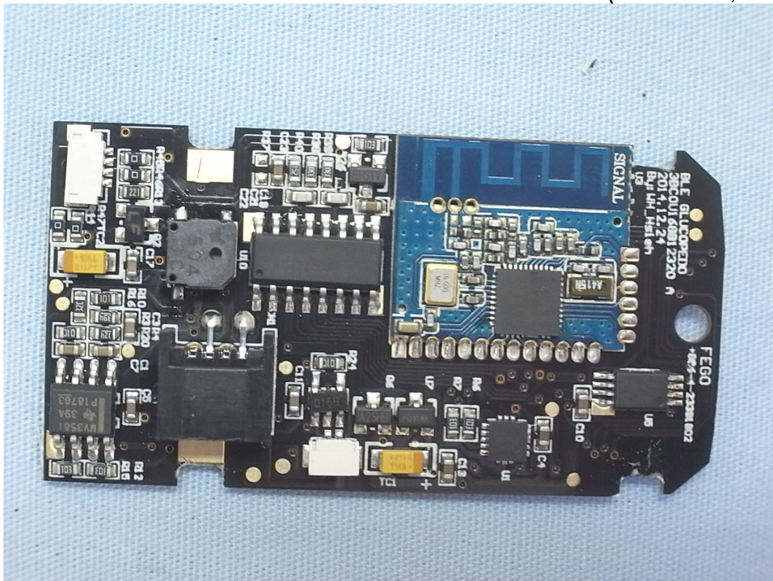
Figure 8 Internal View (Main Board, Front View)
