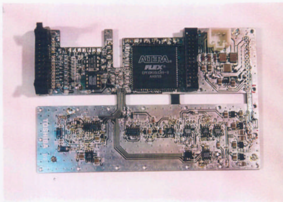
RF board (B2) top view
