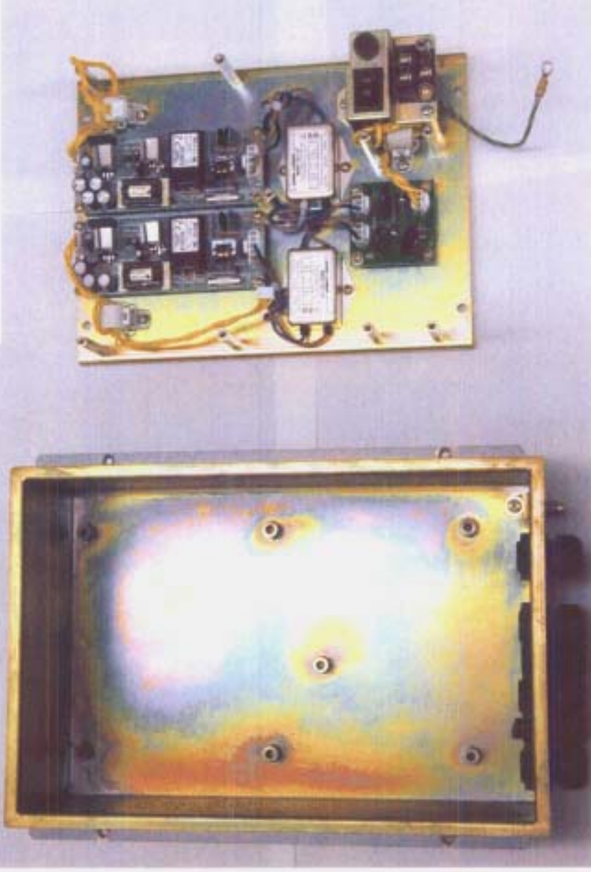
Converter (Inner unit removed)
