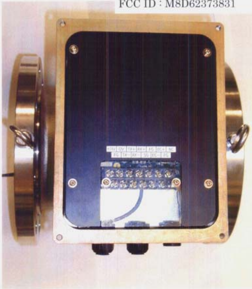
Signal processing unit (Cover removed)
