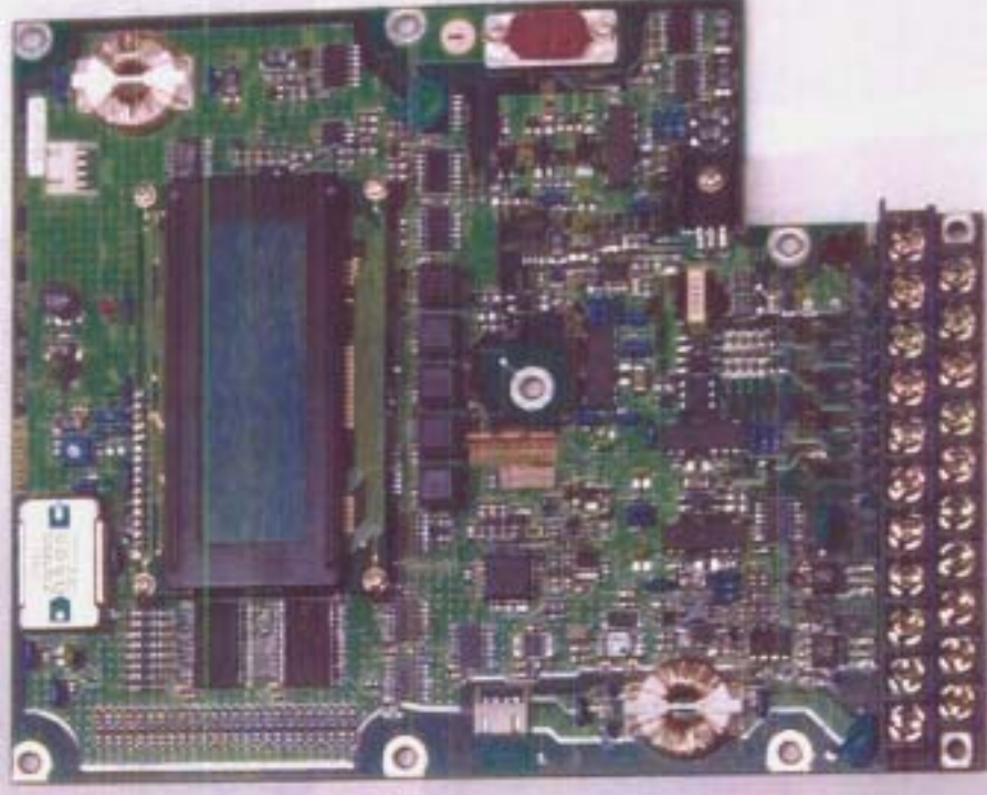
Main(cpu) board of Converter(top view)
