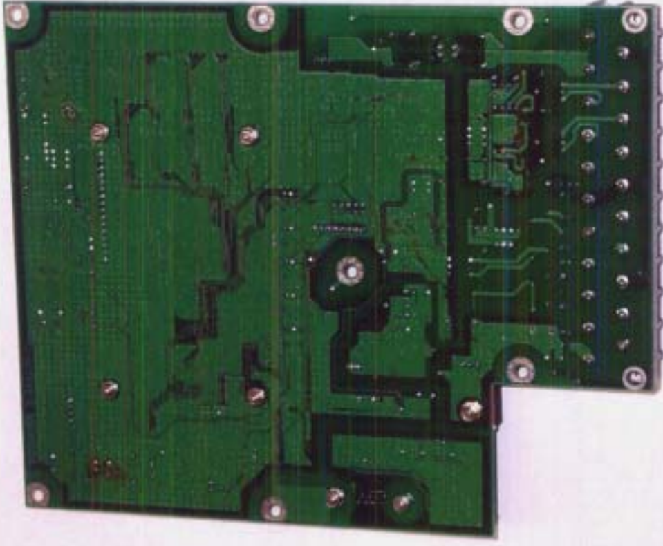
Main(cpu) board of Converter(bottom view)
