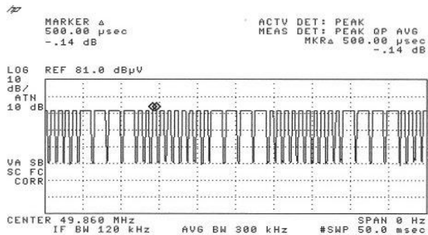
Figure C [Short Pulse]
