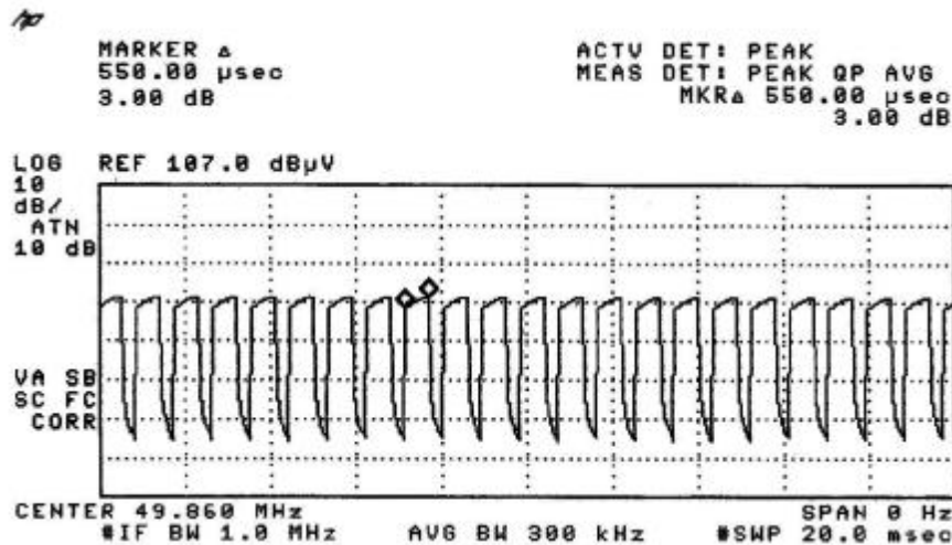
Figure B [Long or Short Pulse]
