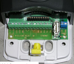
MA120 I-O connections
