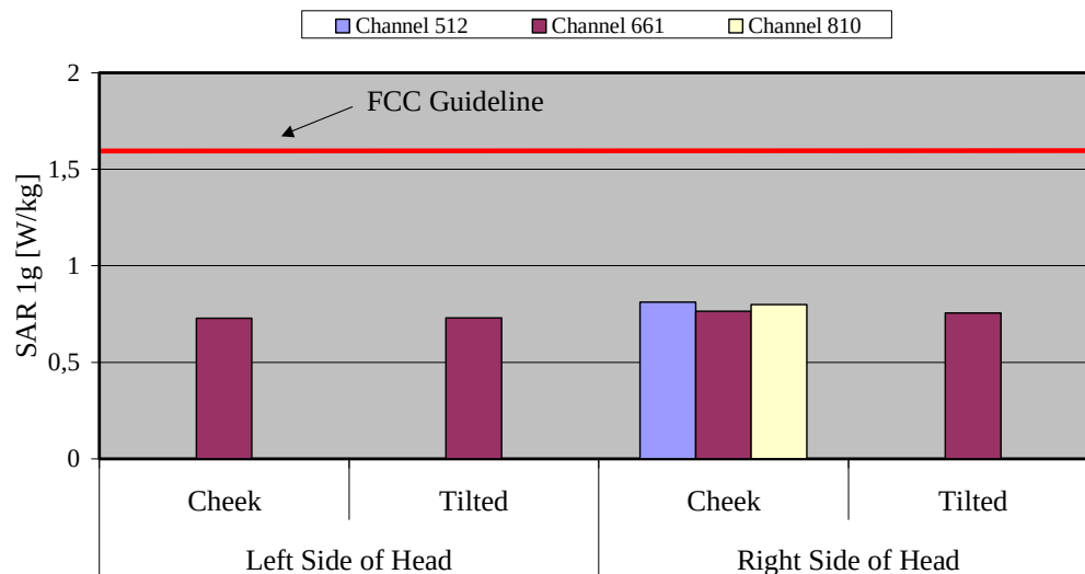
Fig. 7: The measured head phantom SAR values for the Sagem P52-0 for PCS 1900 in comparison to the FCC exposure limit.
