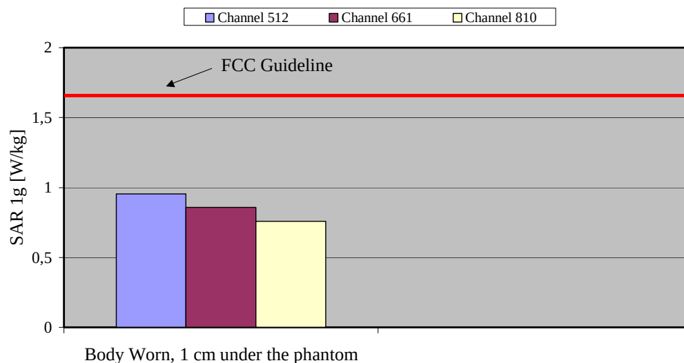
Fig. 8: The measured SAR values in body-worn configuration for the Sagem P52-0 for PCS 1900 in comparison to the FCC exposure limit.
