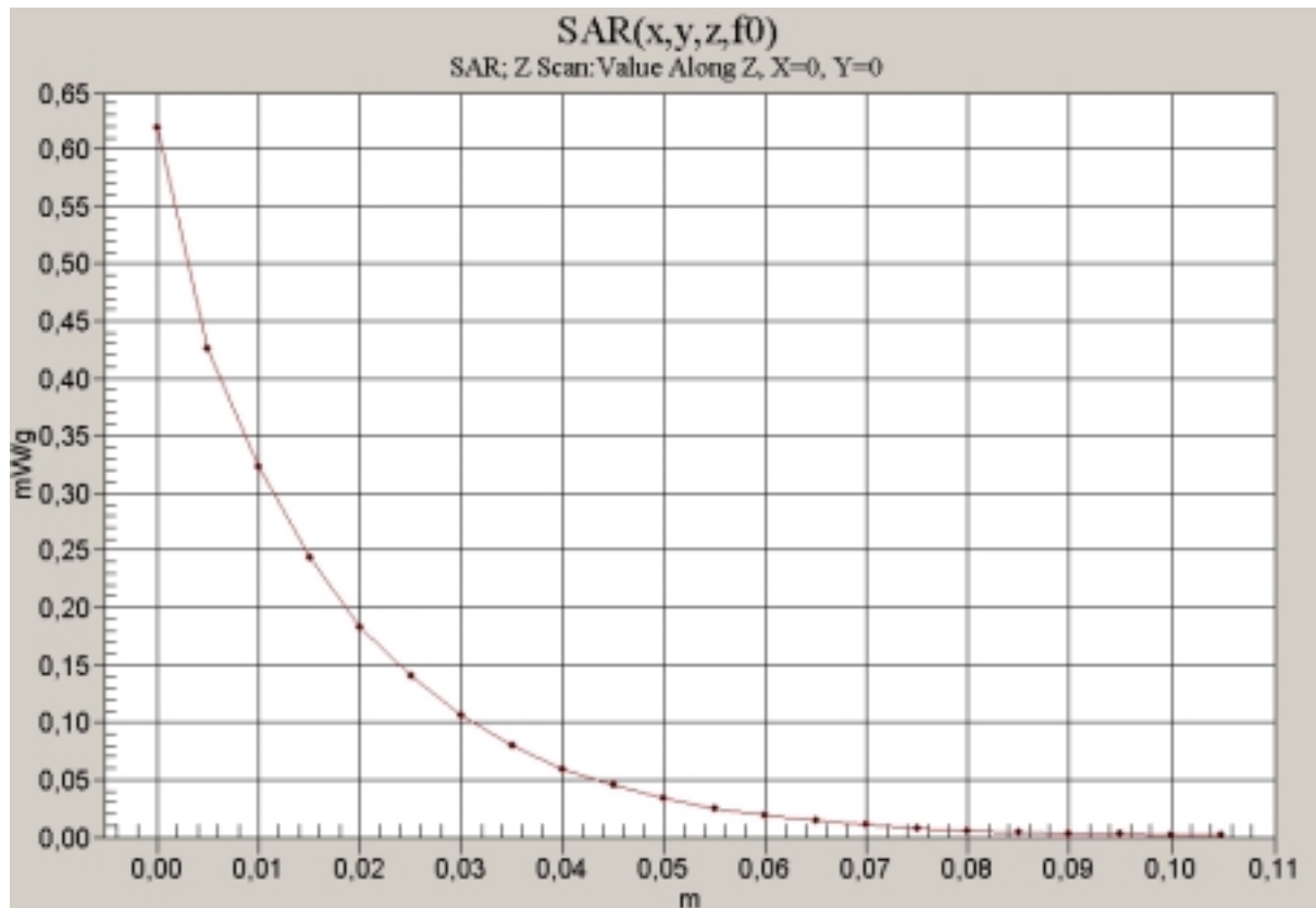
850 MHz head
