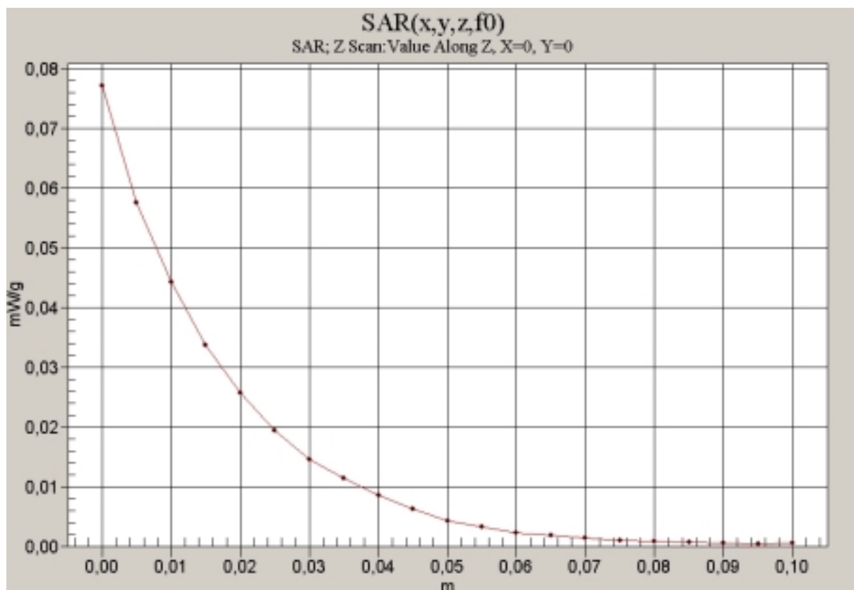
850 MHz Body
